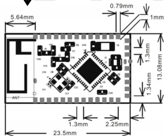
Figure 6. Mechanical Dimension of RB8762-35A1
