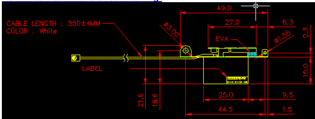
Aux Antenna Dimensioned Drawing:
