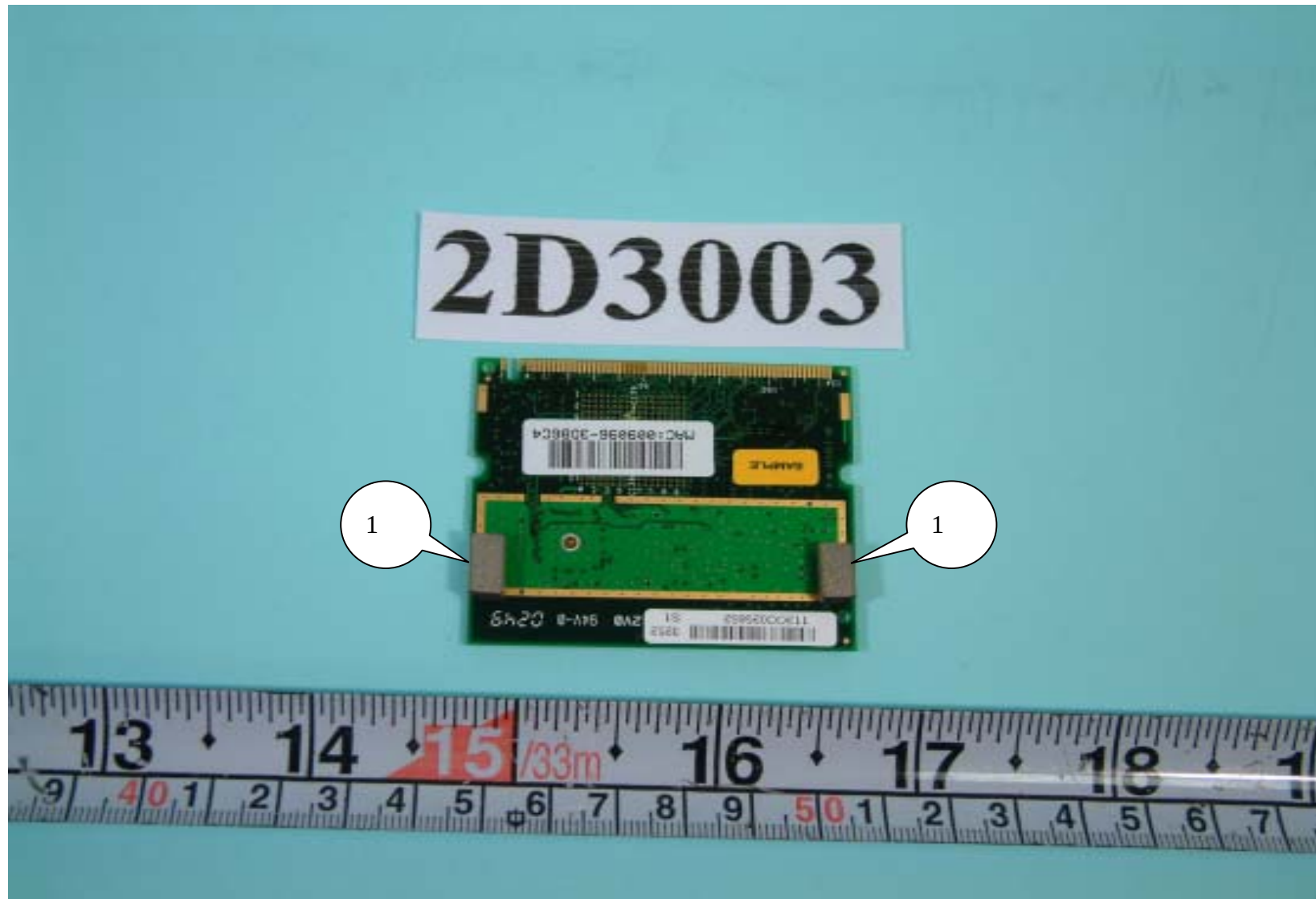
Rear side of daughter board
