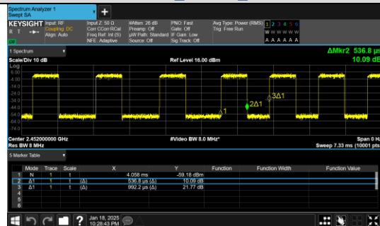
IEEE 802.11ax 40MHz Channel 9
