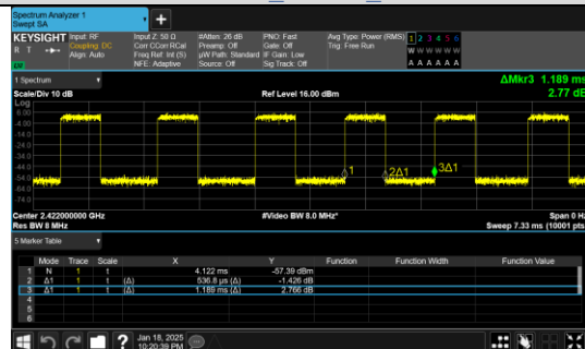
IEEE 802.11ax_40MHz_Channel 3
