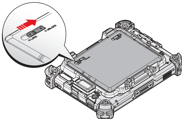
Figure 66. Unlock the External Battery
