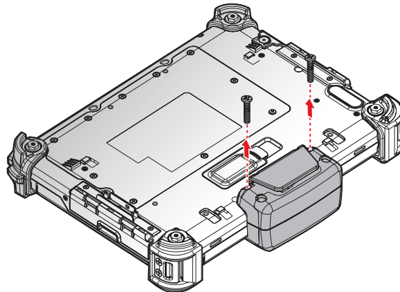
Figure 75. Removing the Screws
