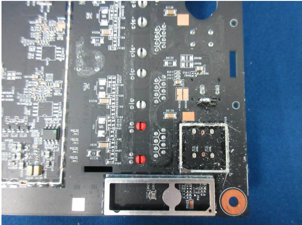
(55) EUT Photo
