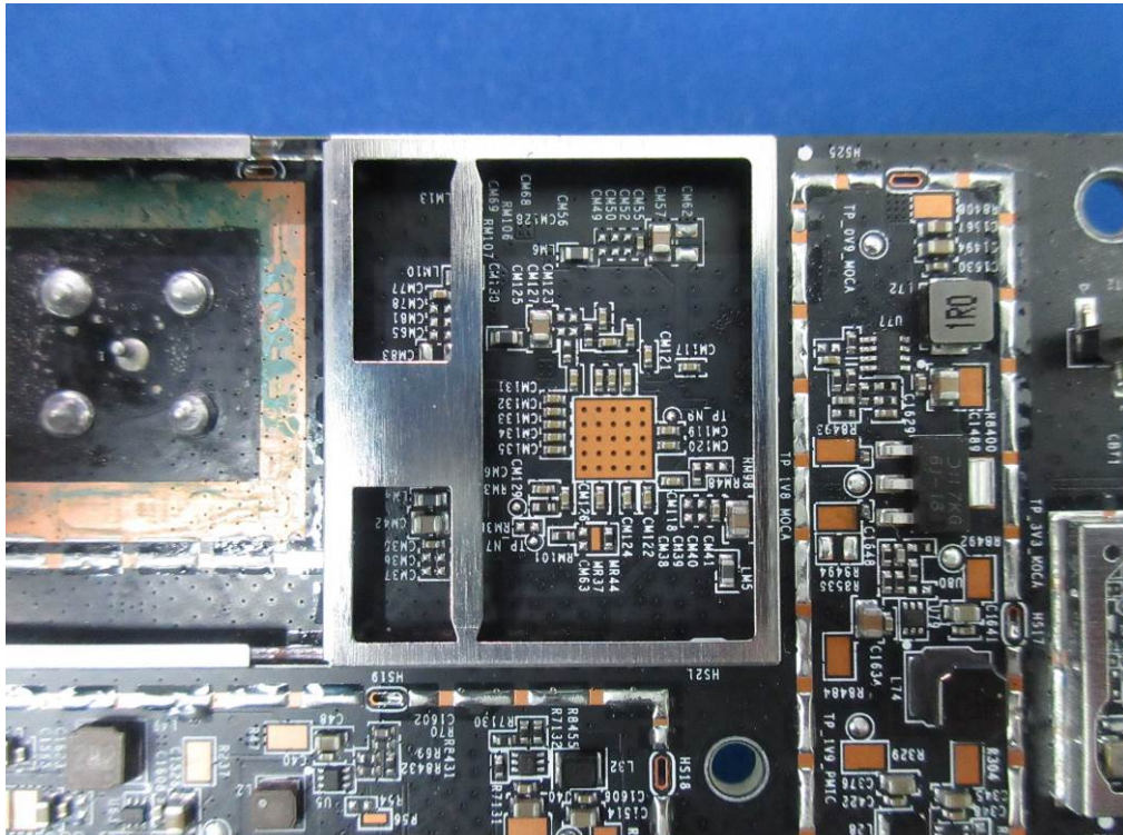
(73) EUT Photo
