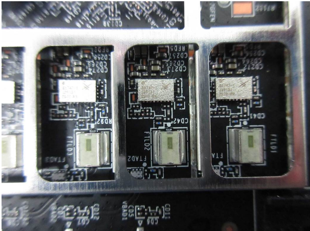
(89) EUT Photo
