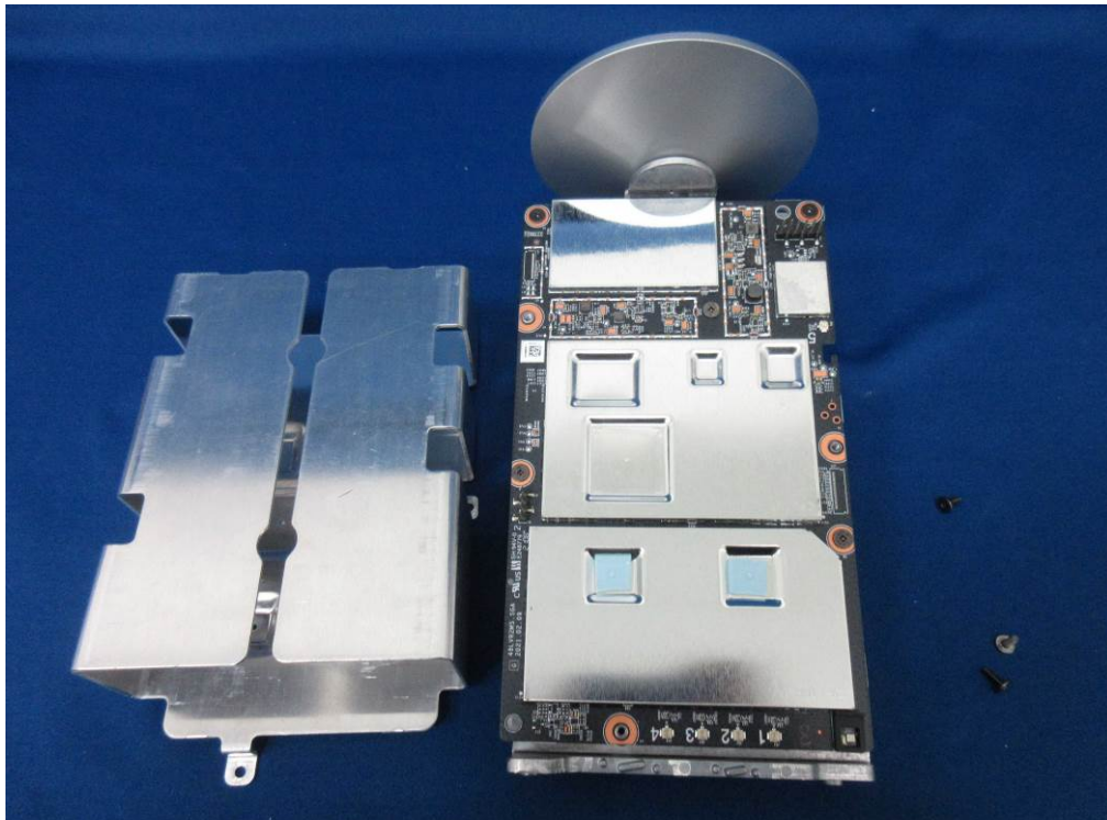
(55) EUT Photo
