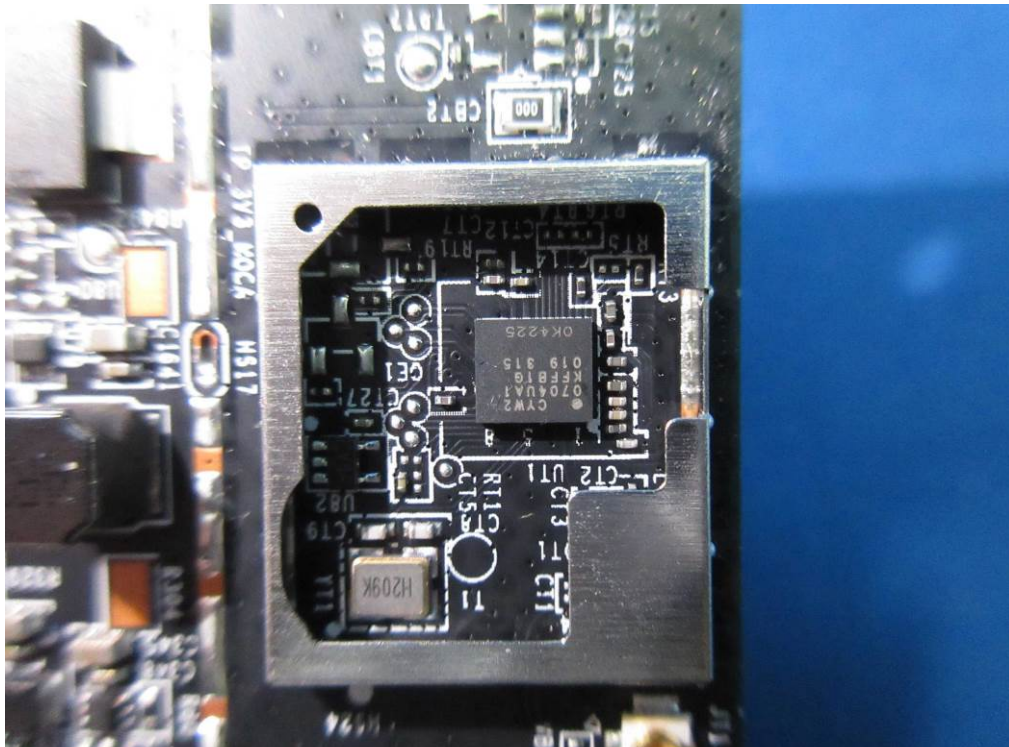
(73) EUT Photo
