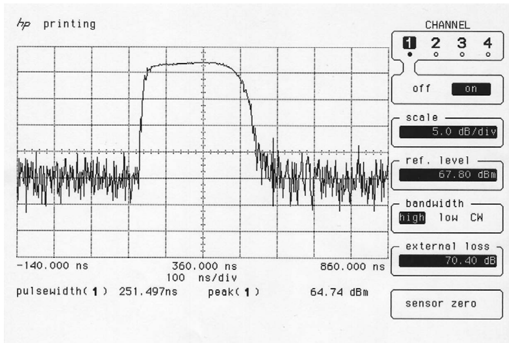
Graph PW/555/1002/04
