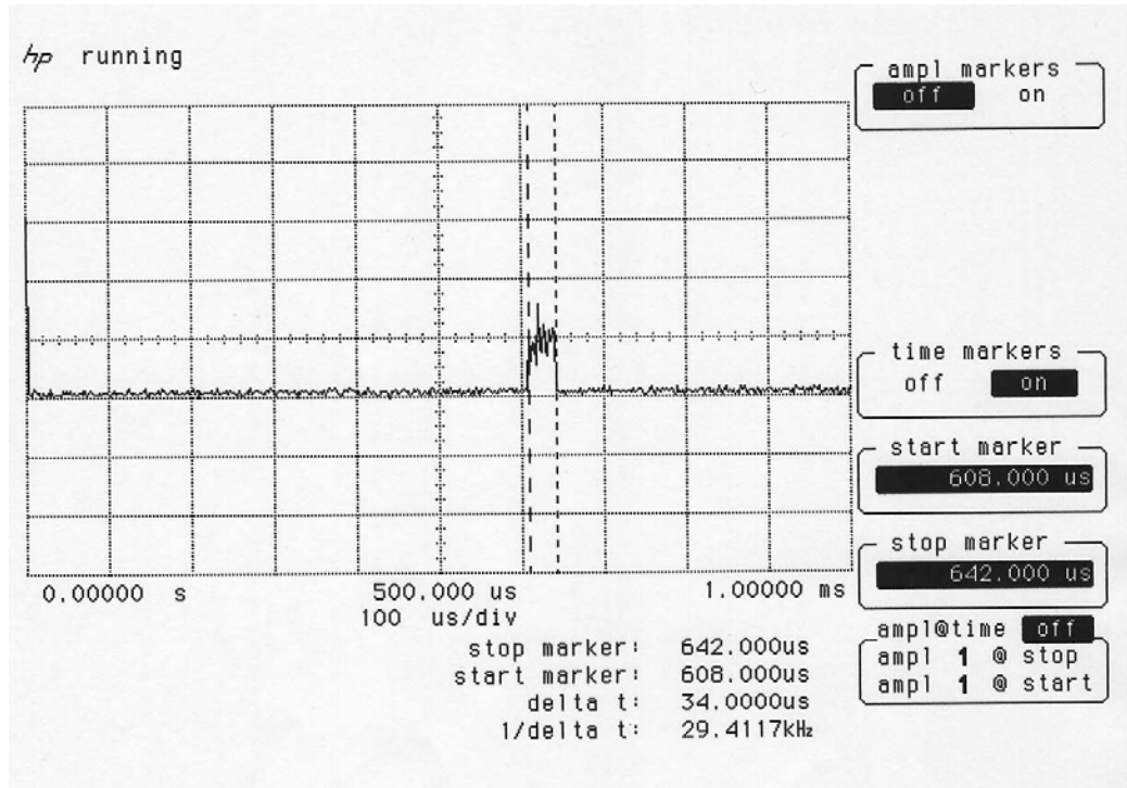
Graph PRF/555/1002/05
