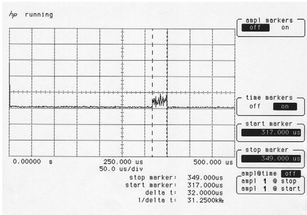
Graph PRF/555/1002/09
