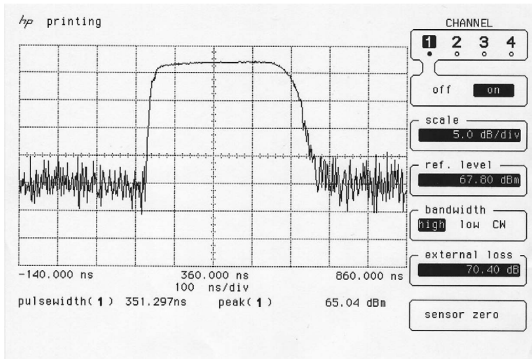
Graph PW/555/1002/05
