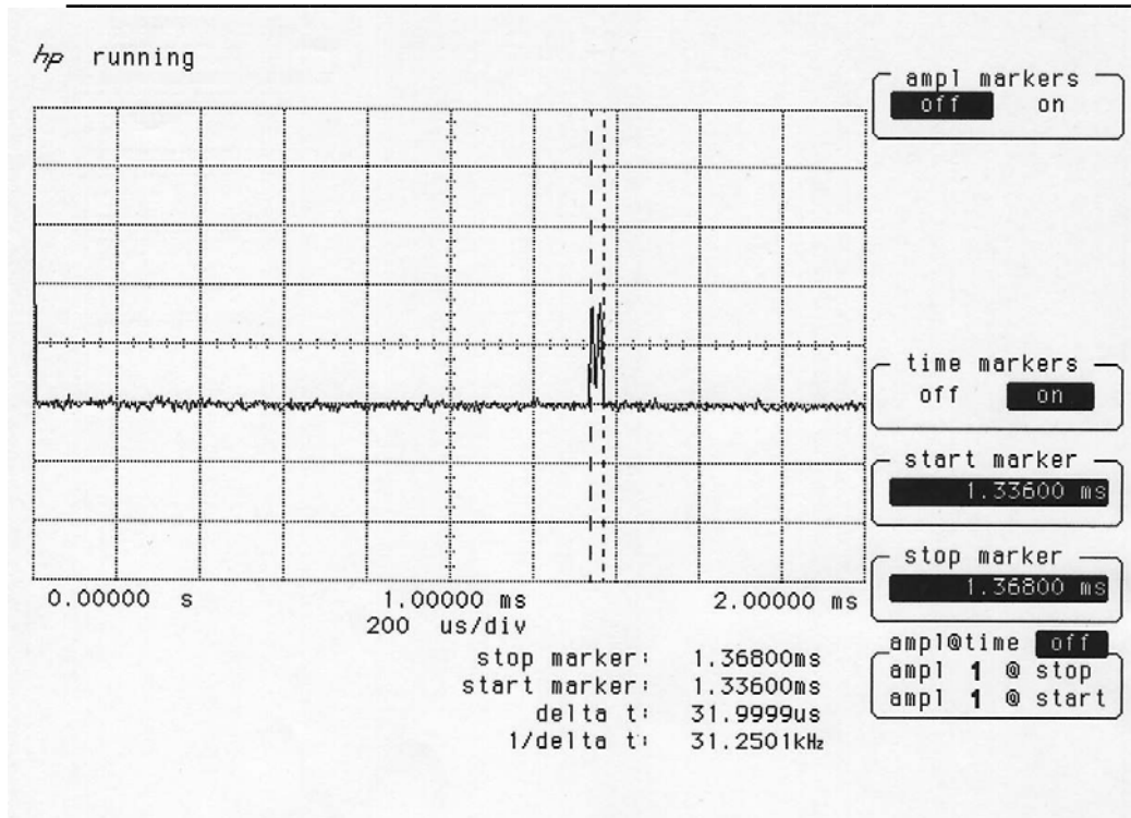
Graph PRF/555/1002/01
