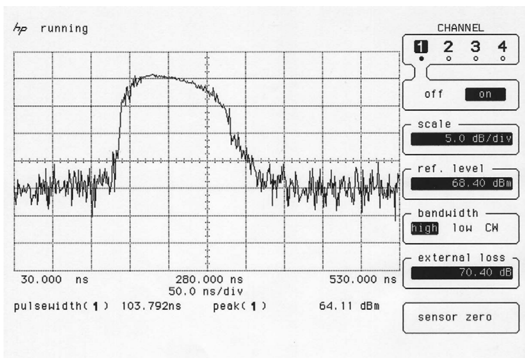
Graph PW/555/1002/02
