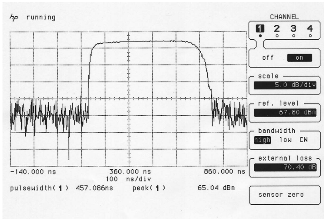
Graph PW/555/1002/06
