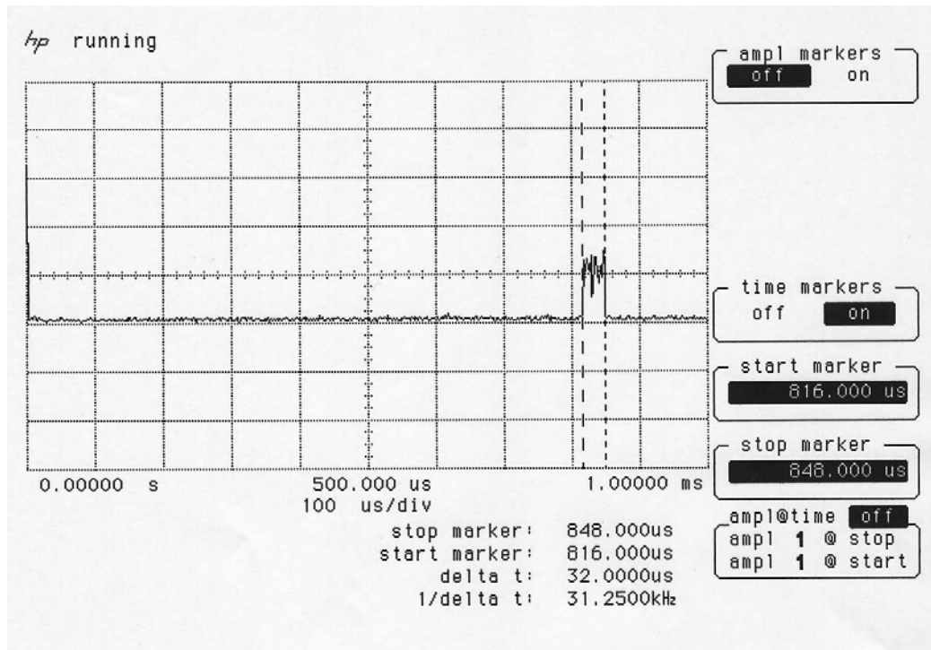
Graph PRF/555/1002/03
