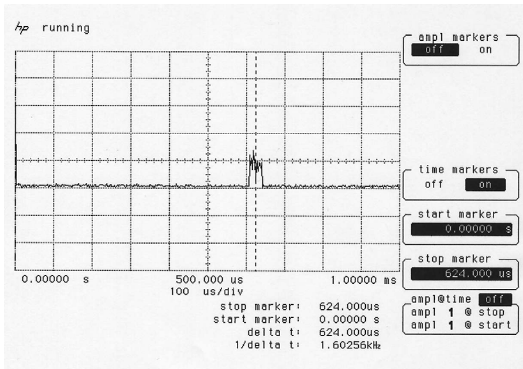
Graph PRF/555/1002/06
