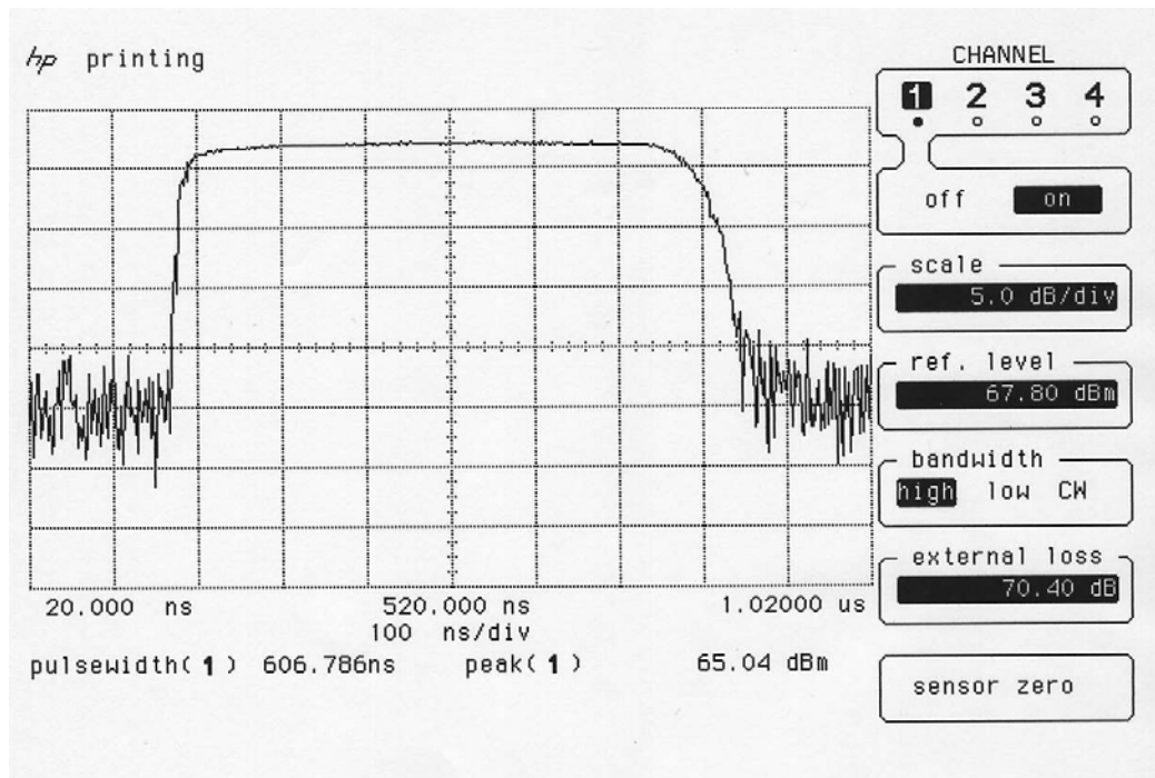
Graph PW/555/1002/07
