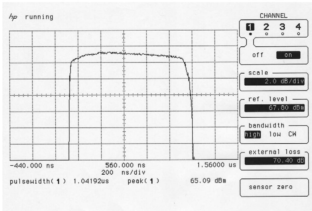
Graph PW/555/1002/08
