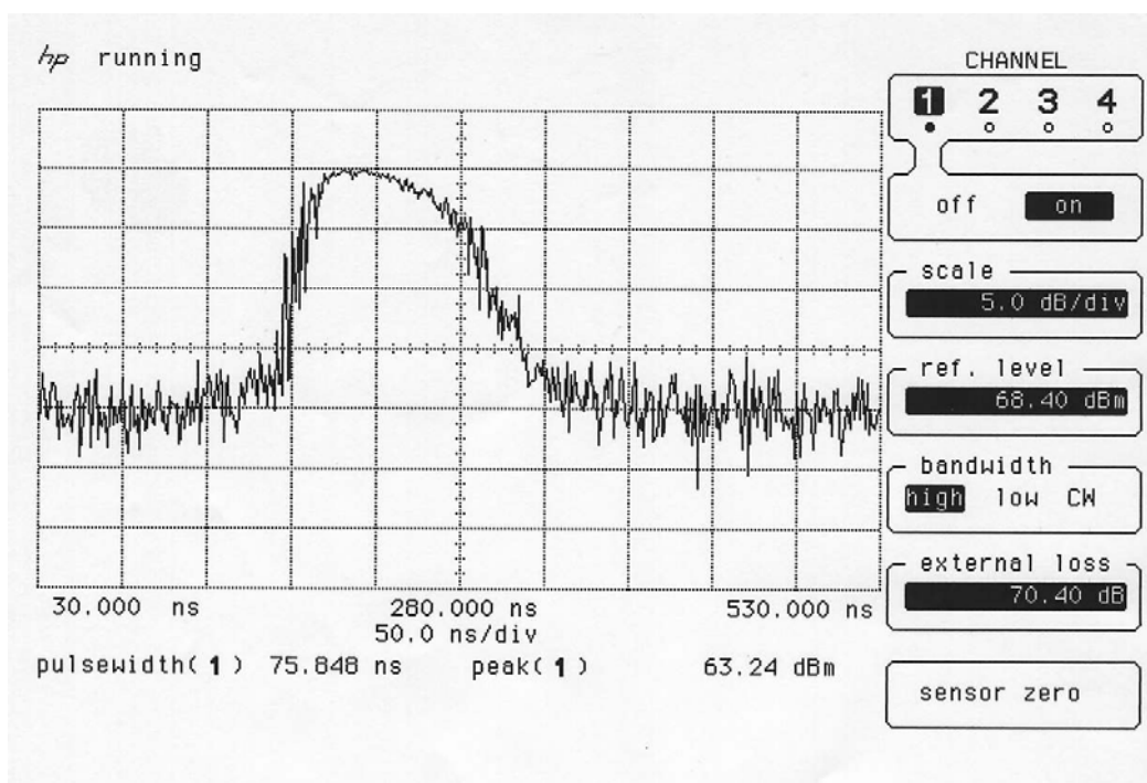
Graph PW/555/1002/01
