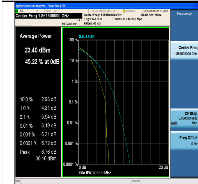
Band2-3MHz-16QAM-18615-1RB#0-PASS
