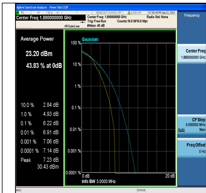
Band2-3MHz-16QAM-18900-1RB#0-PASS
