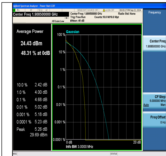
Band2-3MHz-QPSK-19185-1RB#0-PASS
