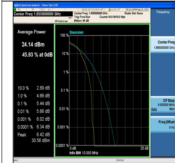
Band2-10MHz-16QAM-18650-1RB#0-PASS
