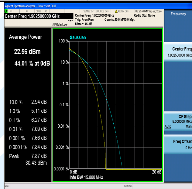
Band2-15MHz-16QAM-19125-75RB#0-PASS
