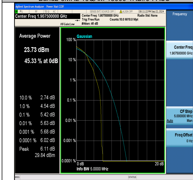
Band2-5MHz-16QAM-19175-1RB#0-PASS
