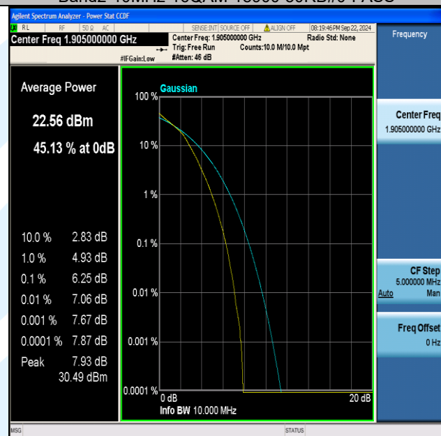
Band2-10MHz-16QAM-19150-50RB#0-PASS
