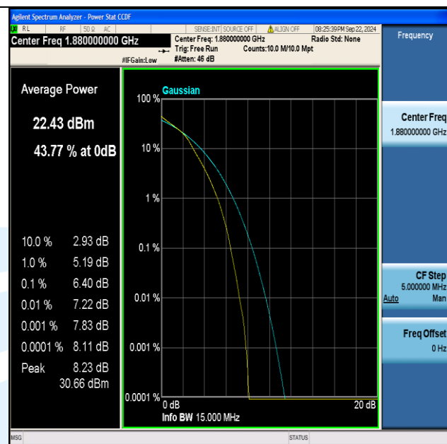
Band2-15MHz-16QAM-18900-75RB#0-PASS
