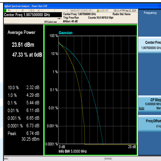
Band2-5MHz-QPSK-19175-25RB#0-PASS
