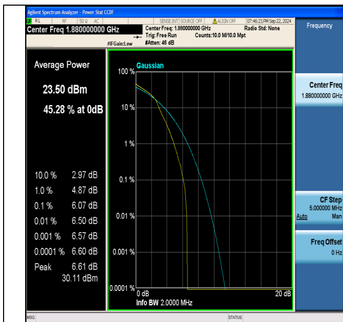
Band2-1.4MHz-16QAM-18900-1RB#0-PASS
