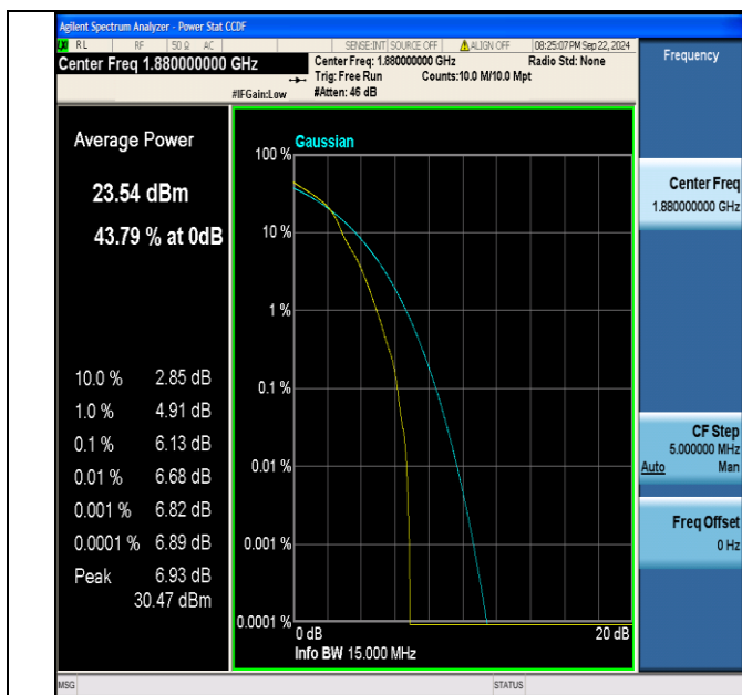
Band2-15MHz-16QAM-18900-1RB#0-PASS
