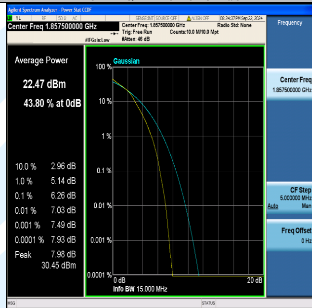
Band2-15MHz-16QAM-18675-75RB#0-PASS
