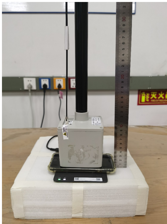
Photograph 4: Set-up photo for RF Exposure
