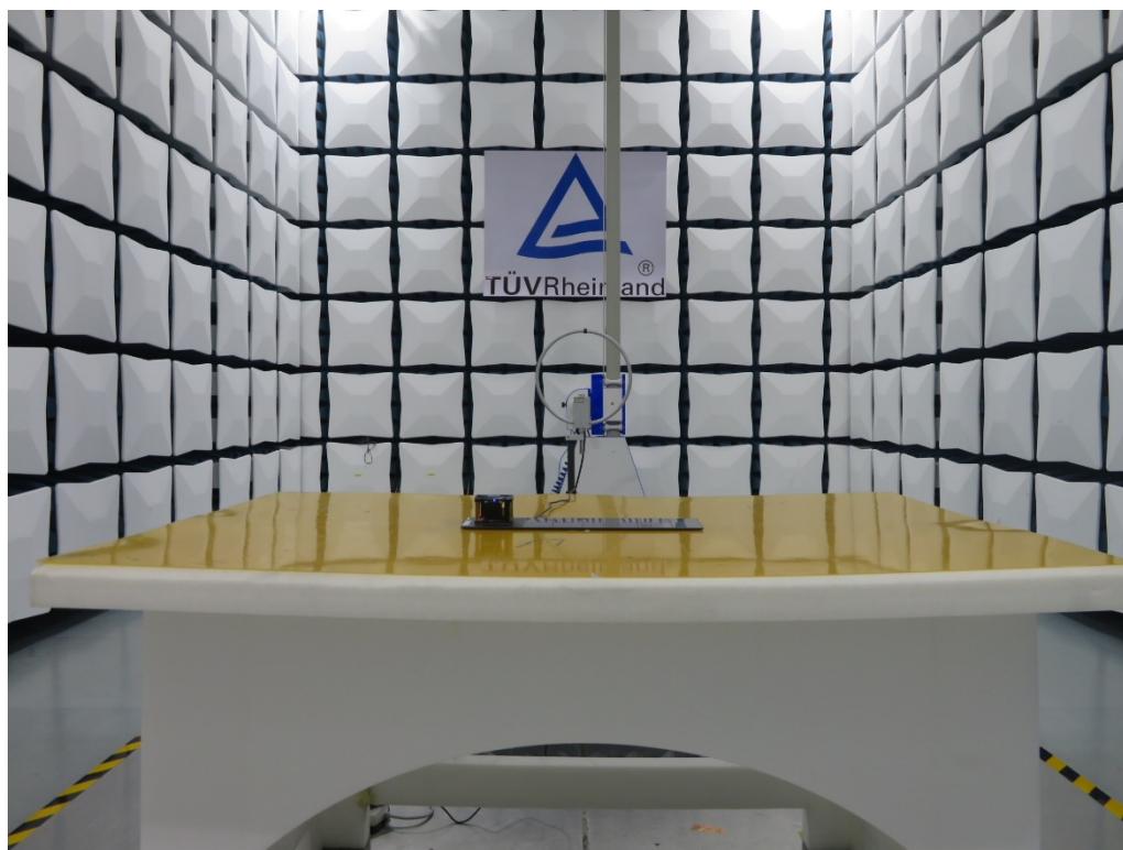
Photograph 1: Set-up photo for Radiated Emission, 9KHz - 30MHz
