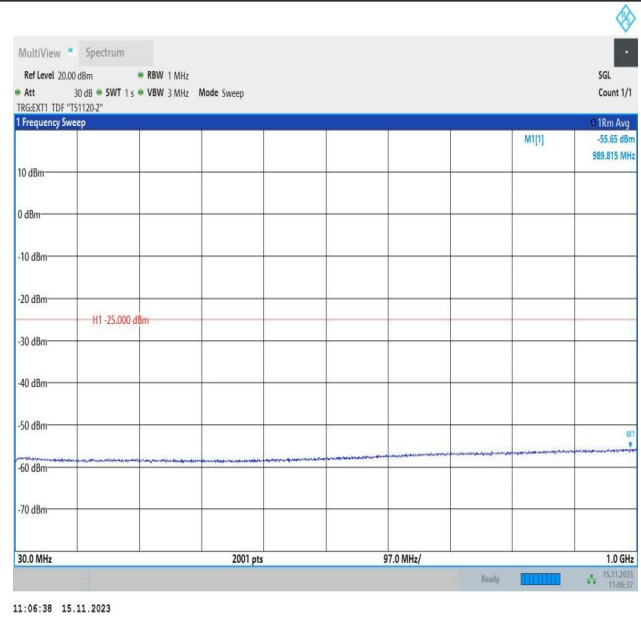
Band38_5MHz_16QAM_37775_1RB#0_30~1000_30~1000
