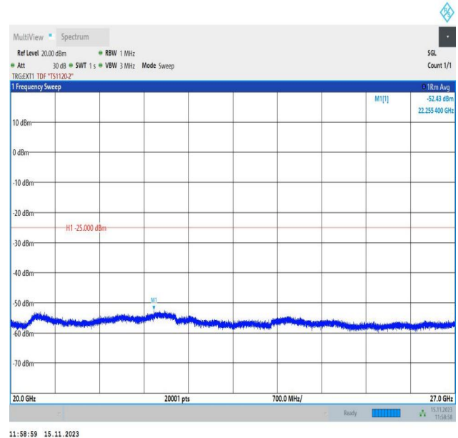
Band38_15MHz_16QAM_38000_1RB#0_20000~27000_20000~27000
