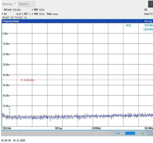
Band38_20MHz_16QAM_38150_1RB#0_0.15~30_0.15~30
