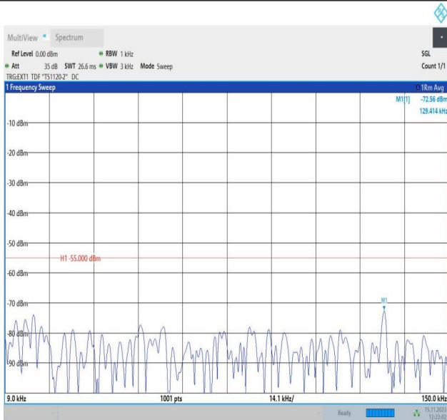
Band38_15MHz_16QAM_38175_1RB#0_1000~20000_1000~20000
