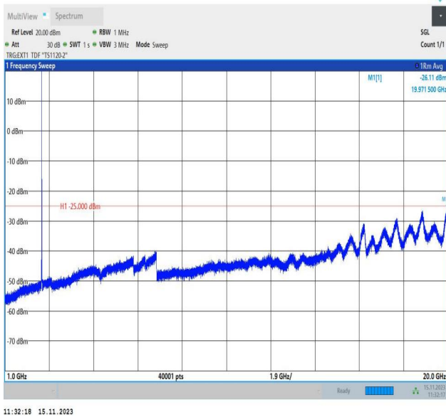
Band38_10MHz_16QAM_37800_1RB#0_1000~20000_1000~20000
