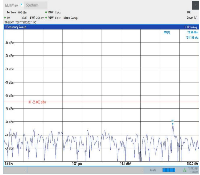
Band38_10MHz_16QAM_38000_1RB#0_0.009~0.15_0.009~0.15 15
