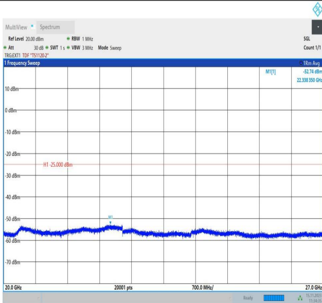
Band38_10MHz_QPSK_38200_1RB#0_20000~27000_20000~27000
