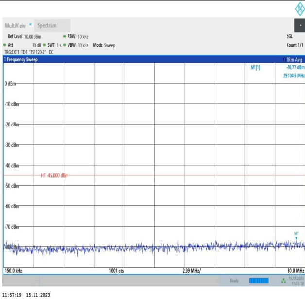
Band38_15MHz_16QAM_37825_1RB#0_0.15~30_0.15~30
