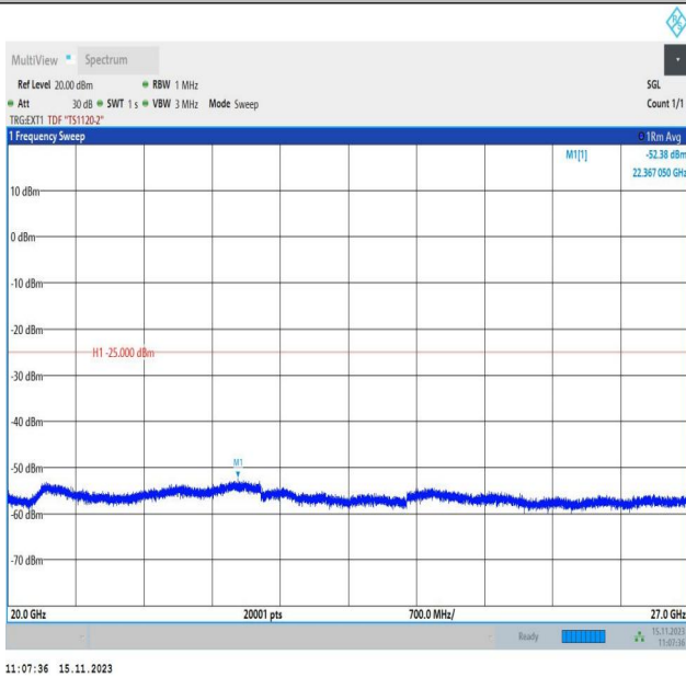
Band38_5MHz_QPSK_38000_1RB#0_20000~27000_20000~ 27000
