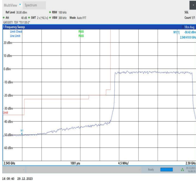
Band38_20MHz_64QAM_37850_100RB#0
