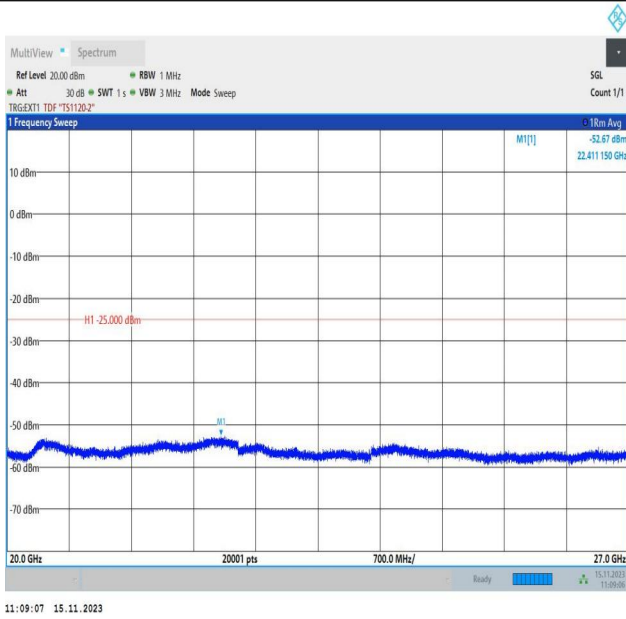
Band38_5MHz_QPSK_38225_1RB#0_20000~27000_20000~27000
