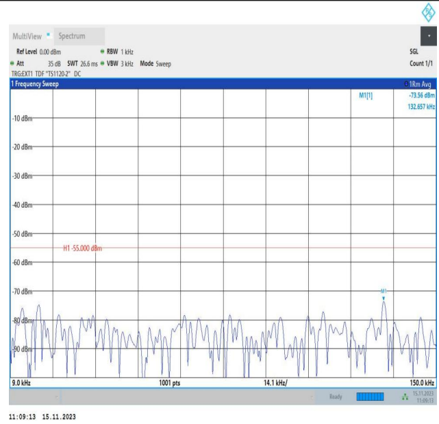
Band38_5MHz_16QAM_38225_1RB#0_0.009~0.15_0.009~0.15 5
