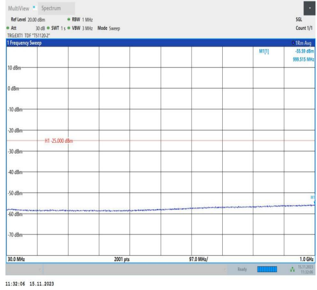
Band38_10MHz_16QAM_37800_1RB#0_30~1000_30~1000
