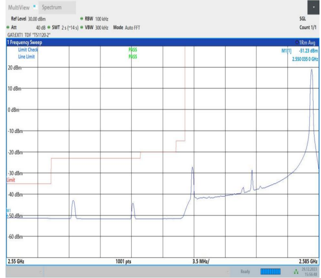
Band38_15MHz_64QAM_37825_1RB#74
