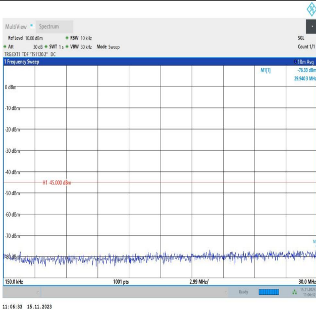
Band38_5MHz_16QAM_37775_1RB#0_0.15~30_0.15~30
