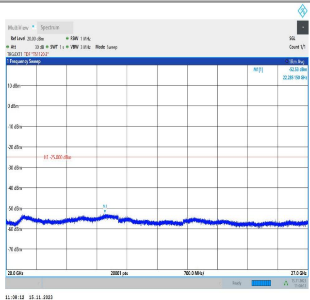
Band38_5MHz_16QAM_38000_1RB#0_20000~27000_20000~27000
