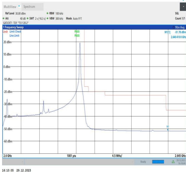
Band38_20MHz_64QAM_38150_1RB#99
