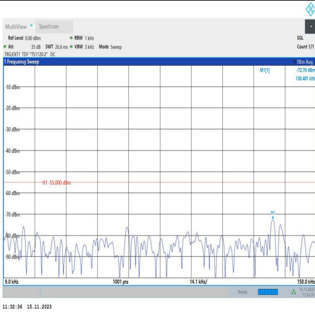
Band38_10MHz_QPSK_38000_1RB#0_0.009~0.15_0.009~0.
