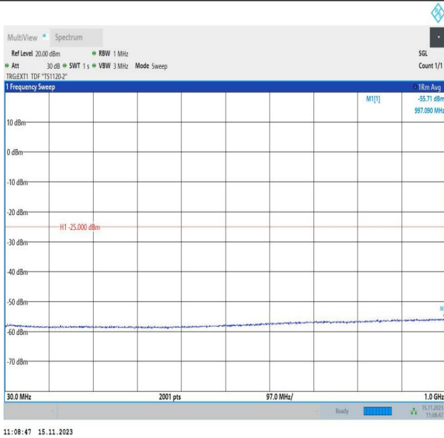
Band38_5MHz_QPSK_38225_1RB#0_30~1000_30~1000
