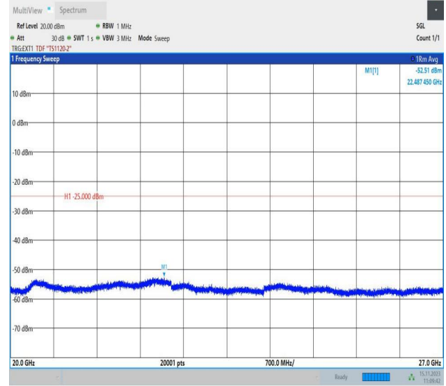
Band38_5MHz_16QAM_38225_1RB#0_20000~27000_20000~27000
