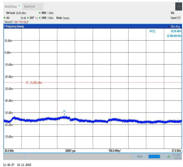
Band38_10MHz_16QAM_37800_1RB#0_20000~27000_20000~27000
