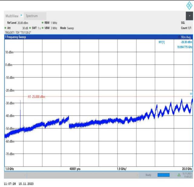
Band38_5MHz_QPSK_38000_1RB#0_1000~20000_1000~200 00
