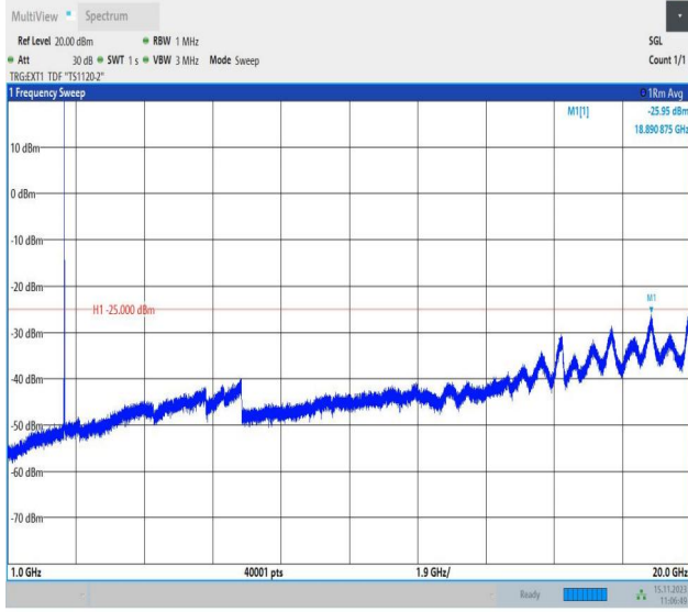
Band38_5MHz_16QAM_37775_1RB#0_1000~20000_1000~20000
