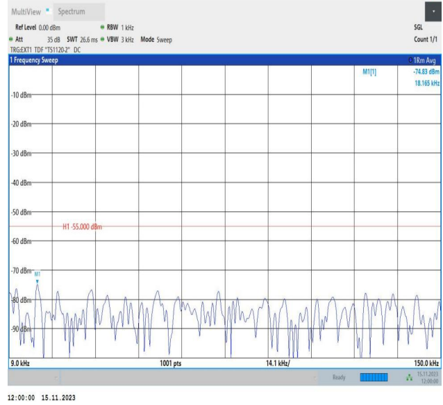
Band38_15MHz_16QAM_38175_1RB#0_0.009~0.15_0.009~0.15 15
