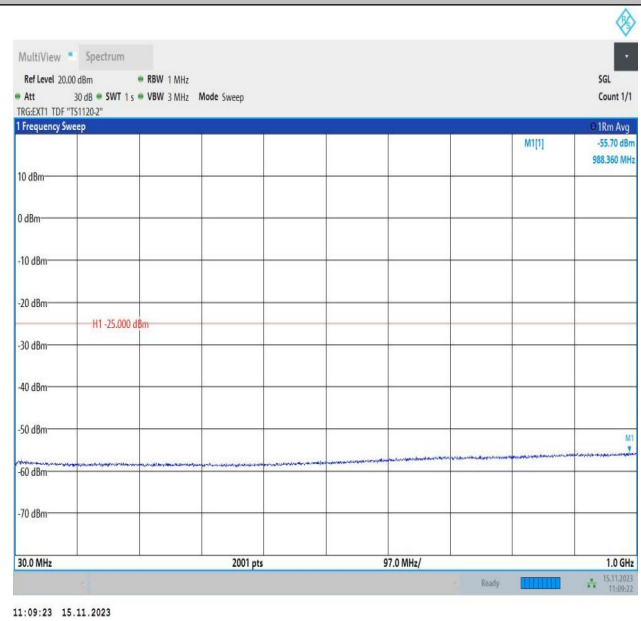
Band38_5MHz_16QAM_38225_1RB#0_30~1000_30~1000
