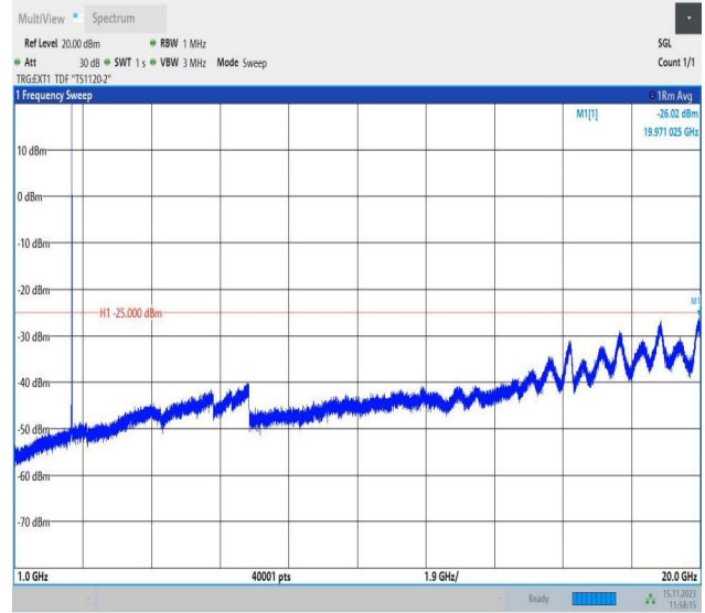
Band38_15MHz_QPSK_38000_1RB#0_1000~20000_1000~20000
