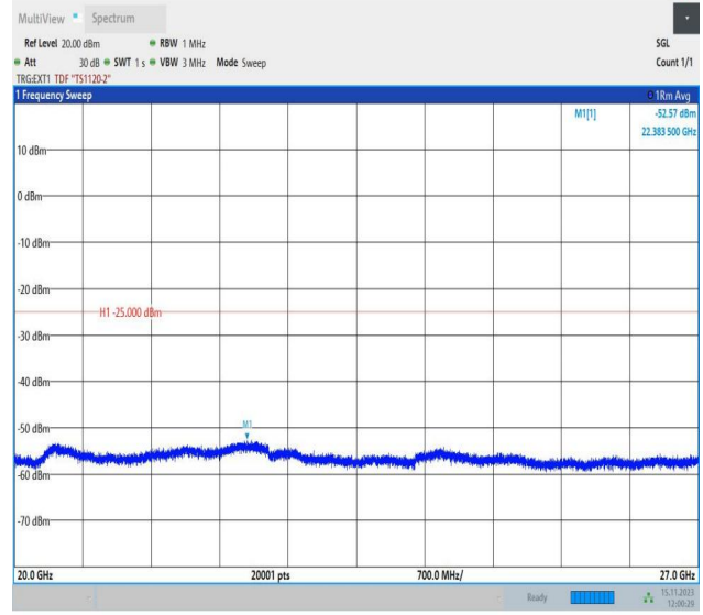
Band38_15MHz_16QAM_38175_1RB#0_20000~27000_20000~27000
