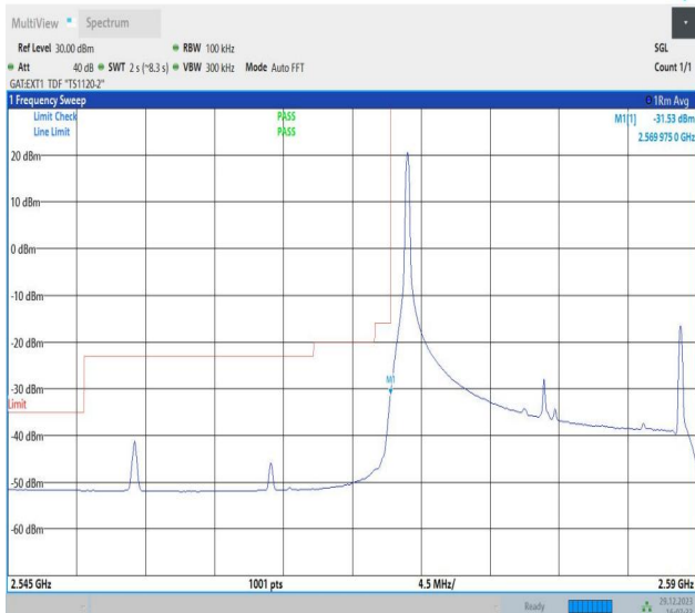
Band38_20MHz_64QAM_37850_1RB#0
