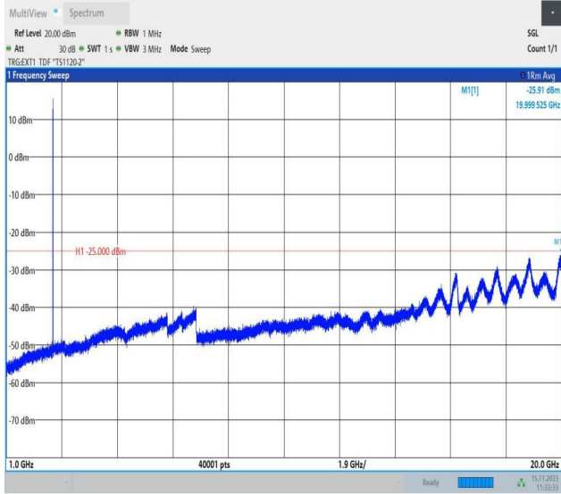
Band38_10MHz_16QAM_38000_1RB#0_1000~20000_1000~20000
