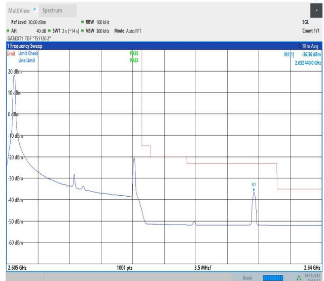
Band38_15MHz_64QAM_38175_1RB#0
