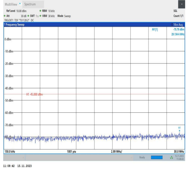
Band38_5MHz_QPSK_38225_1RB#0_0.15~30_0.15~30
