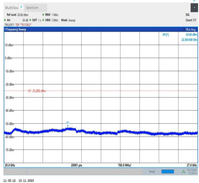
Band38_10MHz_16QAM_38200_1RB#0_20000~27000_20000~27000
