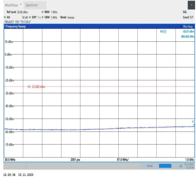
Band38_20MHz_16QAM_38150_1RB#0_30~1000_30~1000
