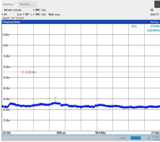
Band38_15MHz_QPSK_37825_1RB#0_20000~27000_20000 ~27000
