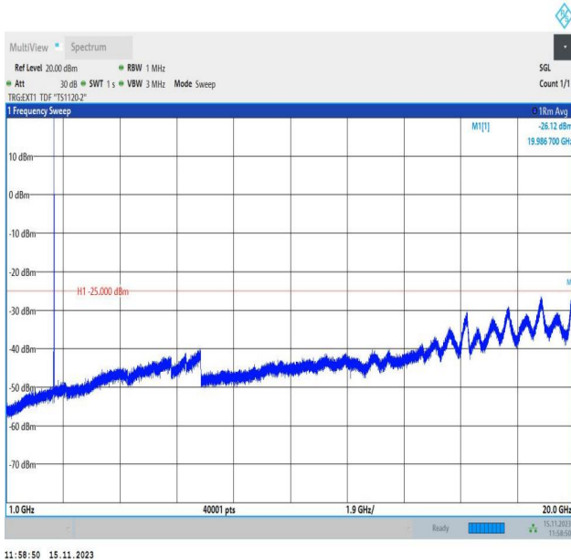
Band38_15MHz_16QAM_38000_1RB#0_1000~20000_1000~20000
