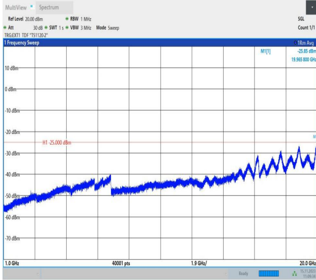
Band38_5MHz_16QAM_38225_1RB#0_1000~20000_1000~20000
