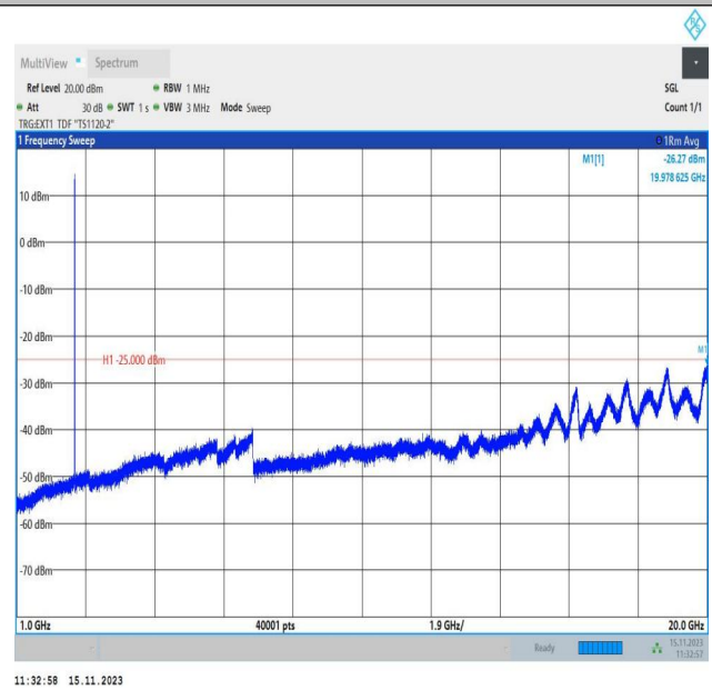
Band38_10MHz_QPSK_38000_1RB#0_1000~20000_1000~20000
