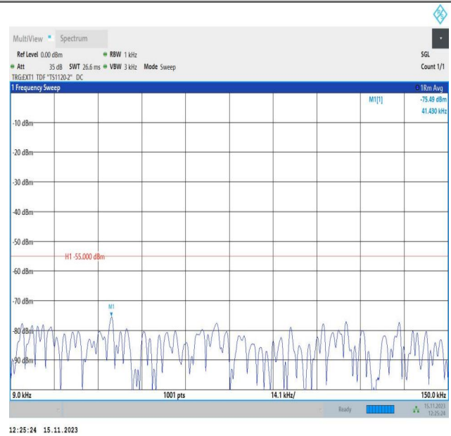
Band38_20MHz_16QAM_38150_1RB#0_0.009~0.15_0.009~0.15
