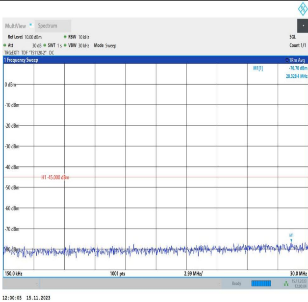
Band38_15MHz_16QAM_38175_1RB#0_0.15~30_0.15~30
