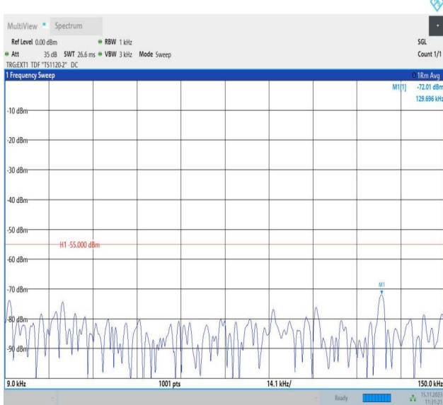
Band38_10MHz_QPSK_37800_1RB#0_0.009~0.15_0.009~0.15
