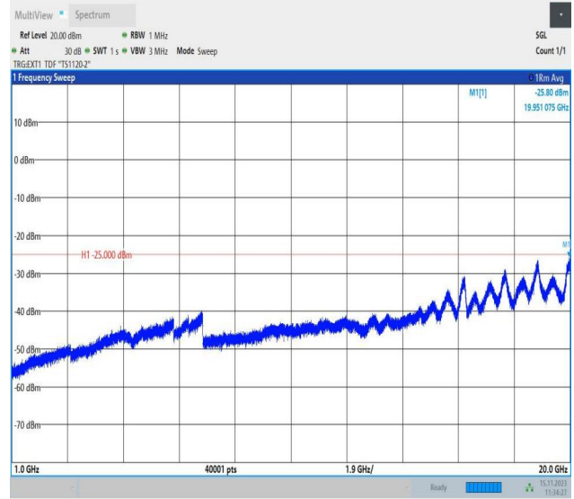
Band38_10MHz_QPSK_38200_1RB#0_1000~20000_1000~20000
