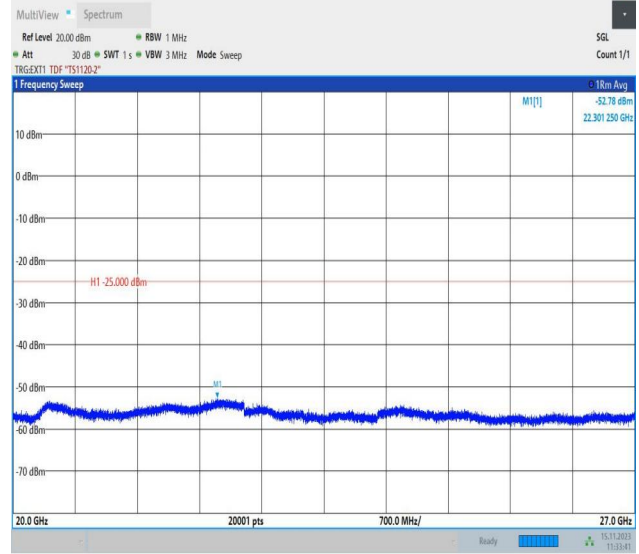
Band38_10MHz_16QAM_38000_1RB#0_20000~27000_20000~27000
