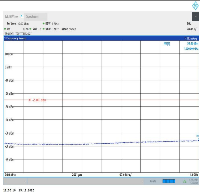
Band38_15MHz_16QAM_38175_1RB#0_30~1000_30~1000
