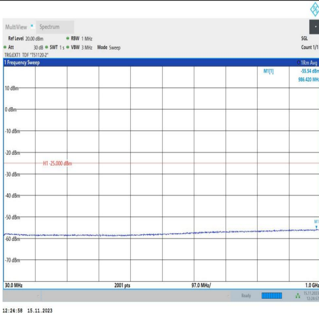
Band38_20MHz_QPSK_38150_1RB#0_30~1000_30~1000
