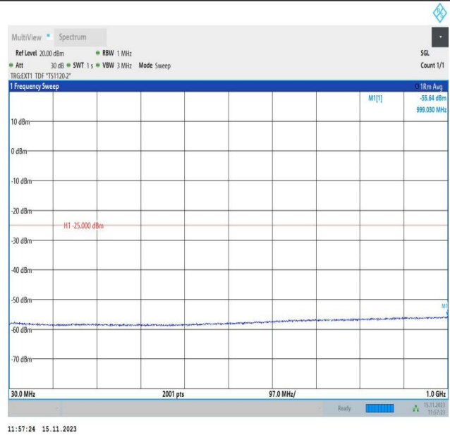
Band38_15MHz_16QAM_37825_1RB#0_30~1000_30~1000
