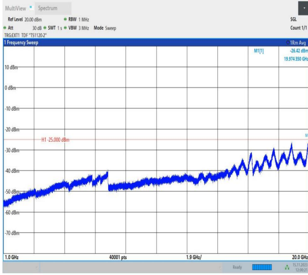
Band38_15MHz_16QAM_38175_1RB#0_1000~20000_1000~20000
