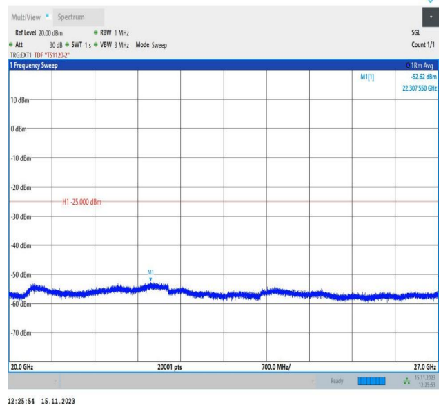
Band38_20MHz_16QAM_38150_1RB#0_20000~27000_20000~27000
