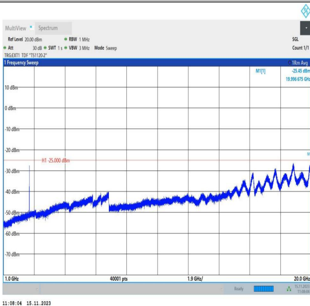
Band38_5MHz_16QAM_38000_1RB#0_1000~20000_1000~20000
