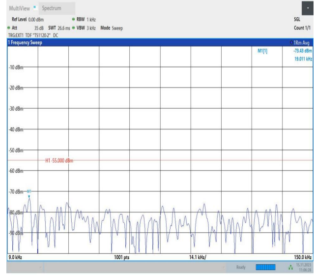
Band38_5MHz_16QAM_37775_1RB#0_0.009~0.15_0.009~0.15 5
