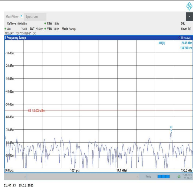
Band38_5MHz_16QAM_38000_1RB#0_0.009~0.15_0.009~0.1 5
