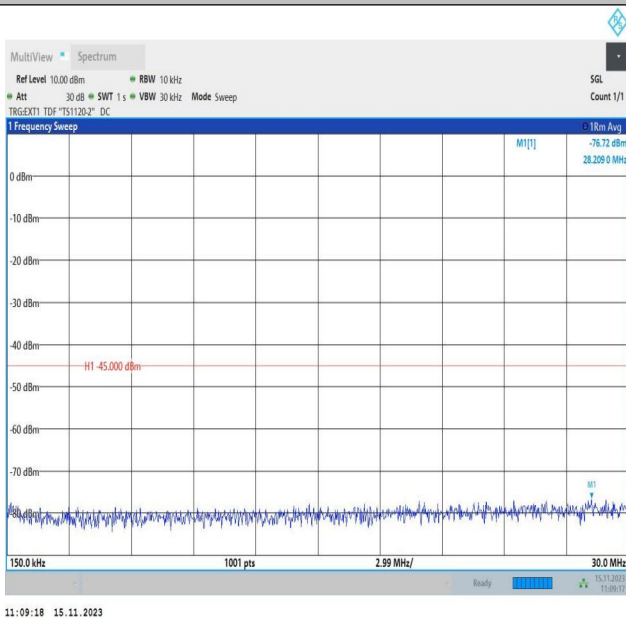
Band38_5MHz_16QAM_38225_1RB#0_0.15~30_0.15~30
