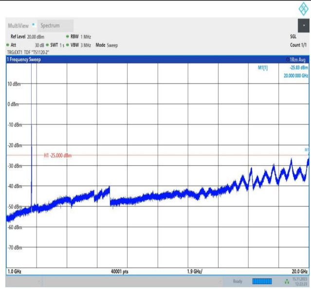
Band38_20MHz_QPSK_37850_1RB#0_1000~20000_1000~20000
