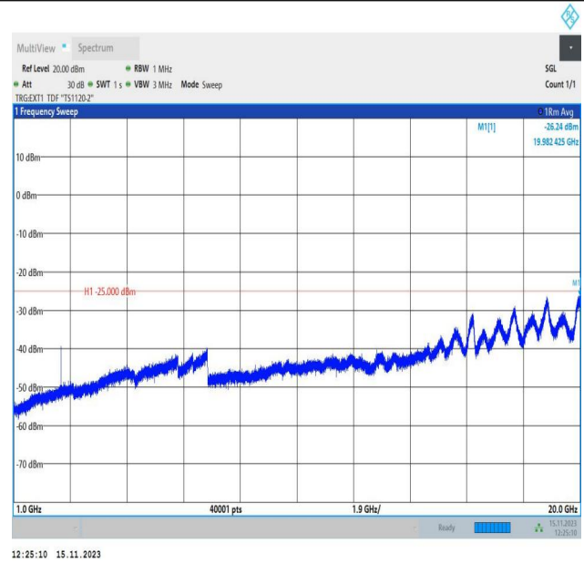
Band38_20MHz_QPSK_38150_1RB#0_1000~20000_1000~20000
