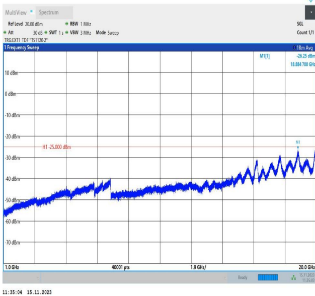
Band38_10MHz_16QAM_38200_1RB#0_1000~20000_1000~20000
