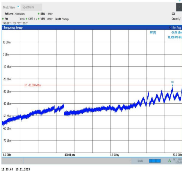
Band38_20MHz_16QAM_38150_1RB#0_1000~20000_1000~20000
