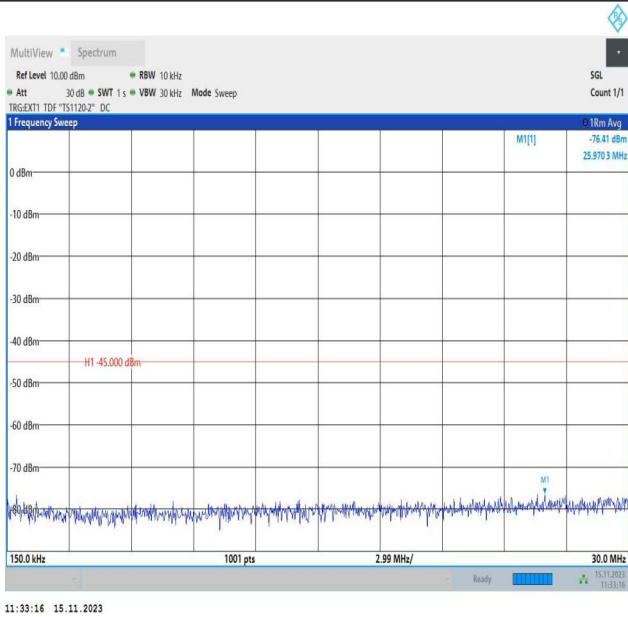
Band38_10MHz_16QAM_38000_1RB#0_0.15~30_0.15~30
