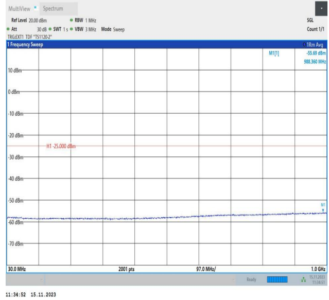
Band38_10MHz_16QAM_38200_1RB#0_30~1000_30~1000
