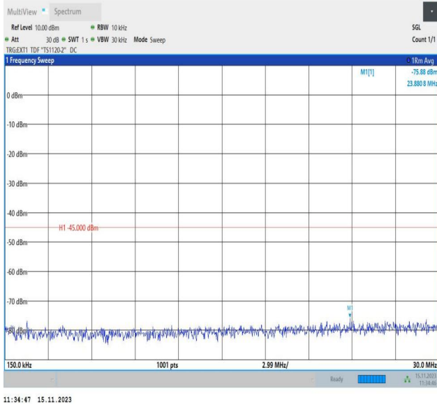
Band38_10MHz_16QAM_38200_1RB#0_0.15~30_0.15~30
