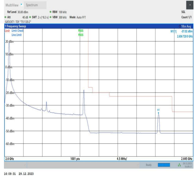
Band38_20MHz_64QAM_38150_1RB#0
