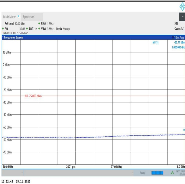
Band38_10MHz_QPSK_38000_1RB#0_30~1000_30~1000
