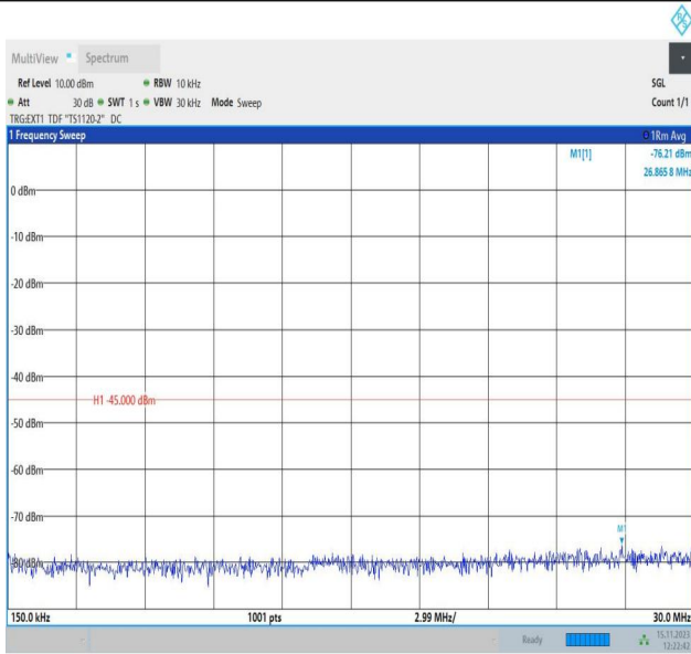
Band38_20MHz_16QAM_37850_1RB#0_0.15~30_0.15~30
