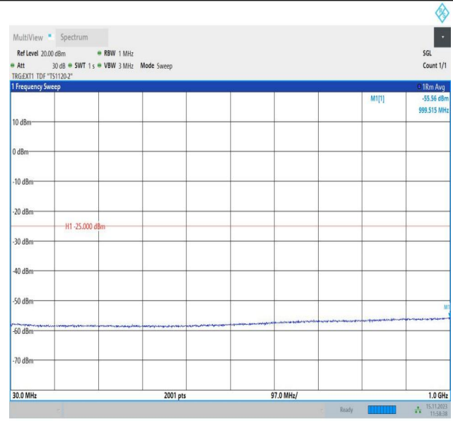
Band38_15MHz_16QAM_38000_1RB#0_30~1000_30~1000
