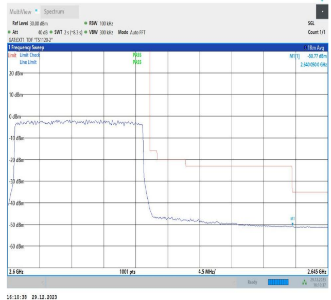
Band38_20MHz_64QAM_38150_100RB#0
