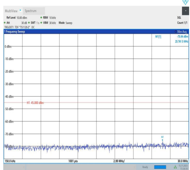
Band38_10MHz_QPSK_38200_1RB#0_0.15~30_0.15~30
