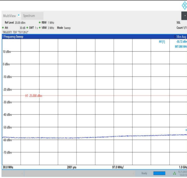
Band38_20MHz_QPSK_37850_1RB#0_30~1000_30~1000
