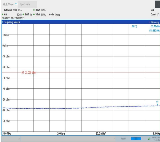
Band38_10MHz_QPSK_38200_1RB#0_30~1000_30~1000
