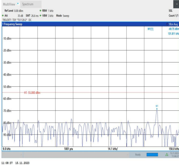
Band38_5MHz_QPSK_38225_1RB#0_0.009~0.15_0.009~0.1
