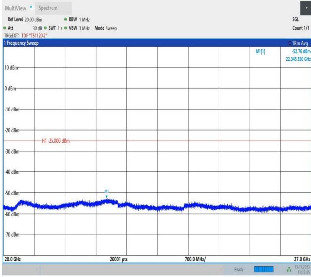
Band38_10MHz_QPSK_38000_1RB#0_20000~27000_20000 ~27000
