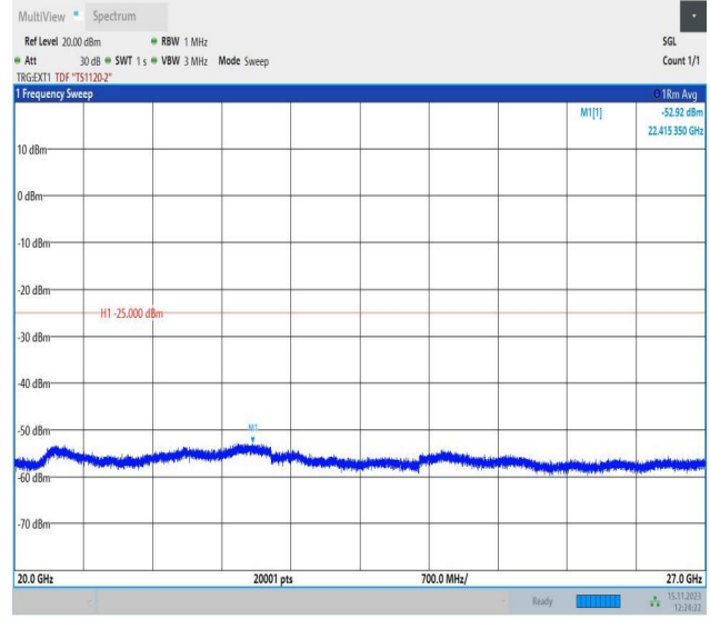
Band38_20MHz_16QAM_38000_1RB#0_20000~27000_20000~27000
