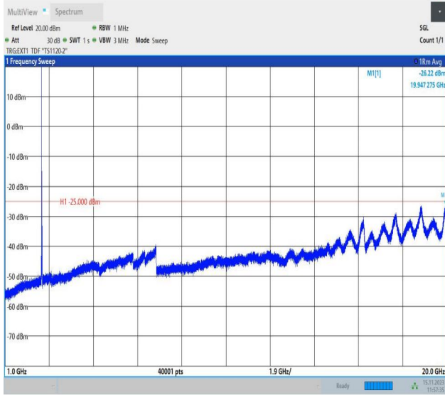
Band38_15MHz_16QAM_37825_1RB#0_1000~20000_1000~20000
