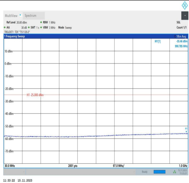
Band38_10MHz_16QAM_38000_1RB#0_30~1000_30~1000
