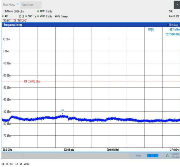
Band38_15MHz_QPSK_38175_1RB#0_20000~27000_20000 ~27000
