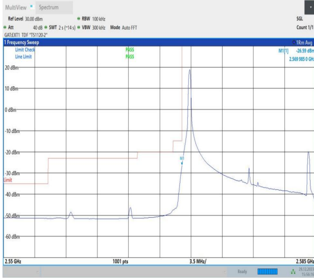
Band38_15MHz_64QAM_37825_1RB#0
