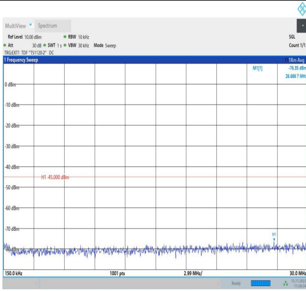
Band38_15MHz_16QAM_38000_1RB#0_0.15~30_0.15~30
