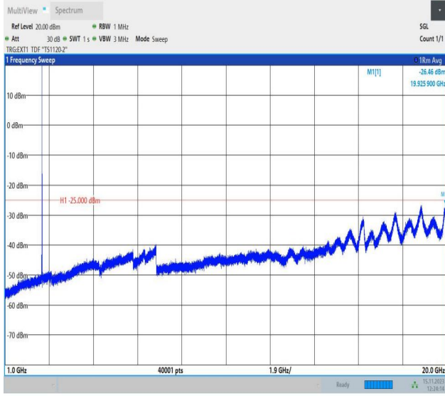
Band38_20MHz_16QAM_38000_1RB#0_1000~20000_1000~20000
