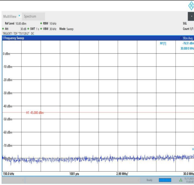
Band38_5MHz_16QAM_38000_1RB#0_0.15~30_0.15~30
