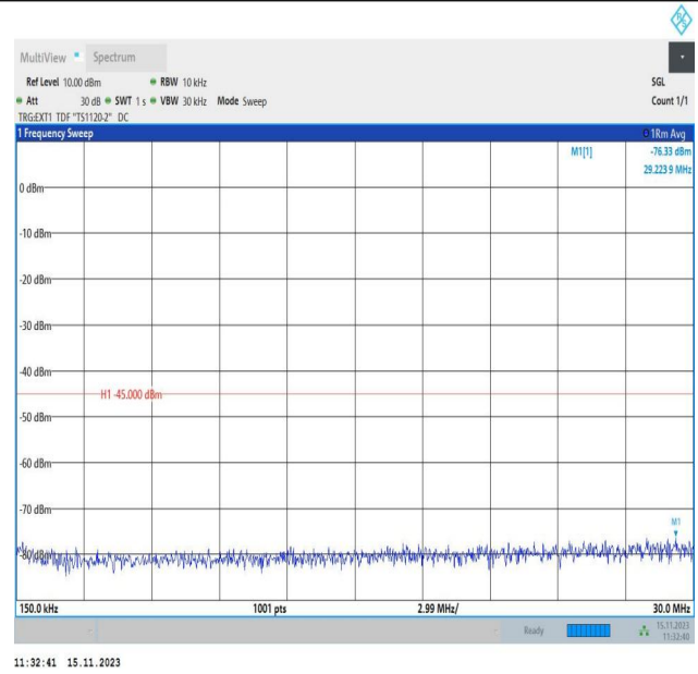
Band38_10MHz_QPSK_38000_1RB#0_0.15~30_0.15~30
