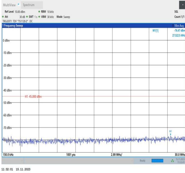
Band38_10MHz_16QAM_37800_1RB#0_0.15~30_0.15~30
