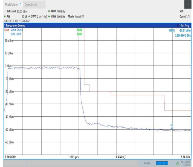
Band38_15MHz_64QAM_38175_75RB#0
