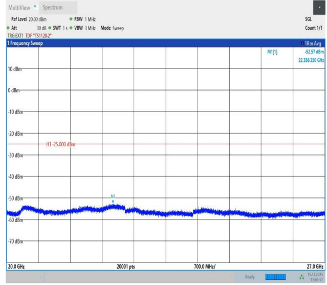
Band38_5MHz_16QAM_37775_1RB#0_20000~27000_20000~27000
