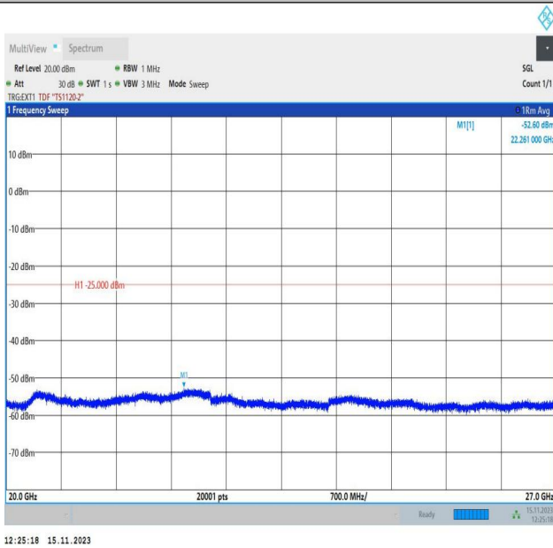
Band38_20MHz_QPSK_38150_1RB#0_20000~27000_20000~27000
