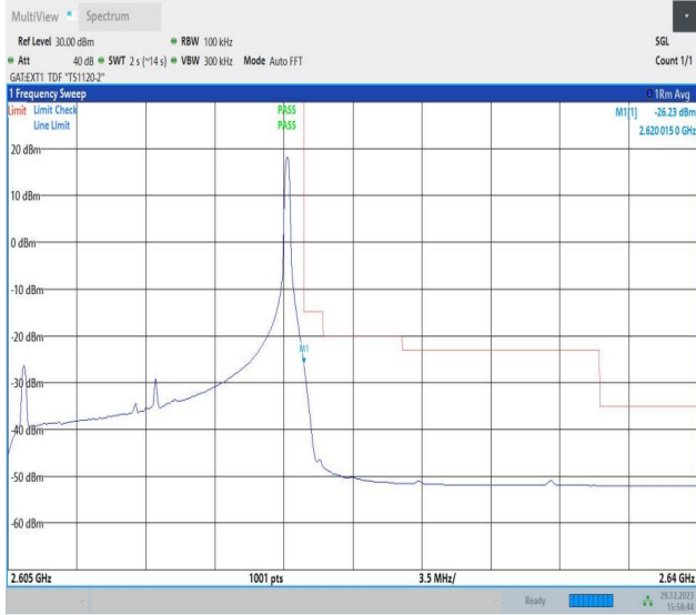
Band38_15MHz_64QAM_38175_1RB#74
