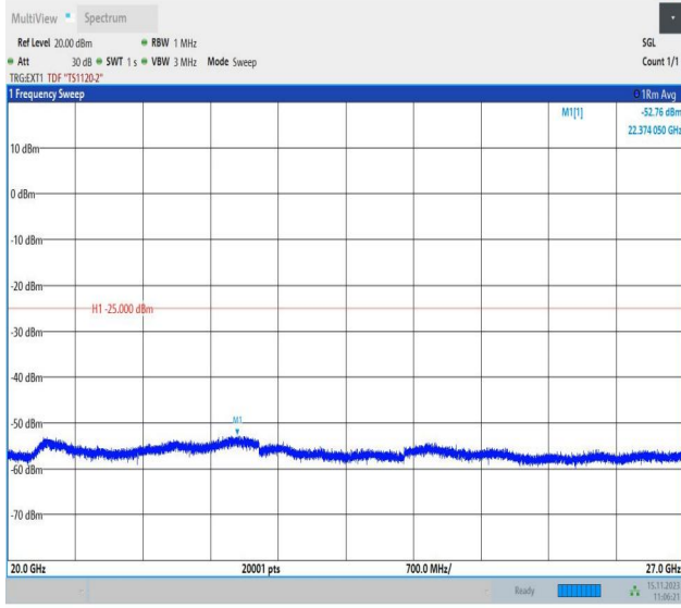
Band38_5MHz_QPSK_37775_1RB#0_20000~27000_20000~27000
