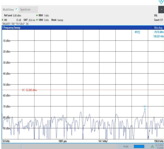
Band38_10MHz_QPSK_38200_1RB#0_0.009~0.15_0.009~0.15
