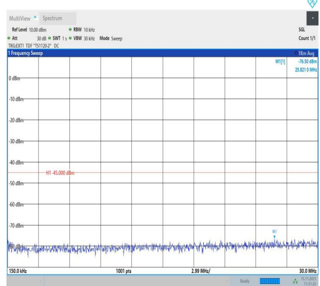
Band38_10MHz_QPSK_37800_1RB#0_0.15~30_0.15~30
