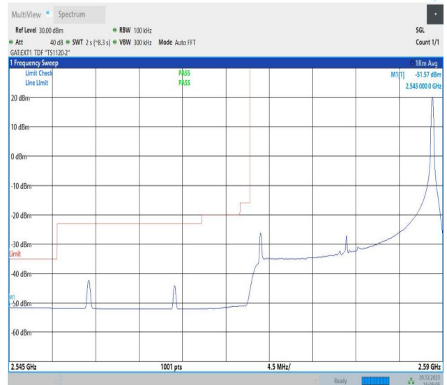
Band38_20MHz_64QAM_37850_1RB#99
