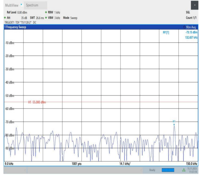
Band38_15MHz_16QAM_37825_1RB#0_0.009~0.15_0.009~0.15 15
