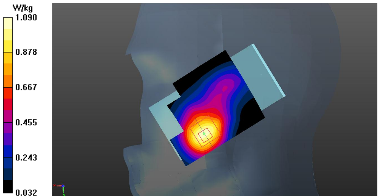
Fig.3 GSM 1900 Head
