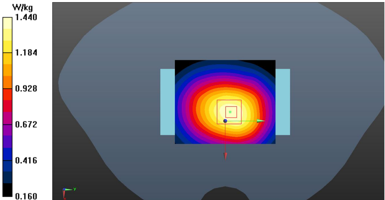
Fig.2 GSM 850 Body-worn
