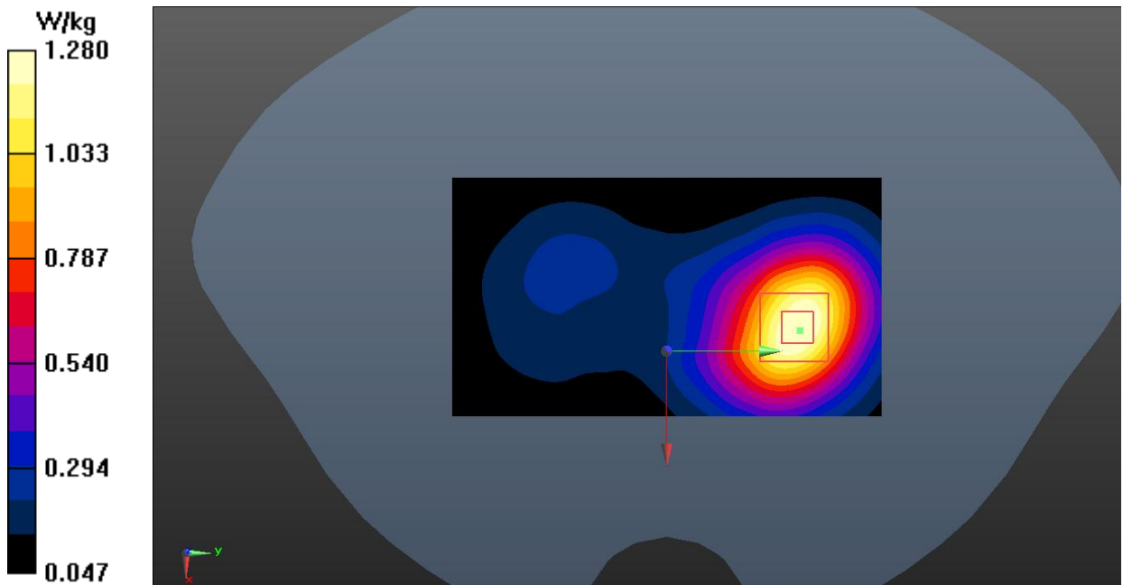
Fig.4 GSM 1900 Body-worn
