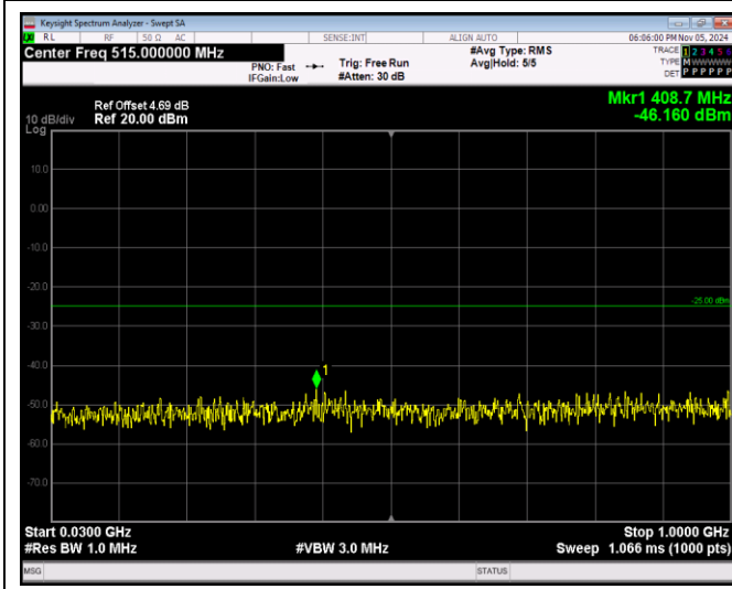
Band41-5MHz-64QAM-41215-1RB#0-Range1:30~100 OMHz
