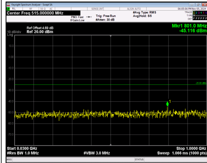
Band41-5MHz-64QAM-41215-1RB#0-Range1:30~100 OMHz
