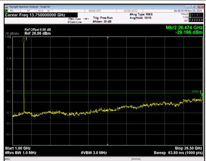
Band41-20MHz-64QAM-40640-1RB#0-Range2:1000~26500MHz
