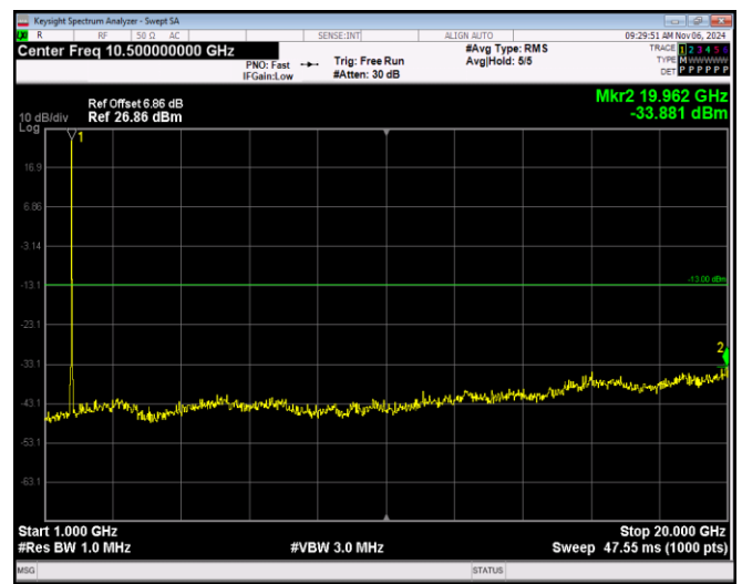
Band66-20MHz-16QAM-132072-1RB#0-Range2:1000~20000MHz
