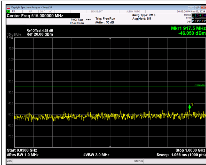
Band41-5MHz-64QAM-40640-1RB#0-Range1:30~100 OMHz
