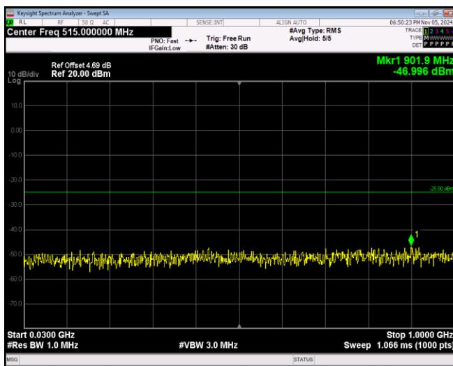
Band41-20MHz-64QAM-40140-1RB#0-Range1:30~1000MHz
