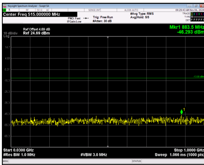
Band66-20MHz-16QAM-132072-1RB#0-Range1:30~1000MHz
