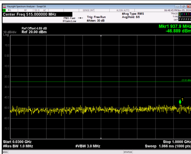
Band41-20MHz-64QAM-40640-1RB#0-Range1:30~1000MHz
