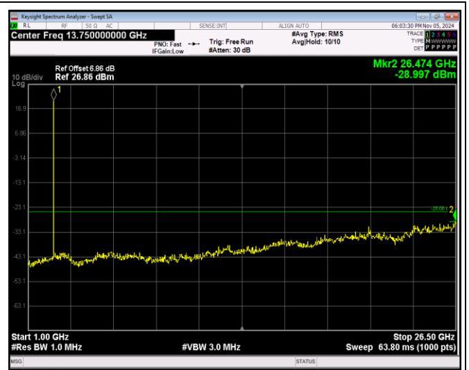
Band41-5MHz-64QAM-40640-1RB#0-Range2:1000~2 6500MHz
