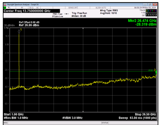
Band41-20MHz-64QAM-40140-1RB#0-Range2:1000~26500MHz
