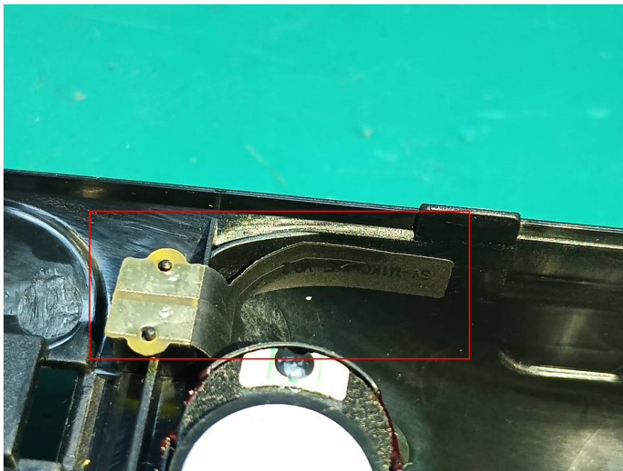
BT/Wi-Fi Antenna
