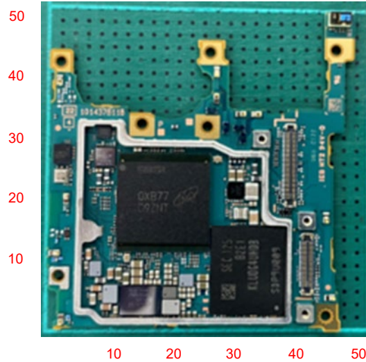
Internal Main-PWB Front without Shield cases (Front-side)
