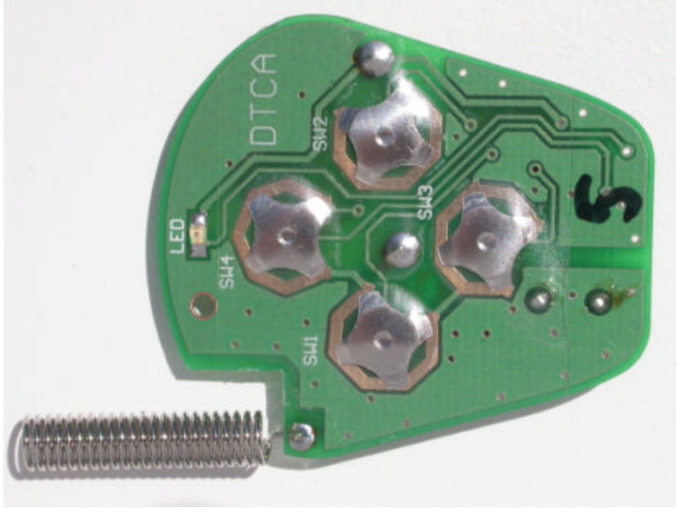
TOP SIDE OF PCB
