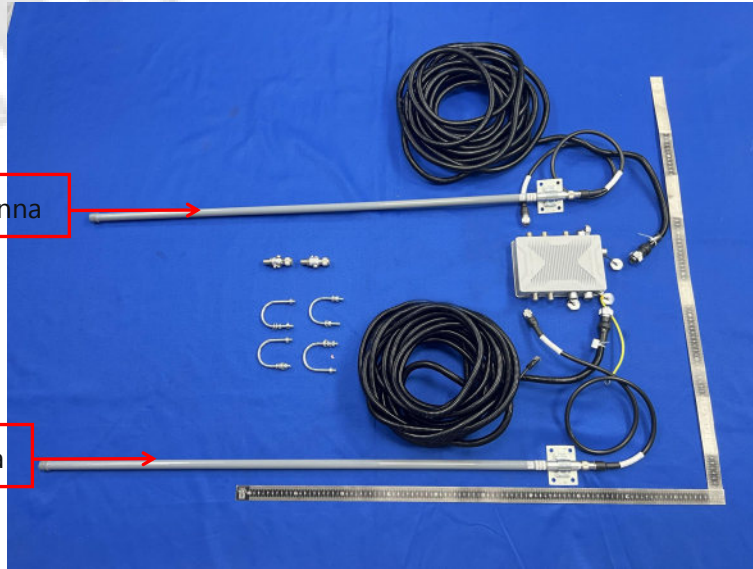
Transmitter antenna
