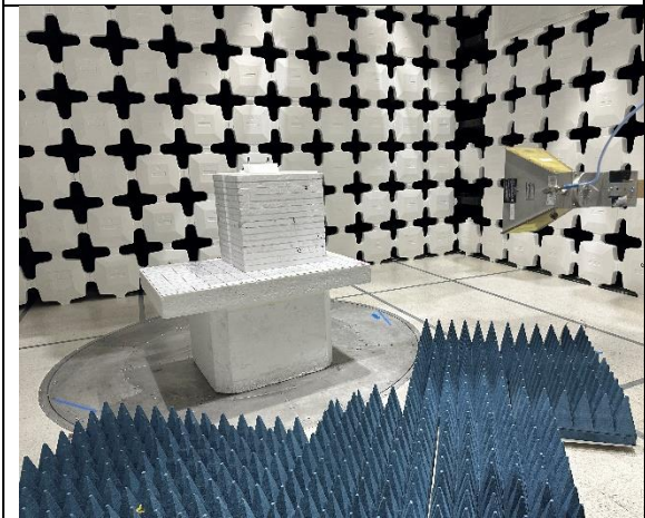
Huber+SUHNER Antenna Radiated Emission-Above 1GHz-Front
