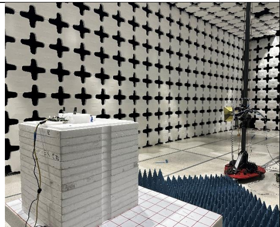
Huber+SUHNER Antenna Radiated Emission-Above 1GHz-Back
