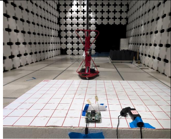
2JF0188P Antenna Radiated Emission-Below 1GHz-Back
