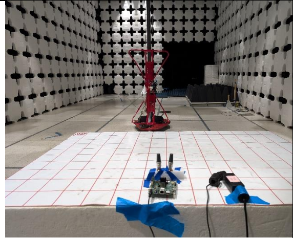
Huber+SUHNER Antenna Radiated Emission-Below 1GHz-Back
