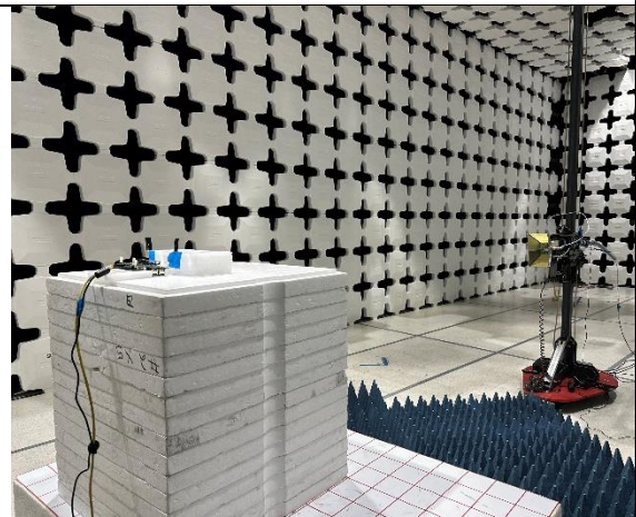
2JF0188P Antenna Radiated Emission-Above 1GHz-Back
