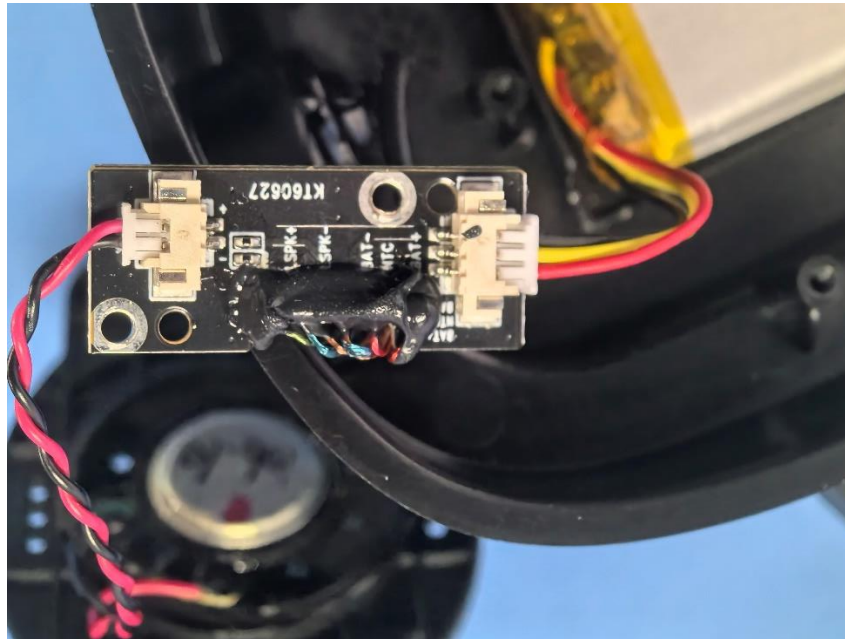
Internal View 7#
