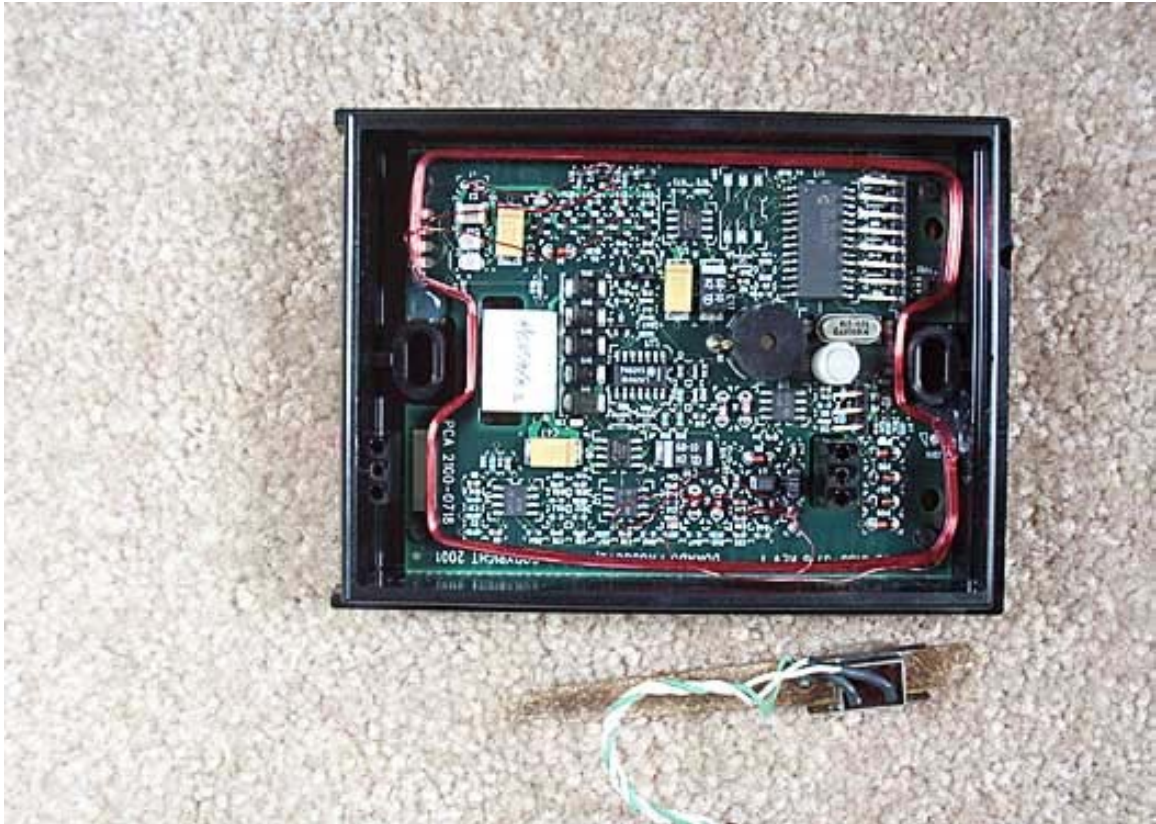
PCB Component Side
