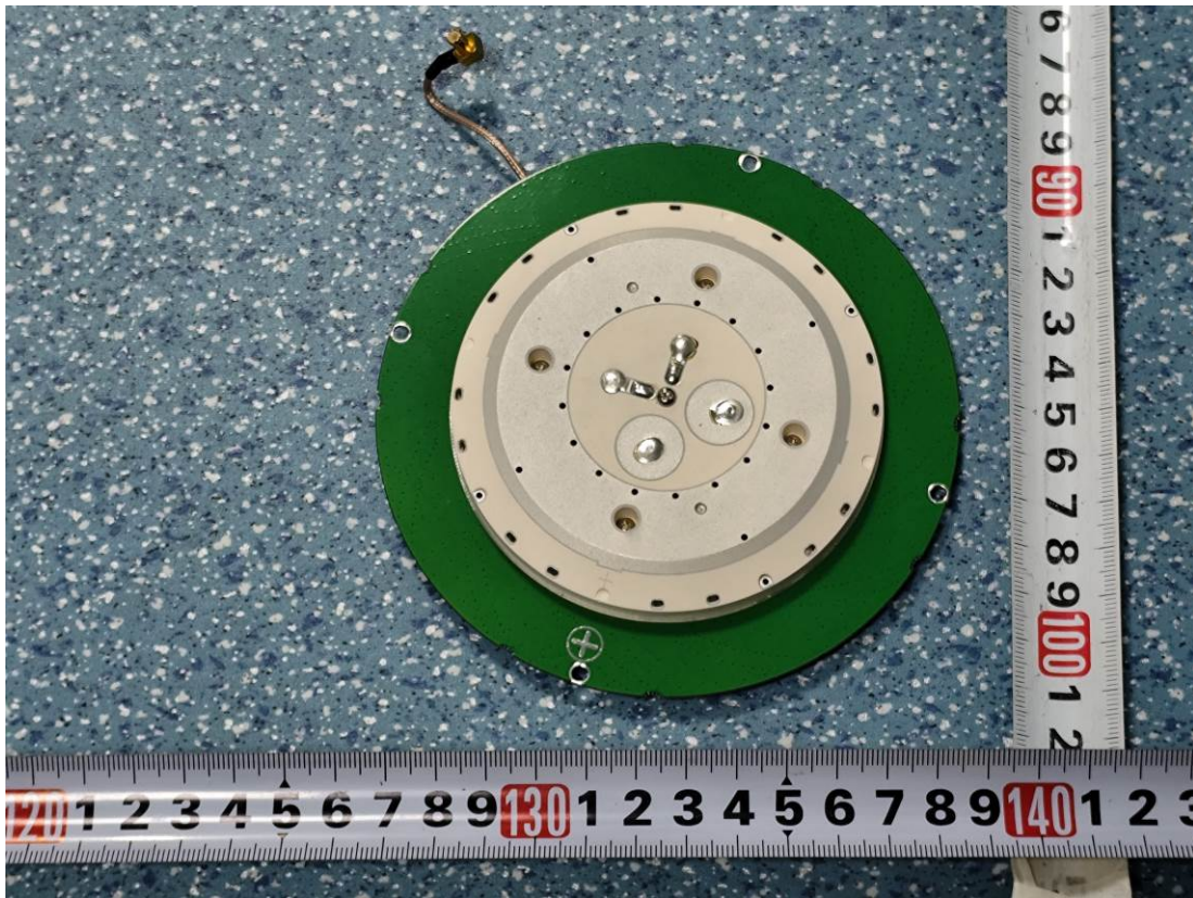
GNSS Antenna
