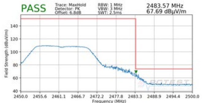
Plot 7-54. Radiated Restricted Upper Band Edge Measurement (Peak)
