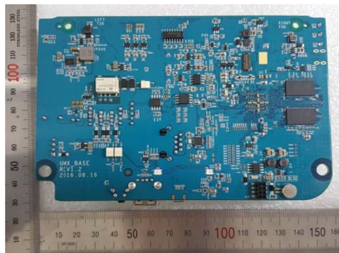
View of Main Board (Bottom)
