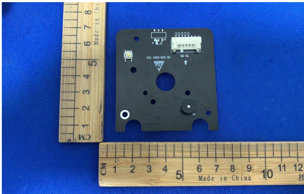
Figure 4. Internal view
