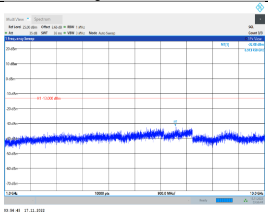
Band13-10MHz-64QAM-23230-1RB#0- Range2:1000~10000MHz
