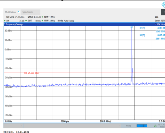
Band7-5MHz-16QAM-21425-1RB#0- Range2:1000~3000MHz
