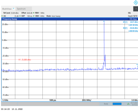
Band7-10MHz-16QAM-20800-1RB#0- Range2:1000~3000MHz
