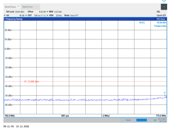
Band13-5MHz-16QAM-23230-1RB#0- Range3:763~775MHz
