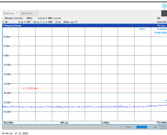
Band13-5MHz-64QAM-23230-1RB#0- Range3:763~775MHz
