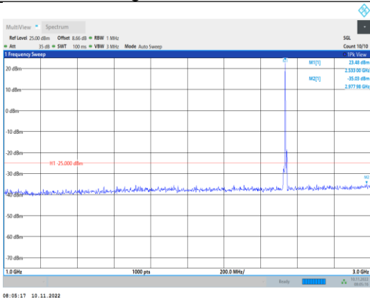
Band7-5MHz-16QAM-21100-1RB#0- Range2:1000~3000MHz
