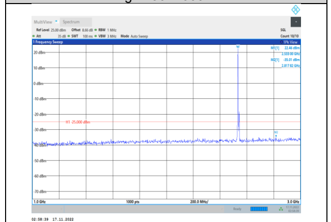
Band7-5MHz-64QAM-21100-1RB#0- Range2:1000~3000MHz
