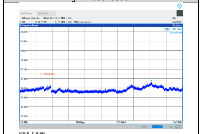
Band7-5MHz-64QAM-21100-1RB#0- Range3:3000~26500MHz
