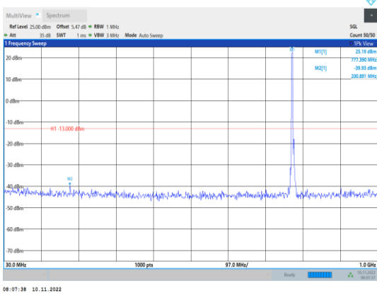
Band13-5MHz-QPSK-23205-1RB#0- Range1:30~1000MHz
