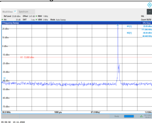
Band13-10MHz-16QAM-23230-1RB#0- Range1:30~1000MHz
