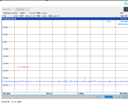
Band13-5MHz-64QAM-23230-1RB#0- Range4:793~805MHz
