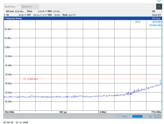
Band13-10MHz-16QAM-23230-1RB#0- Range3:763~775MHz
