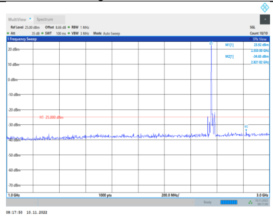
Band7-15MHz-QPSK-21375-1RB#0- Range2:1000~3000MHz
