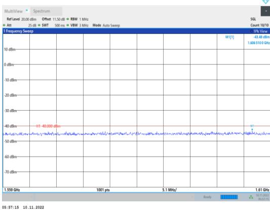
Band13-10MHz-16QAM-23230-1RB#0- Range5:1559~1610MHz
