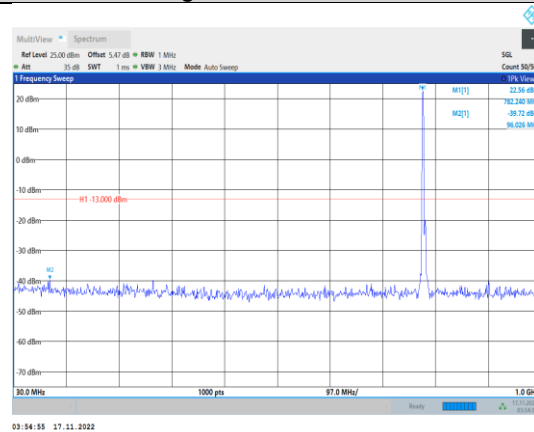
Band13-5MHz-64QAM-23255-1RB#0- Range1:30~1000MHz
