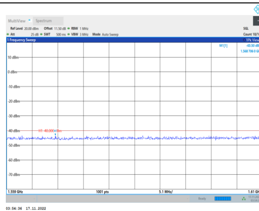
Band13-5MHz-64QAM-23230-1RB#0- Range5:1559~1610MHz
