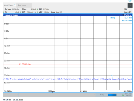
Band13-5MHz-16QAM-23255-1RB#0- Range4:793~805MHz
