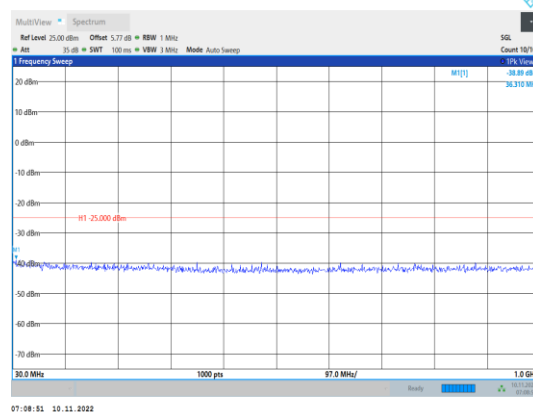
Band7-20MHz-QPSK-21100-1RB#0- Range1:30~1000MHz
