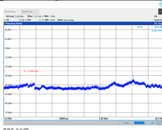
Band7-5MHz-16QAM-20775-1RB#0- Range3:3000~26500MHz
