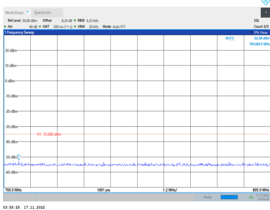
Band13-5MHz-64QAM-23255-1RB#0- Range4:793~805MHz
