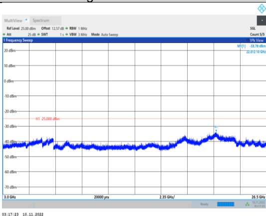
Band7-10MHz-16QAM-21400-1RB#0- Range3:3000~26500MHz
