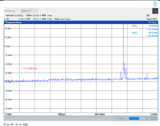
Band7-20MHz-16QAM-21350-1RB#0- Range2:1000~3000MHz
