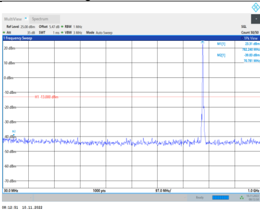
Band13-5MHz-16QAM-23255-1RB#0- Range1:30~1000MHz
