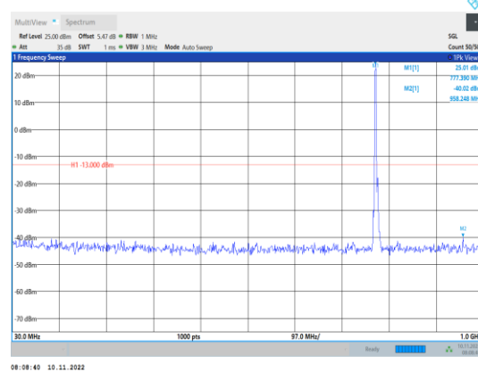
Band13-5MHz-16QAM-23205-1RB#0- Range1:30~1000MHz
