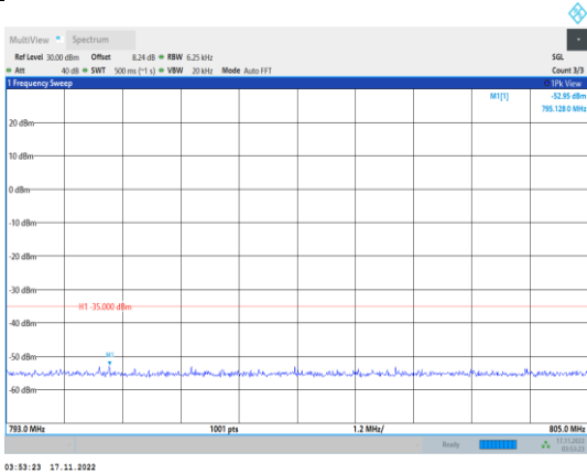
Band13-5MHz-64QAM-23205-1RB#0- Range4:793~805MHz
