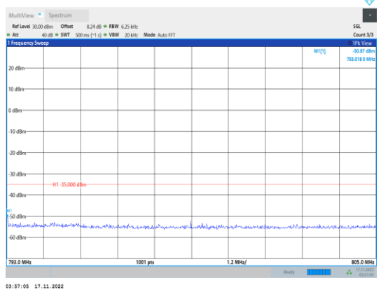
Band13-10MHz-64QAM-23230-1RB#0- Range4:793~805MHz
