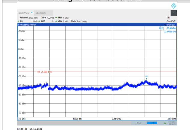
Band7-5MHz-64QAM-20775-1RB#0- Range3:3000~26500MHz
