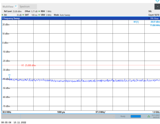
Band7-5MHz-16QAM-21100-1RB#0- Range1:30~1000MHz
