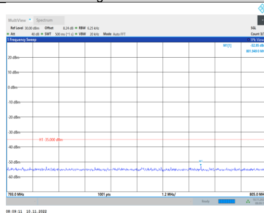
Band13-5MHz-16QAM-23205-1RB#0- Range4:793~805MHz
