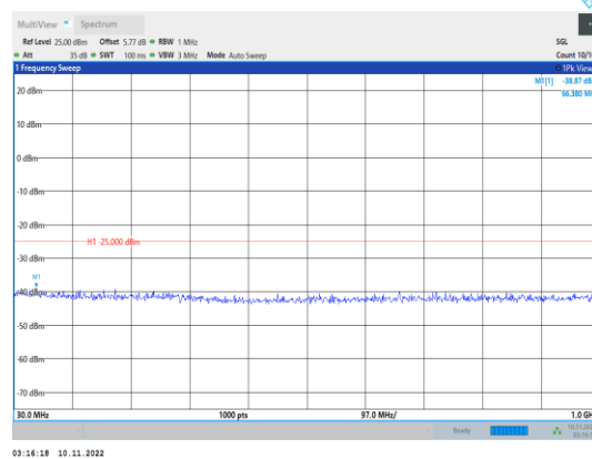
Band7-10MHz-QPSK-21400-1RB#0- Range1:30~1000MHz
