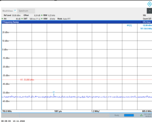
Band13-5MHz-QPSK-23205-1RB#0- Range4:793~805MHz
