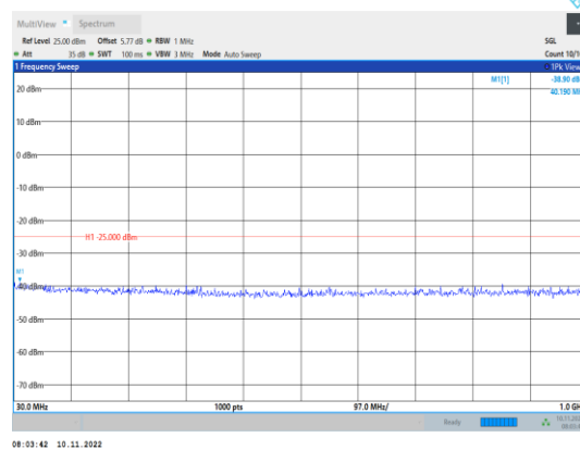
Band7-5MHz-16QAM-20775-1RB#0- Range1:30~1000MHz
