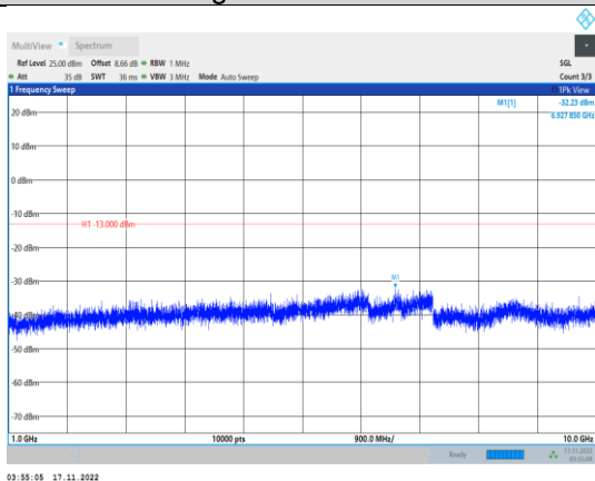
Band13-5MHz-64QAM-23255-1RB#0- Range2:1000~10000MHz
