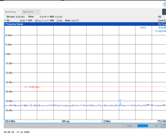
Band13-5MHz-64QAM-23255-1RB#0- Range3:763~775MHz
