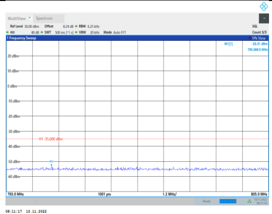
Band13-5MHz-16QAM-23230-1RB#0- Range4:793~805MHz
