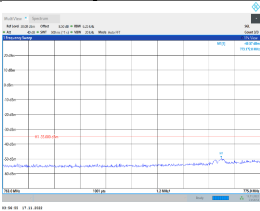
Band13-10MHz-64QAM-23230-1RB#0- Range3:763~775MHz
