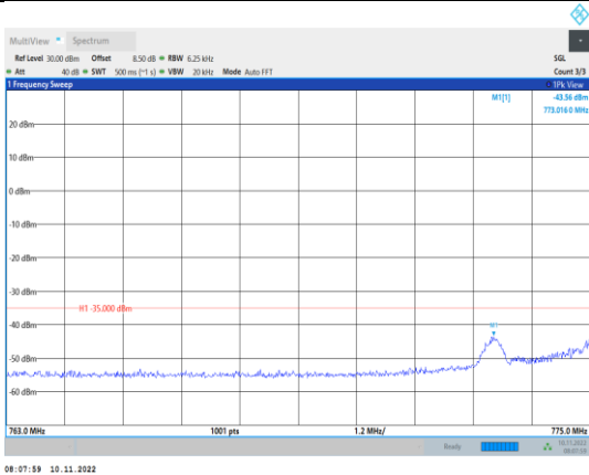
Band13-5MHz-QPSK-23205-1RB#0- Range3:763~775MHz
