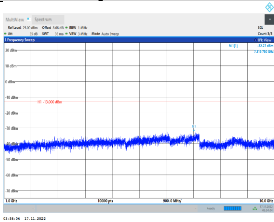
Band13-5MHz-64QAM-23230-1RB#0- Range2:1000~10000MHz
