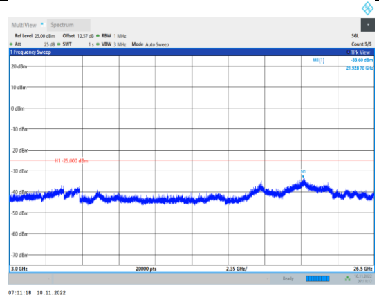
Band7-20MHz-16QAM-21350-1RB#0- Range3:3000~26500MHz
