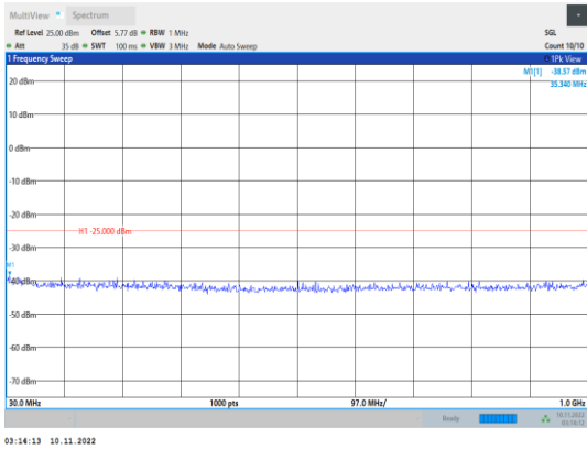
Band7-10MHz-16QAM-20800-1RB#0- Range1:30~1000MHz
