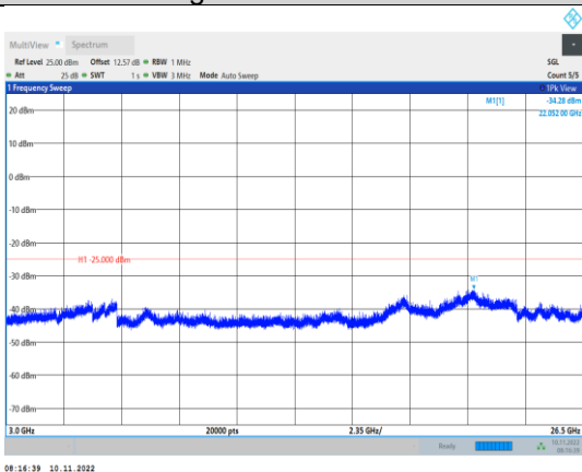
Band7-15MHz-QPSK-21100-1RB#0- Range3:3000~26500MHz
