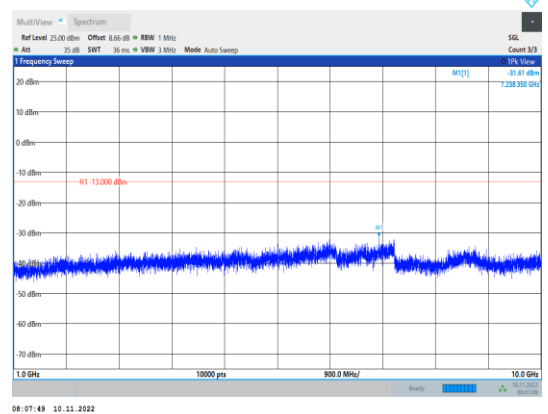
Band13-5MHz-QPSK-23205-1RB#0- Range2:1000~10000MHz
