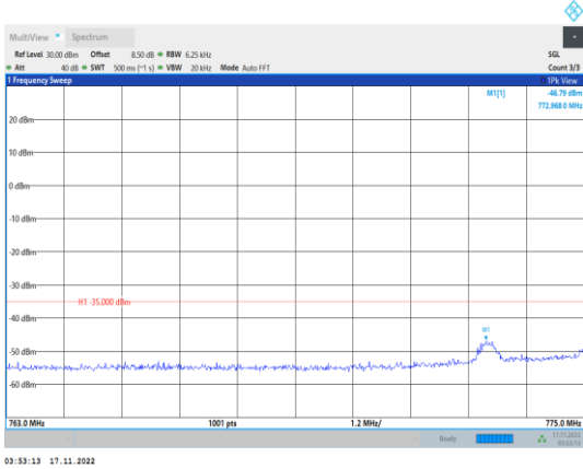
Band13-5MHz-64QAM-23205-1RB#0- Range3:763~775MHz
