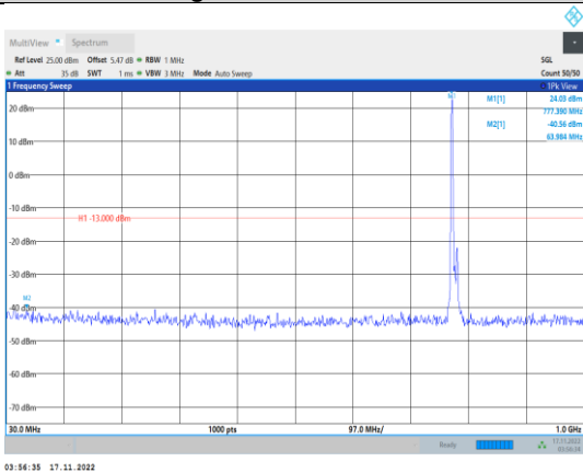
Band13-10MHz-64QAM-23230-1RB#0- Range1:30~1000MHz
