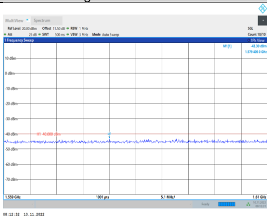
Band13-5MHz-QPSK-23255-1RB#0- Range5:1559~1610MHz
