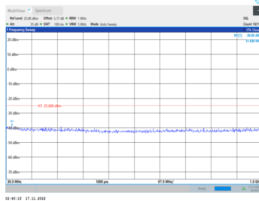
Band7-15MHz-64QAM-20825-1RB#0- Range1:30~1000MHz
