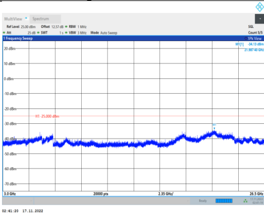
Band7-15MHz-64QAM-21100-1RB#0- Range3:3000~26500MHz
