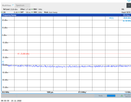
Band7-5MHz-QPSK-20775-1RB#0- Range1:30~1000MHz
