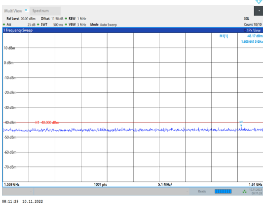
Band13-5MHz-16QAM-23230-1RB#0- Range5:1559~1610MHz
