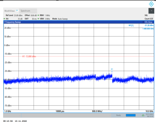
Band13-5MHz-16QAM-23230-1RB#0- Range2:1000~10000MHz
