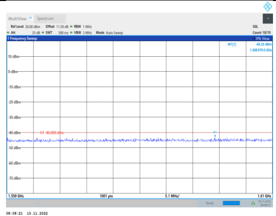
Band13-5MHz-QPSK-23205-1RB#0- Range5:1559~1610MHz
