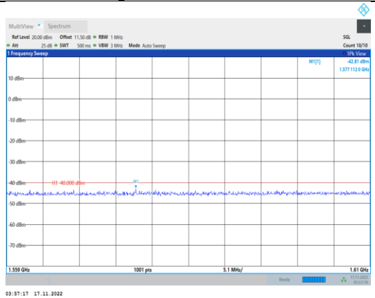
Band13-10MHz-64QAM-23230-1RB#0- Range5:1559~1610MHz
