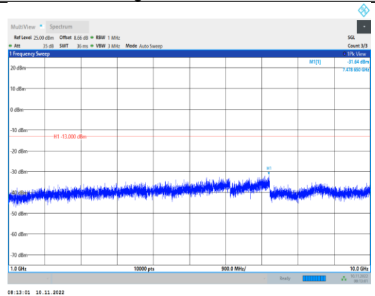
Band13-5MHz-16QAM-23255-1RB#0- Range2:1000~10000MHz
