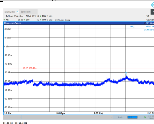
Band7-5MHz-16QAM-21425-1RB#0- Range3:3000~26500MHz
