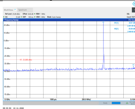
Band7-5MHz-16QAM-20775-1RB#0- Range2:1000~3000MHz
