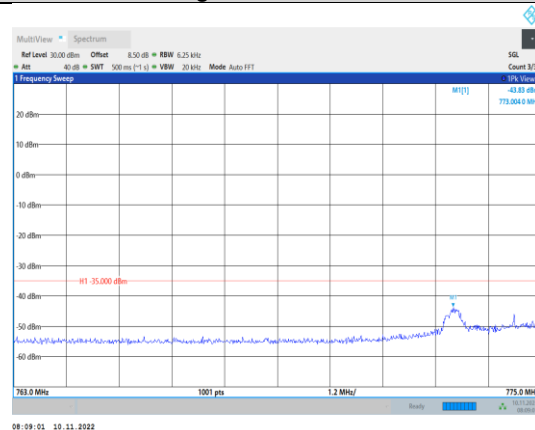
Band13-5MHz-16QAM-23205-1RB#0- Range3:763~775MHz
