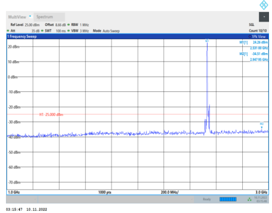
Band7-10MHz-16QAM-21100-1RB#0- Range2:1000~3000MHz
