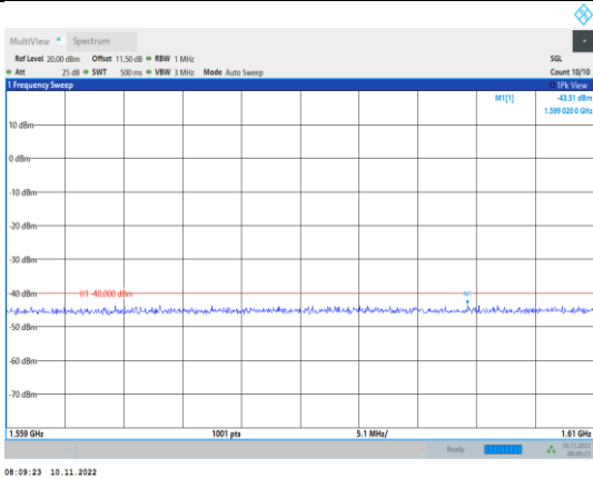
Band13-5MHz-16QAM-23205-1RB#0- Range5:1559~1610MHz
