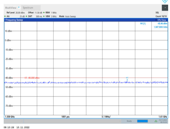
Band13-5MHz-QPSK-23230-1RB#0- Range5:1559~1610MHz
