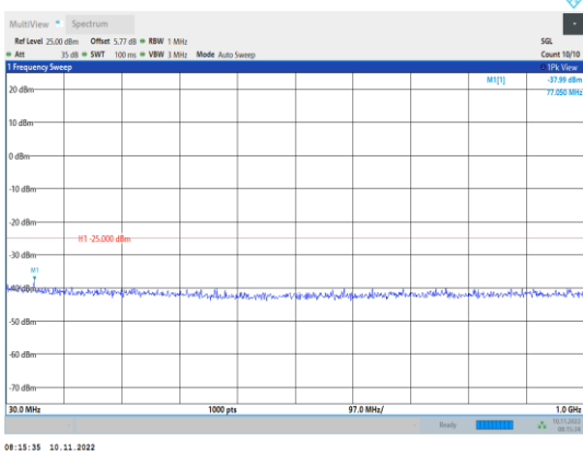
Band7-15MHz-16QAM-20825-1RB#0- Range1:30~1000MHz
