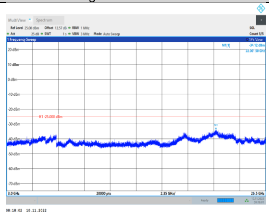
Band7-15MHz-QPSK-21375-1RB#0- Range3:3000~26500MHz
