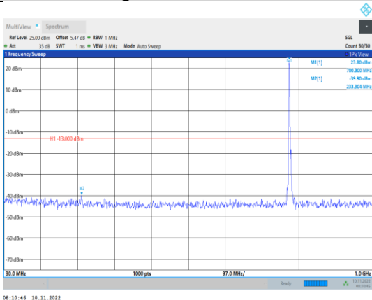
Band13-5MHz-16QAM-23230-1RB#0- Range1:30~1000MHz
