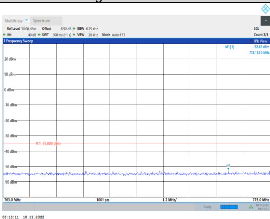
Band13-5MHz-16QAM-23255-1RB#0- Range3:763~775MHz
