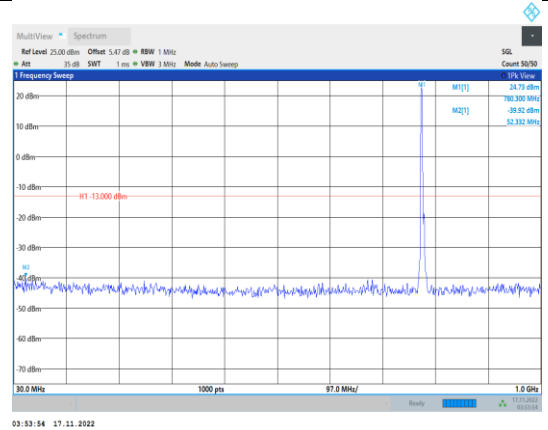
Band13-5MHz-64QAM-23230-1RB#0- Range1:30~1000MHz
