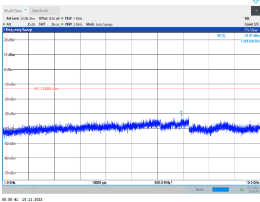
Band13-10MHz-QPSK-23230-1RB#0- Range2:1000~10000MHz
