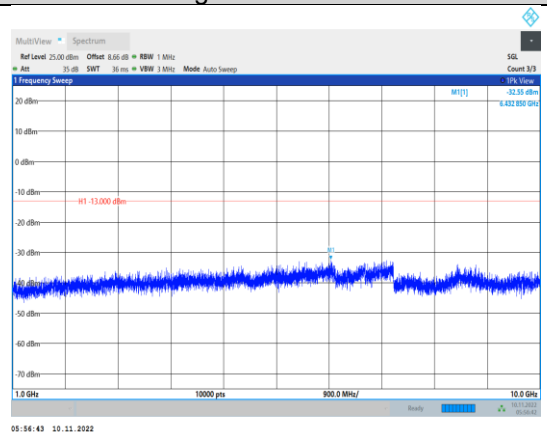
Band13-10MHz-16QAM-23230-1RB#0- Range2:1000~10000MHz
