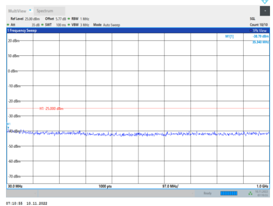
Band7-20MHz-16QAM-21350-1RB#0- Range1:30~1000MHz
