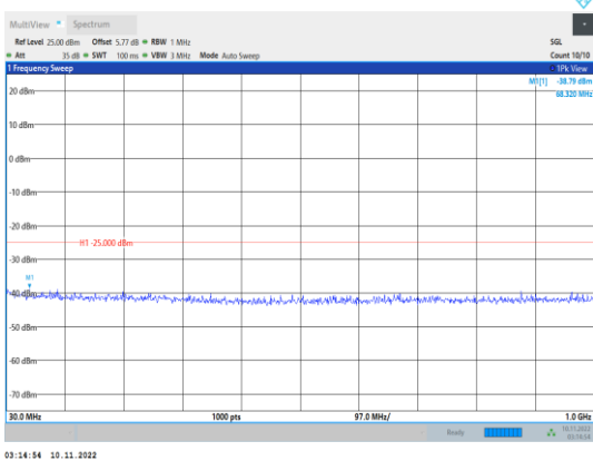
Band7-10MHz-QPSK-21100-1RB#0- Range1:30~1000MHz
