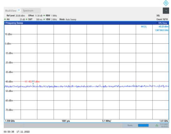
Band13-5MHz-64QAM-23205-1RB#0- Range5:1559~1610MHz
