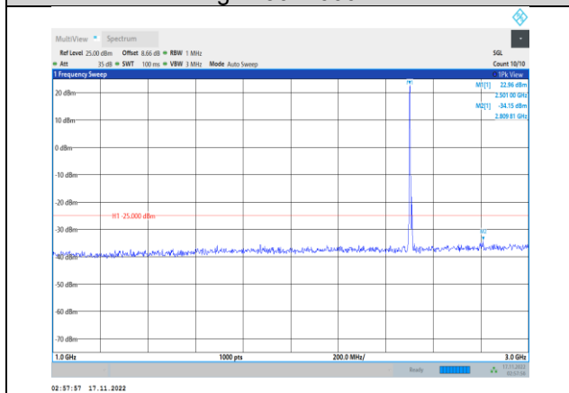
Band7-5MHz-64QAM-20775-1RB#0- Range2:1000~3000MHz
