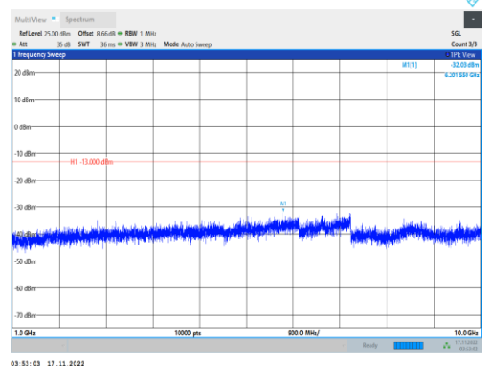
Band13-5MHz-64QAM-23205-1RB#0- Range2:1000~10000MHz
