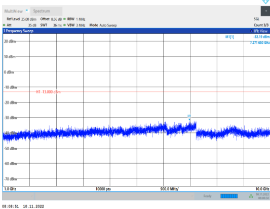
Band13-5MHz-16QAM-23205-1RB#0- Range2:1000~10000MHz
