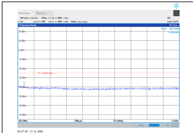
Band7-5MHz-64QAM-20775-1RB#0- Range1:30~1000MHz
