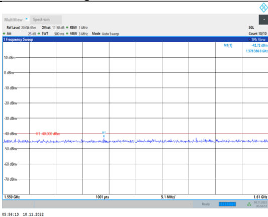
Band13-10MHz-QPSK-23230-1RB#0- Range5:1559~1610MHz
