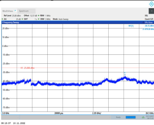
Band7-15MHz-16QAM-20825-1RB#0- Range3:3000~26500MHz
