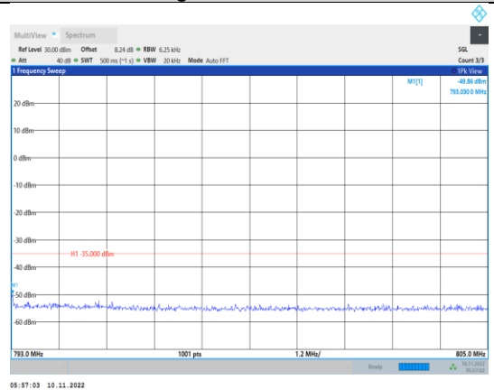
Band13-10MHz-16QAM-23230-1RB#0- Range4:793~805MHz
