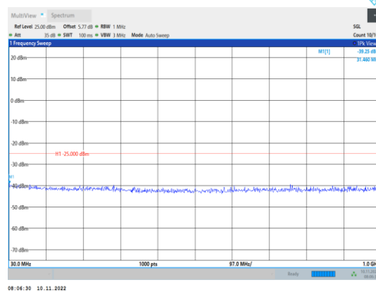
Band7-5MHz-16QAM-21425-1RB#0- Range1:30~1000MHz
