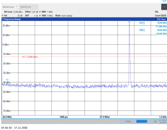
Band13-5MHz-64QAM-23205-1RB#0- Range1:30~1000MHz
