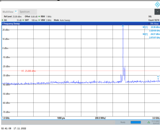
Band7-15MHz-64QAM-21100-1RB#0- Range2:1000~3000MHz
