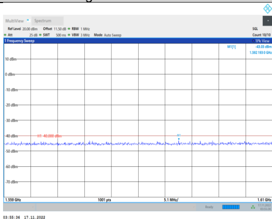
Band13-5MHz-64QAM-23255-1RB#0- Range5:1559~1610MHz
