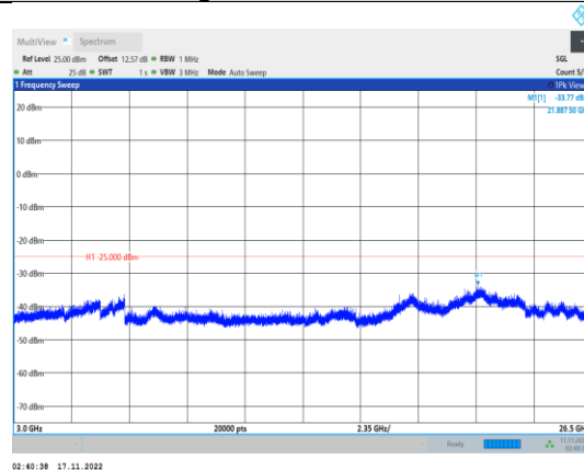
Band7-15MHz-64QAM-20825-1RB#0- Range3:3000~26500MHz
