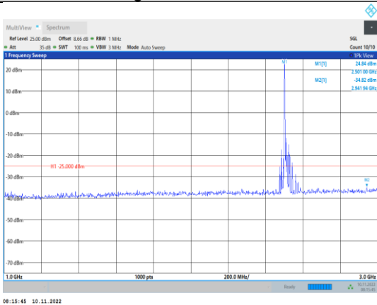
Band7-15MHz-16QAM-20825-1RB#0- Range2:1000~3000MHz
