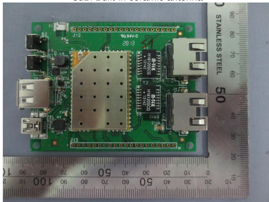
3dBi Built-in ceramic antenna
