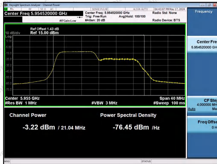
11AX20SISO-Ant1-5955-106Tone-RU53-PASS
