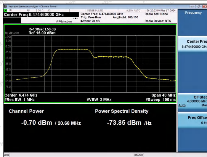
11AX20SISO-Ant1-6475-106Tone-RU53-PASS
