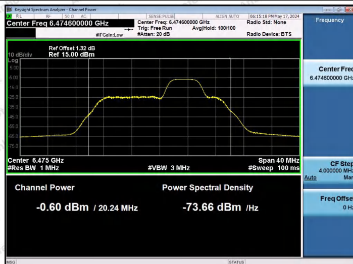
11AX20SISO-Ant1-6475-52Tone-RU39-PASS
