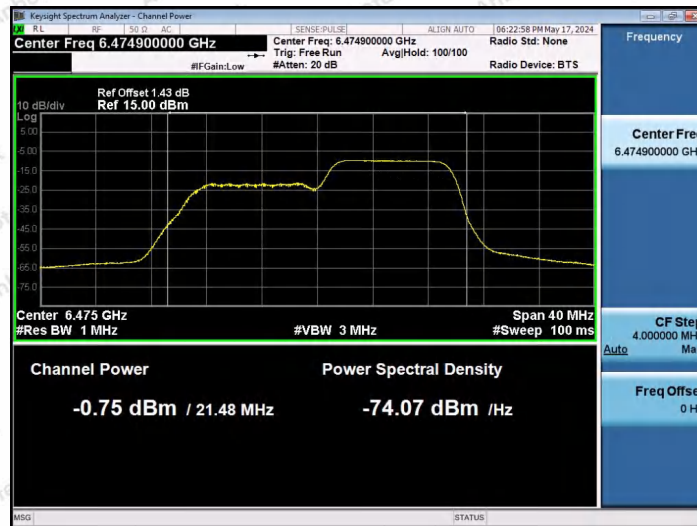
11AX20SISO-Ant1-6475-106Tone-RU54-PASS
