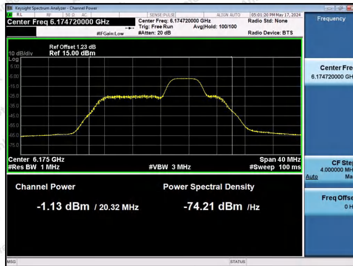
11AX20SISO-Ant1-6175-52Tone-RU39-PASS
