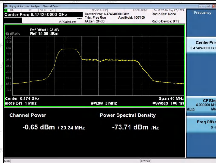
11AX20SISO-Ant1-6475-52Tone-RU37-PASS
