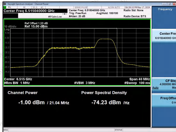
11AX20SISO-Ant1-6515-52Tone-RU40-PASS
