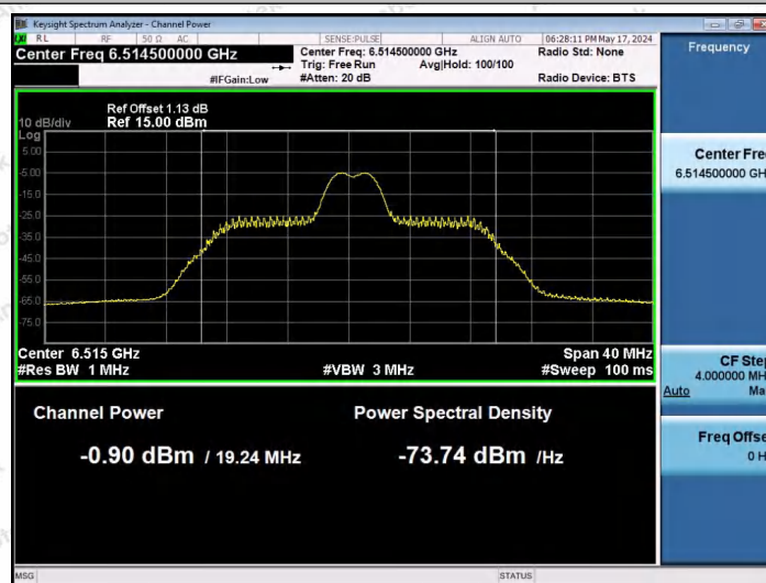
11AX20SISO-Ant1-6515-26Tone-RU4-PASS
