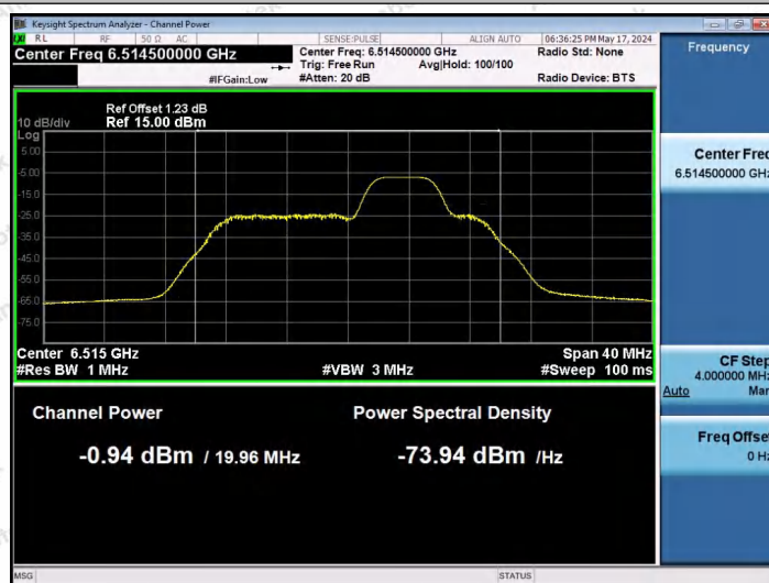
11AX20SISO-Ant1-6515-52Tone-RU39-PASS
