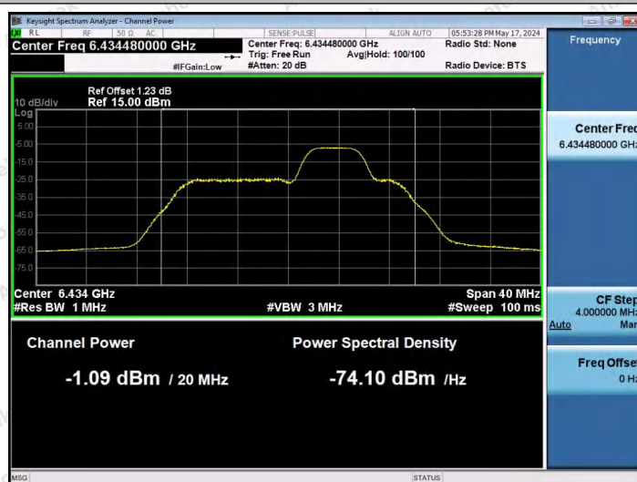
11AX20SISO-Ant1-6435-52Tone-RU39-PASS
