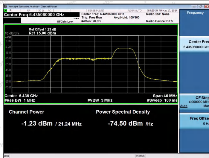
11AX20SISO-Ant1-6435-52Tone-RU40-PASS
