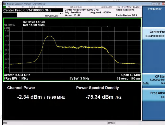
11AX20SISO-Ant1-6535-26Tone-RU0-PASS
