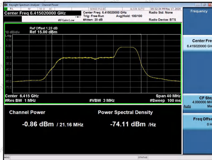
11AX20SISO-Ant1-6415-52Tone-RU40-PASS
