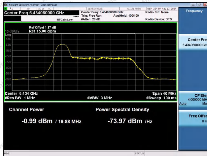
11AX20SISO-Ant1-6435-26Tone-RU0-PASS
