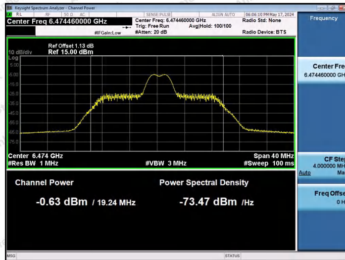
11AX20SISO-Ant1-6475-26Tone-RU4-PASS
