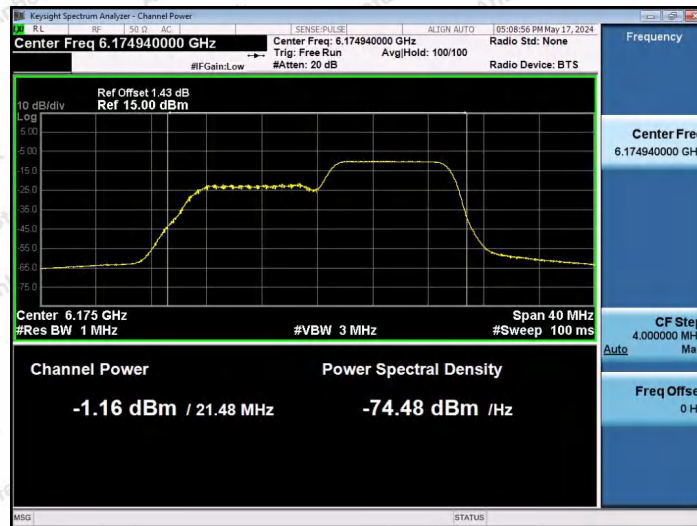
11AX20SISO-Ant1-6175-106Tone-RU54-PASS
