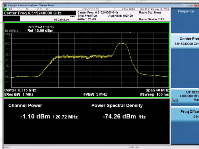
11AX20SISO-Ant1-6515-26Tone-RU8-PASS
