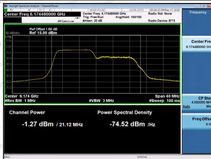
11AX20SISO-Ant1-6175-106Tone-RU53-PASS
