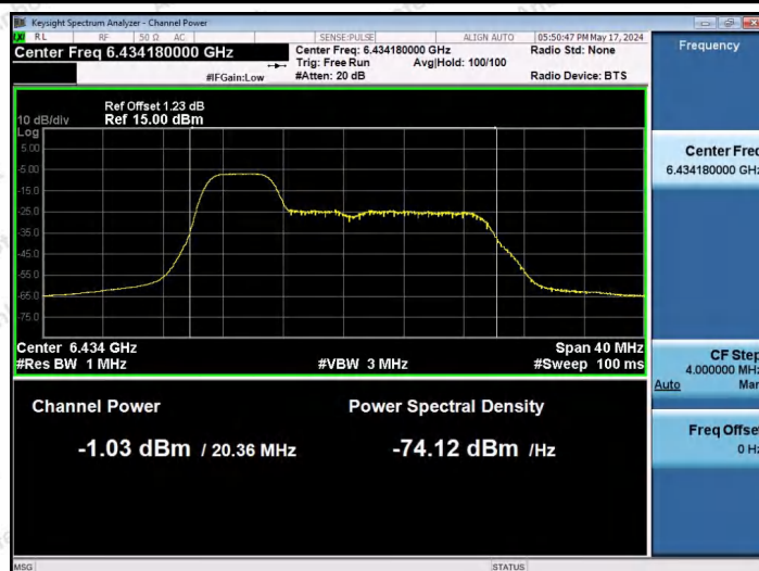
11AX20SISO-Ant1-6435-52Tone-RU37-PASS
