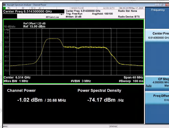
11AX20SISO-Ant1-6515-52Tone-RU37-PASS
