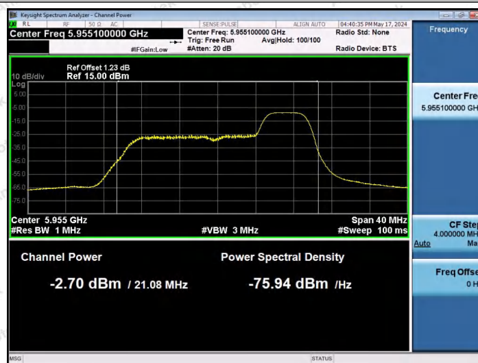
11AX20SISO-Ant1-5955-52Tone-RU40-PASS
