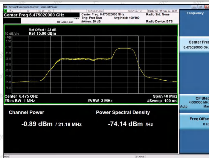
11AX20SISO-Ant1-6475-52Tone-RU40-PASS
