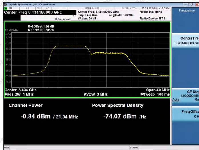
11AX20SISO-Ant1-6435-106Tone-RU53-PASS
