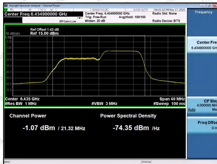
11AX20SISO-Ant1-6435-106Tone-RU54-PASS
