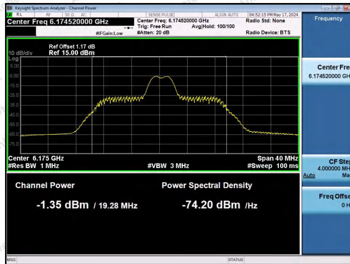
11AX20SISO-Ant1-6175-26Tone-RU4-PASS
