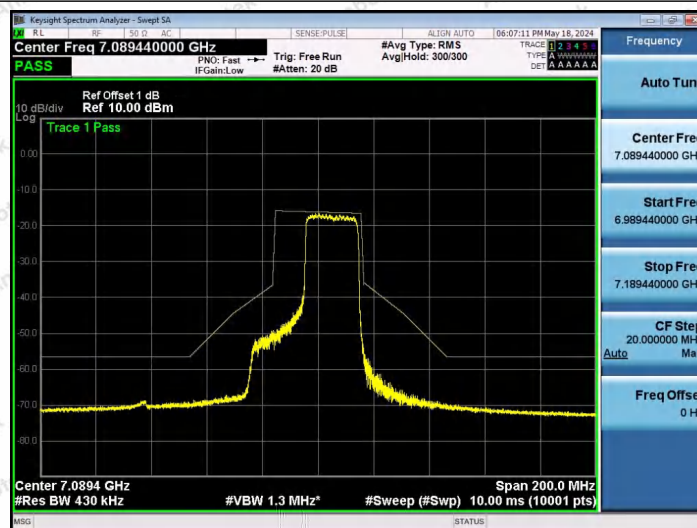
NTNV-11AX40SISO-Ant1-7085-242Tone-RU62-PASS
