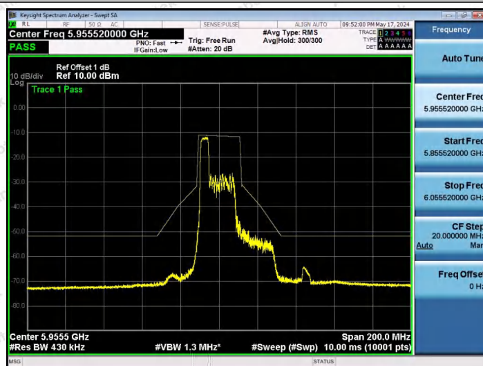
NTNV-11AX40SISO-Ant1-5965-52Tone-RU37-PASS
