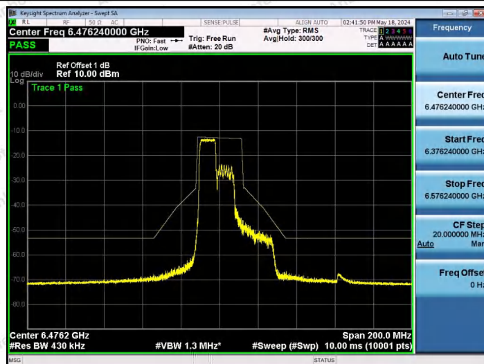
NTNV-11AX40SISO-Ant1-6485-106Tone-RU53-PASS
