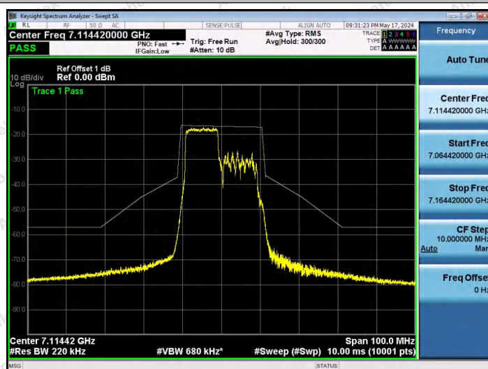
NTNV-11AX20SISO-Ant1-7115-106Tone-RU53-PASS
