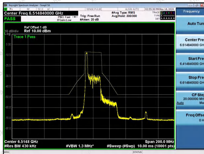
NTNV-11AX40SISO-Ant1-6525-26Tone-RU0-PASS
