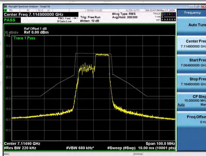
NTNV-11AX20SISO-Ant1-7115-106Tone-RU54-PASS
