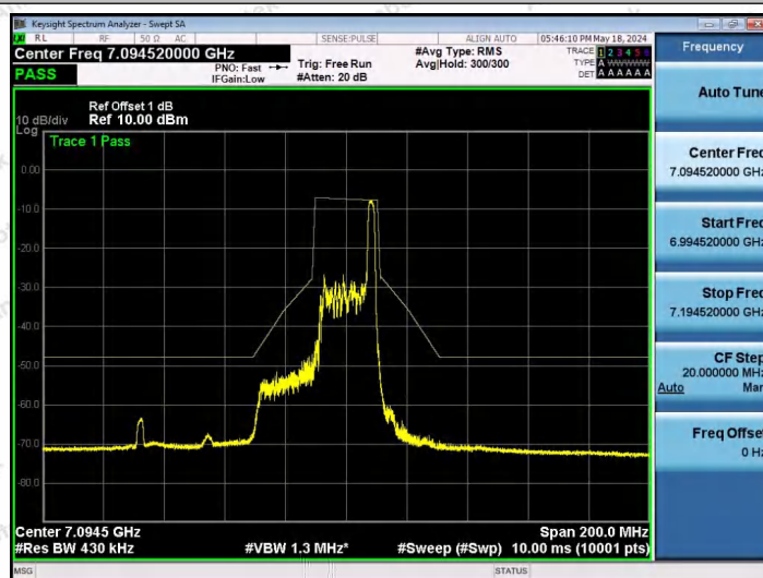
NTNV-11AX40SISO-Ant1-7085-26Tone-RU17-PASS
