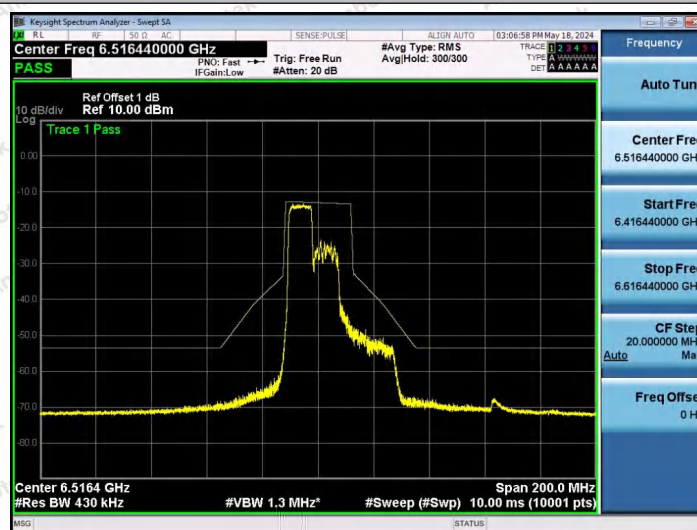
NTNV-11AX40SISO-Ant1-6525-106Tone-RU53-PASS
