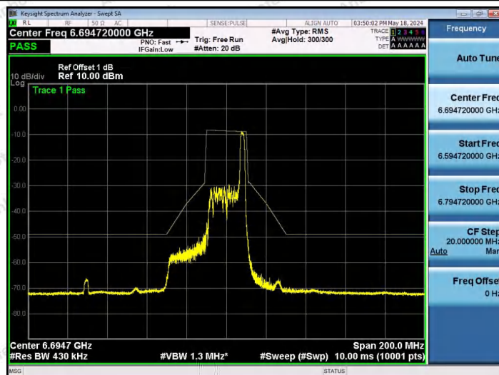
NTNV-11AX40SISO-Ant1-6685-26Tone-RU17-PASS
