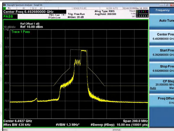
NTNV-11AX40SISO-Ant1-6485-106Tone-RU56-PASS
