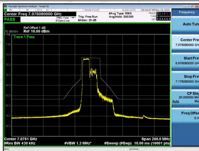
NTNV-11AX40SISO-Ant1-7085-106Tone-RU53-PASS
