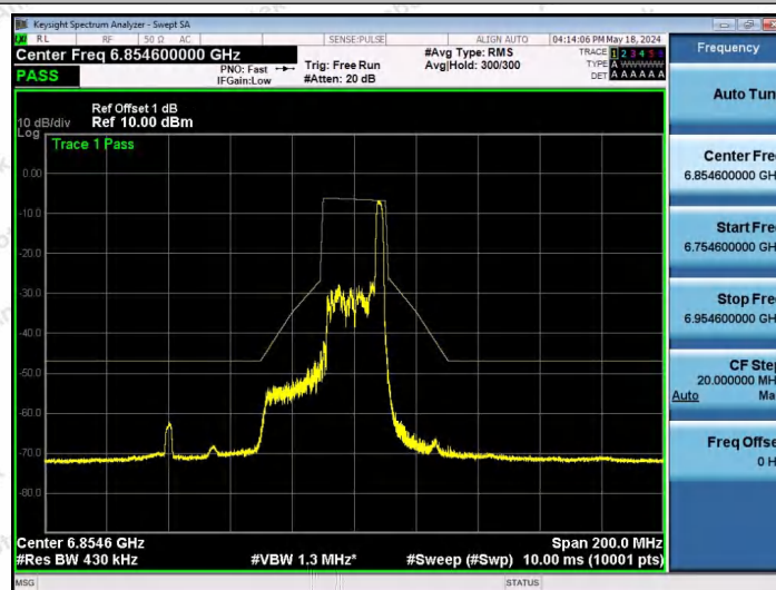
NTNV-11AX40SISO-Ant1-6845-26Tone-RU17-PASS
