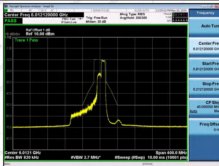
NTNV-11AX80SISO-Ant1-5985-106Tone-RU60-PASS
