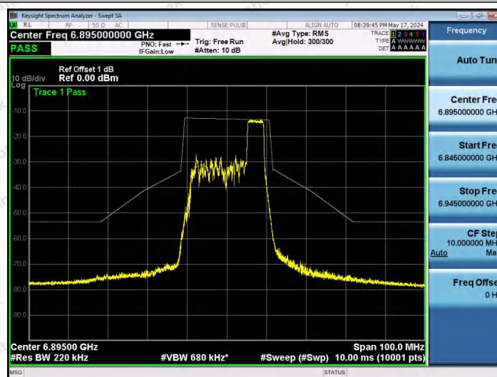
NTNV-11AX20SISO-Ant1-6895-52Tone-RU40-PASS
