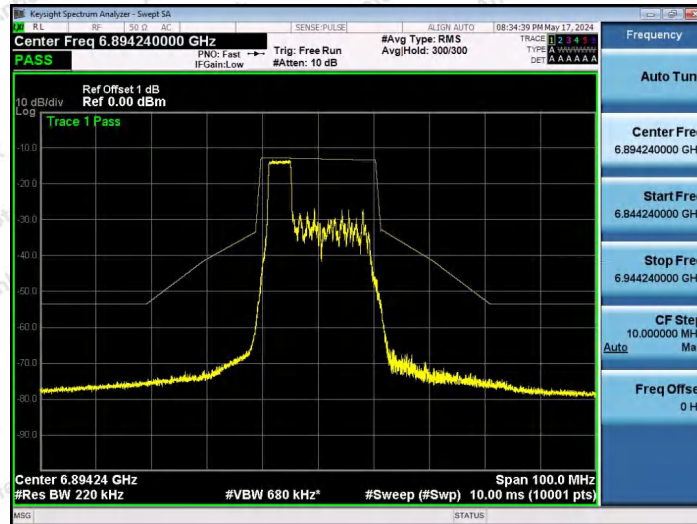
NTNV-11AX20SISO-Ant1-6895-52Tone-RU37-PASS
