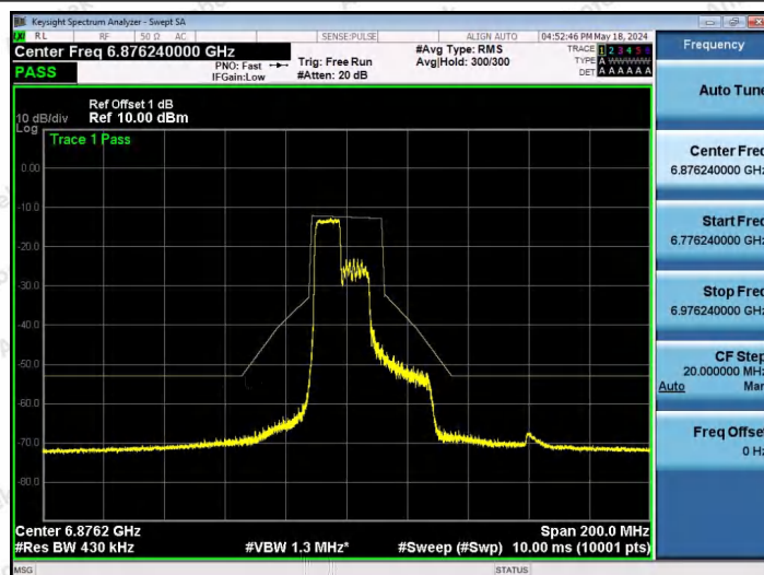
NTNV-11AX40SISO-Ant1-6885-106Tone-RU53-PASS
