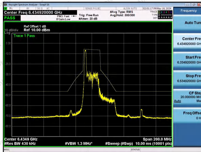
NTNV-11AX40SISO-Ant1-6445-26Tone-RU0-PASS
