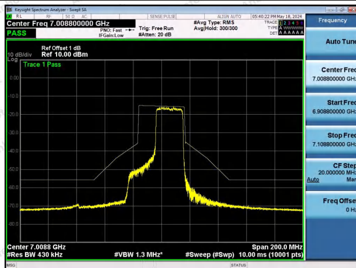
NTNV-11AX40SISO-Ant1-7005-242Tone-RU62-PASS
