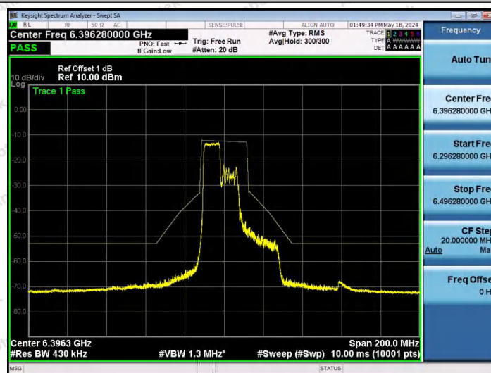
NTNV-11AX40SISO-Ant1-6405-106Tone-RU53-PASS
