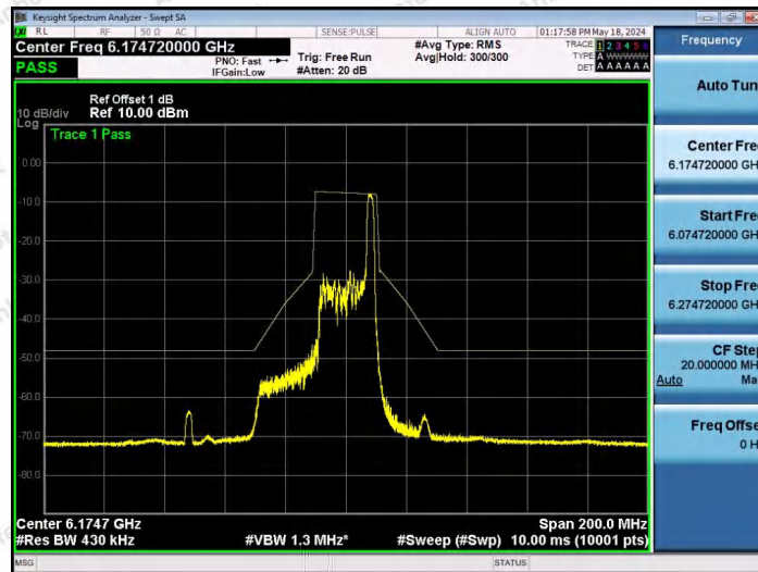
NTNV-11AX40SISO-Ant1-6165-26Tone-RU17-PASS
