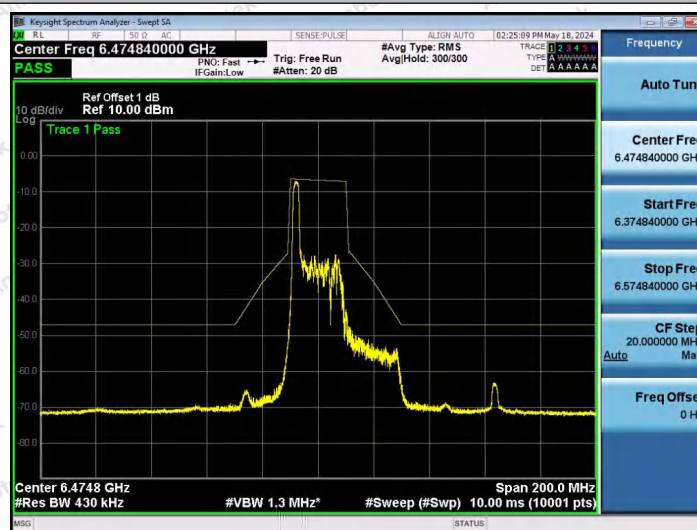
NTNV-11AX40SISO-Ant1-6485-26Tone-RU0-PASS
