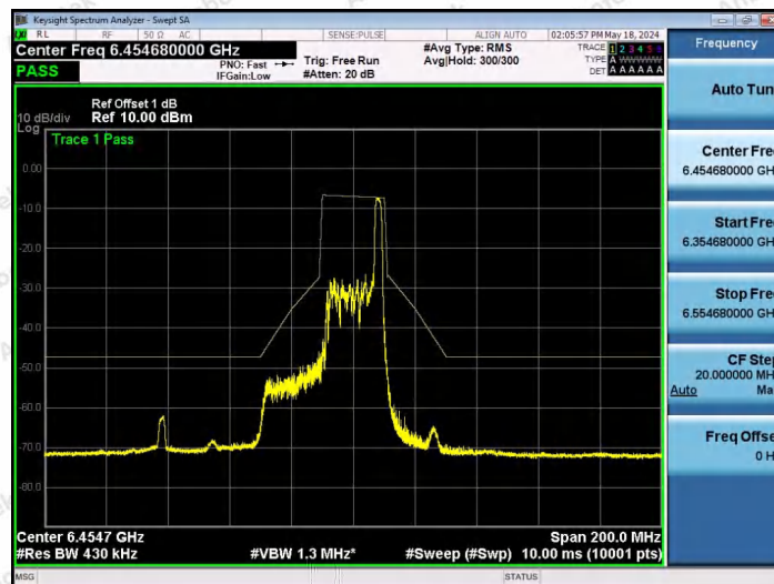
NTNV-11AX40SISO-Ant1-6445-26Tone-RU17-PASS
