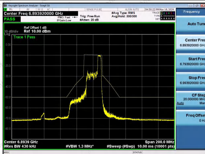
NTNV-11AX40SISO-Ant1-6885-52Tone-RU44-PASS
