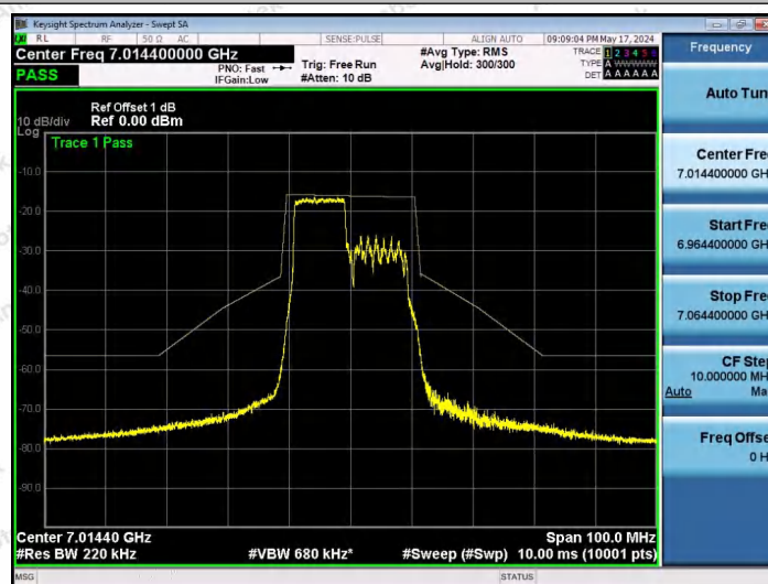
NTNV-11AX20SISO-Ant1-7015-106Tone-RU53-PASS
