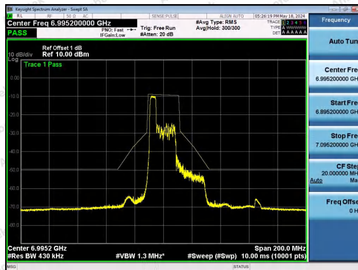
NTNV-11AX40SISO-Ant1-7005-52Tone-RU37-PASS
