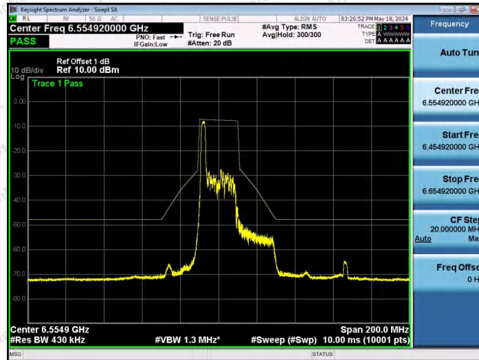
NTNV-11AX40SISO-Ant1-6565-26Tone-RU0-PASS
