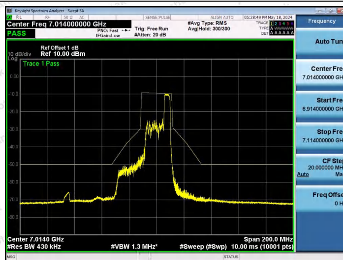
NTNV-11AX40SISO-Ant1-7005-52Tone-RU44-PASS
