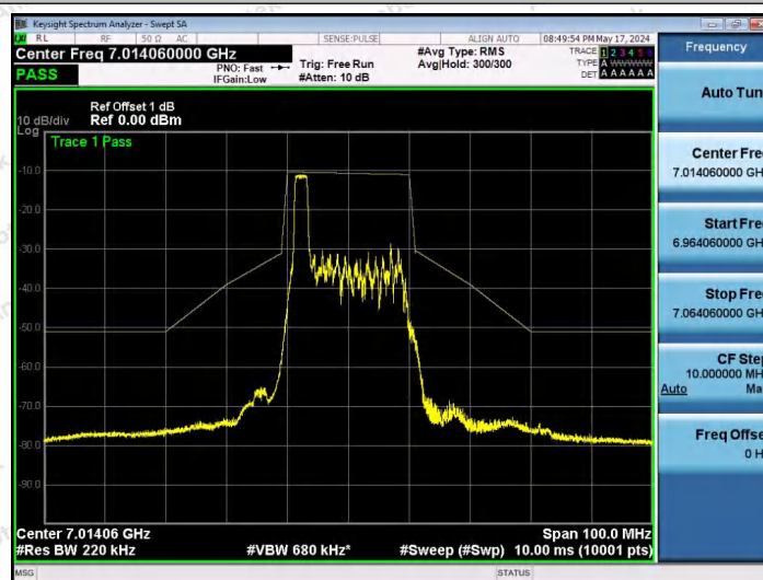
NTNV-11AX20SISO-Ant1-7015-26Tone-RU0-PASS
