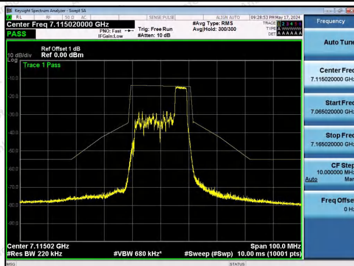
NTNV-11AX20SISO-Ant1-7115-52Tone-RU40-PASS
