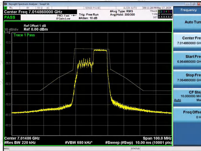
NTNV-11AX20SISO-Ant1-7015-106Tone-RU54-PASS
