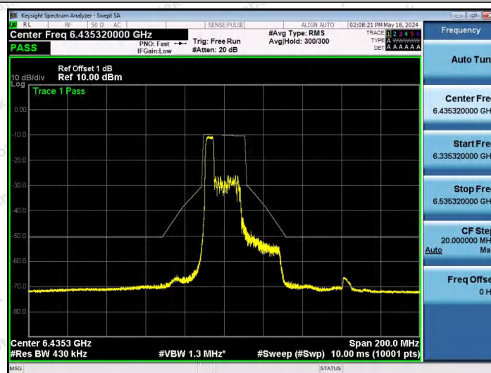
NTNV-11AX40SISO-Ant1-6445-52Tone-RU37-PASS
