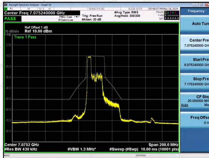
NTNV-11AX40SISO-Ant1-7085-52Tone-RU37-PASS
