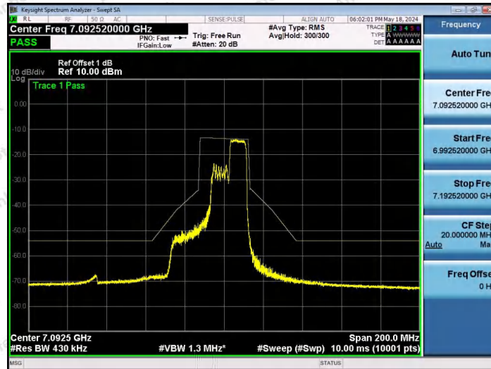
NTNV-11AX40SISO-Ant1-7085-106Tone-RU56-PASS
