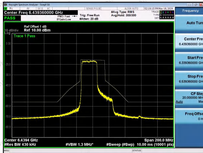
NTNV-11AX40SISO-Ant1-6445-242Tone-RU61-PASS
