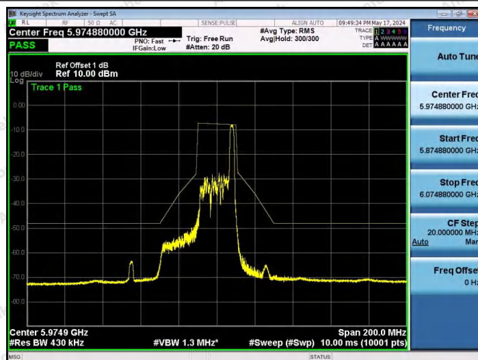
NTNV-11AX40SISO-Ant1-5965-26Tone-RU17-PASS
