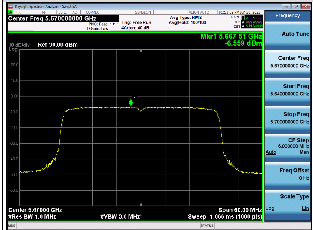
Test_Graph_802.11ax40_ANT2_5670_MCS9_PSD
