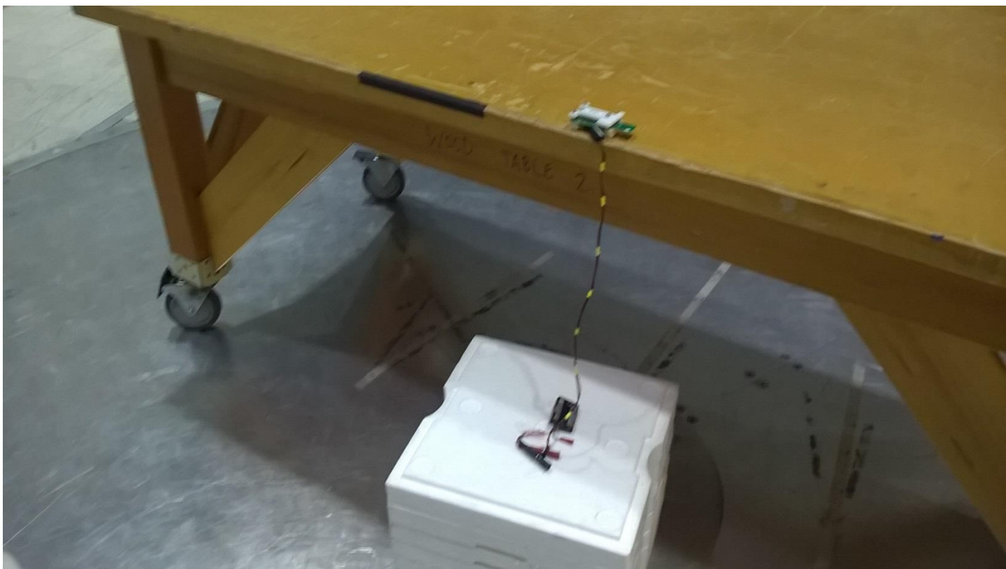
Figure 3 – Radiated Emissions Test Setup, 30MHz – 1GHz
