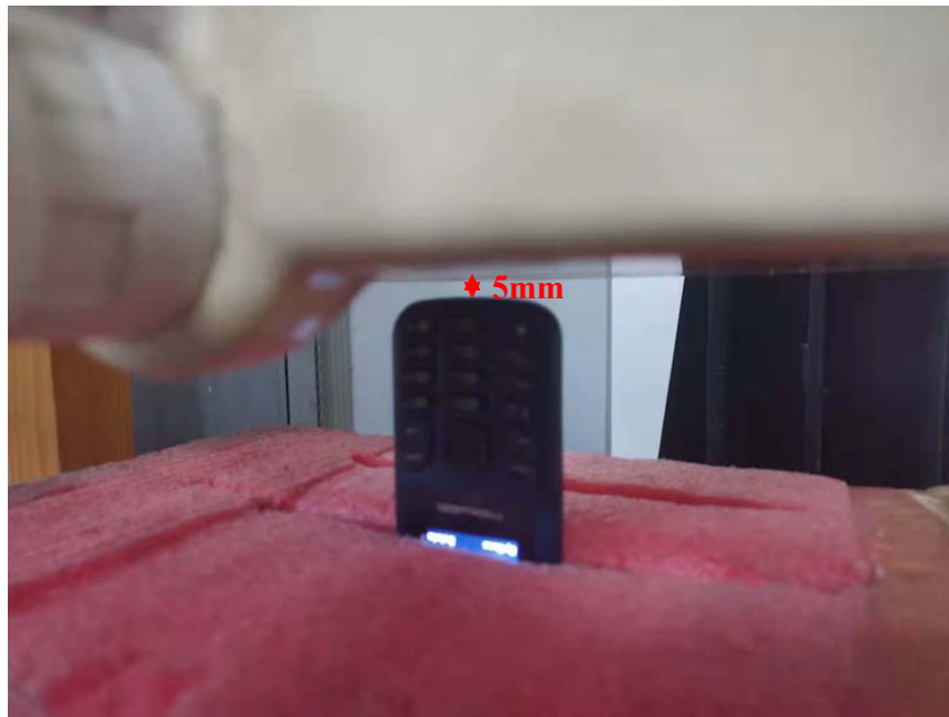
Body Bottom Setup Photo (5mm)
