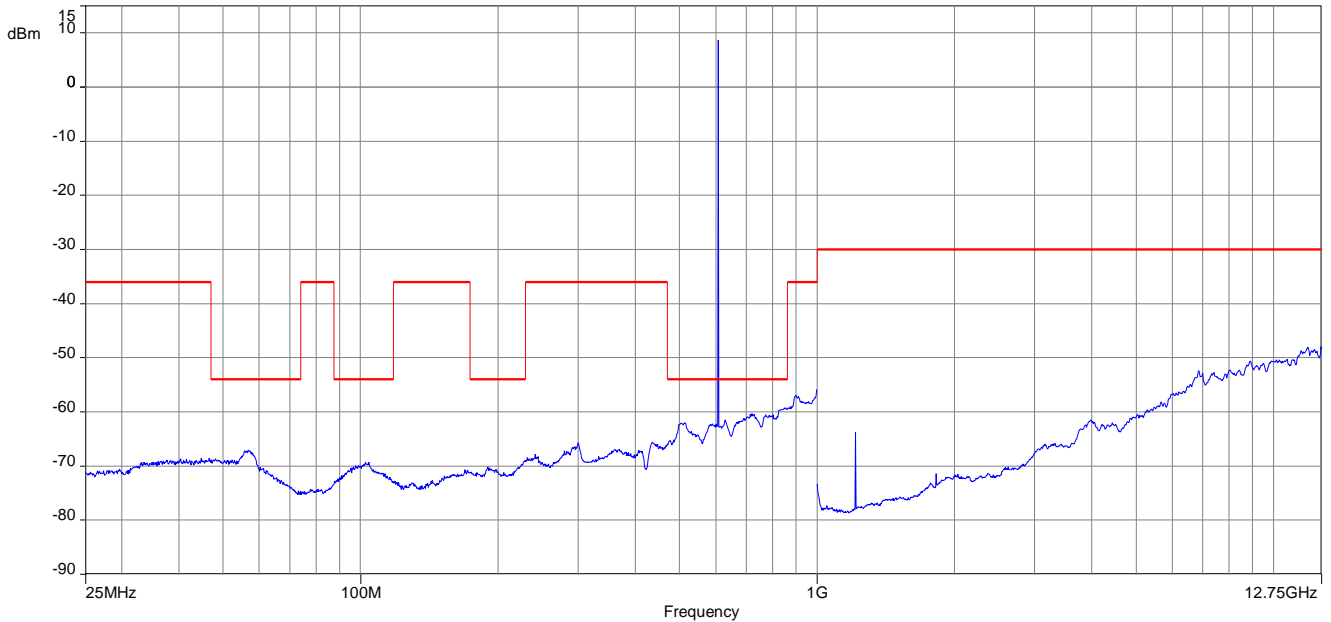
Plots: Spectrum mask, Band A+
