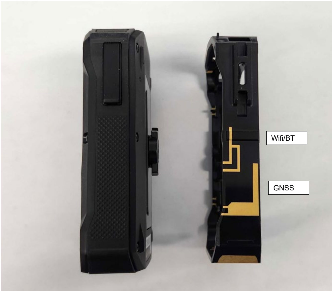
Antenna Left (Wifi/BT and GNSS)
