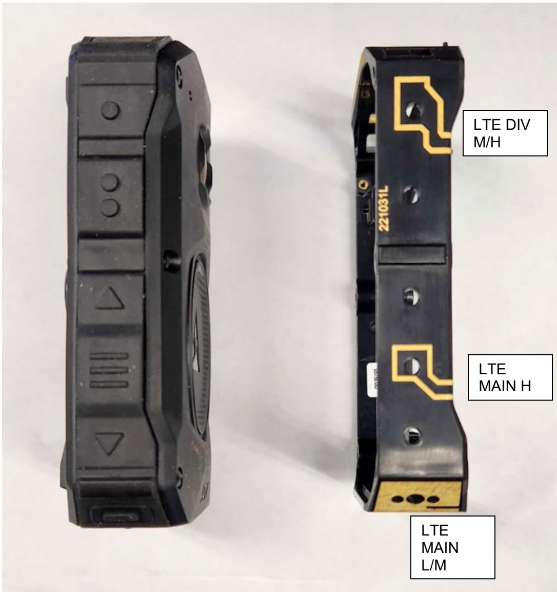
Antenna Right (LTE Main L/B, LTE Main H, LTE Div M/H)
