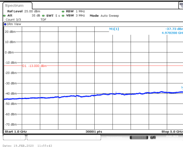
Band5_Stand-Alone_NaN_BPSK_20649_1@0_15kHz_1000_5000_1000~5000MHz@-37.73dBm_-13_PASS__
