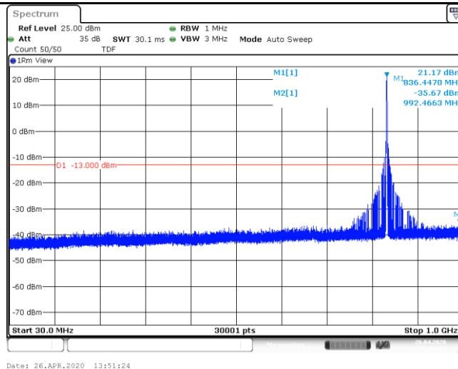
Band5_Stand-Alone_NaN_QPSK_20525_1@0_3.75kHz_30_1000_30-1000MHz@-35.67dBm_-13_PASS__
