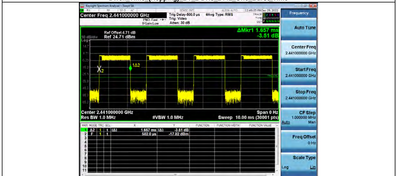
Dwell Time (Hopping) BT 2-DH1_2441_One_Burst_Time
