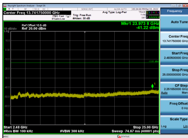
,Plot 4,2483.5MHz~25000MHz-802.11g
