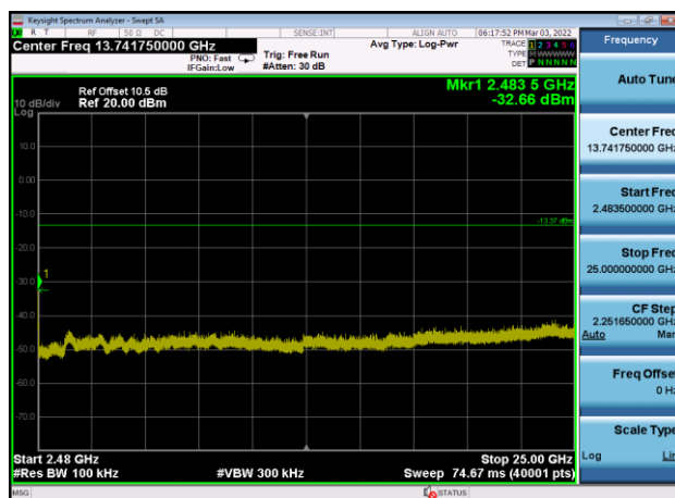
,Plot 4,2483.5MHz~25000MHz-802.11g
