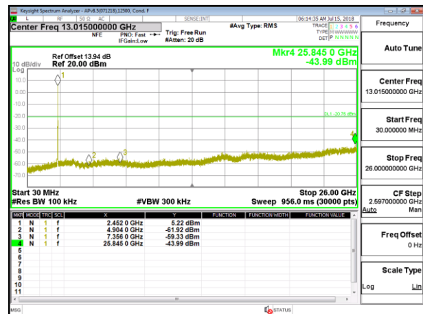
OUT-OF-BAND HIGH CHANNEL 9 ANTENNA 2
