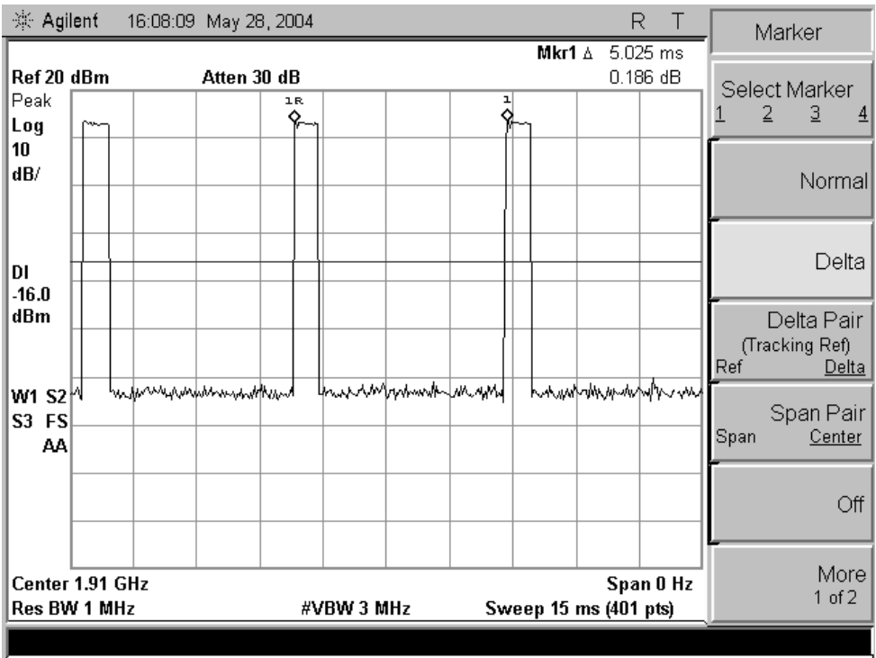
figure 1 (Modulation Characteristics)
