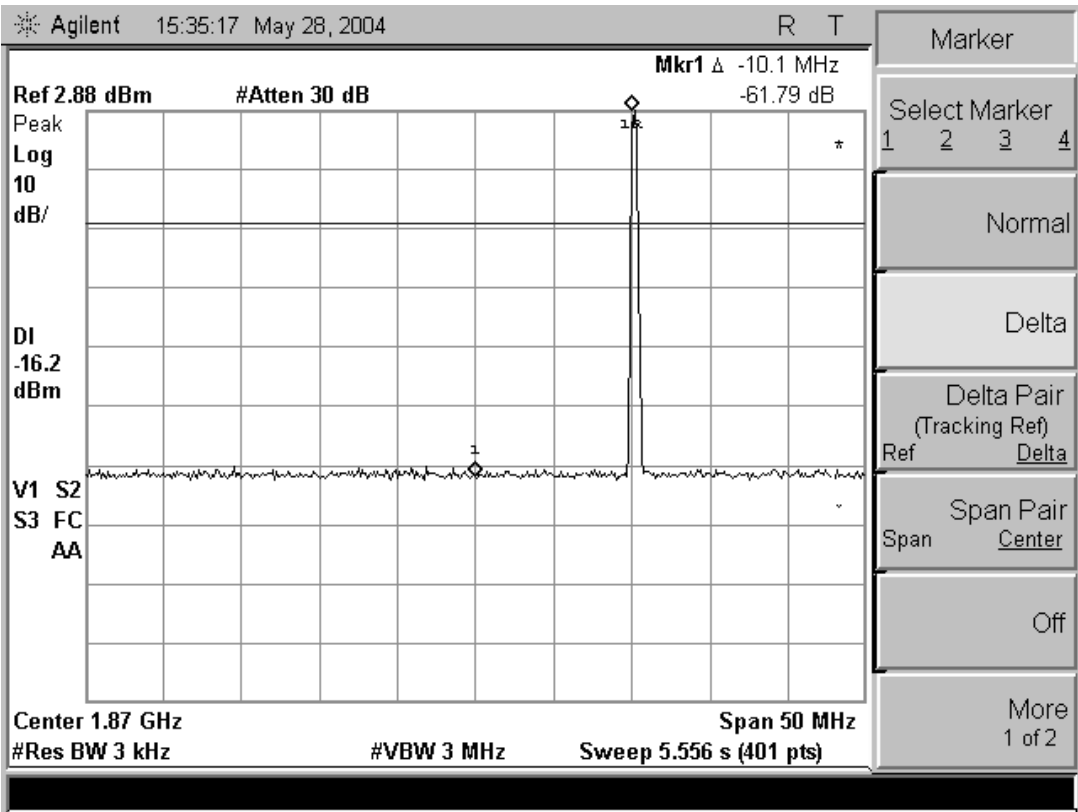
figure 6 Band Edge Low frequency side
