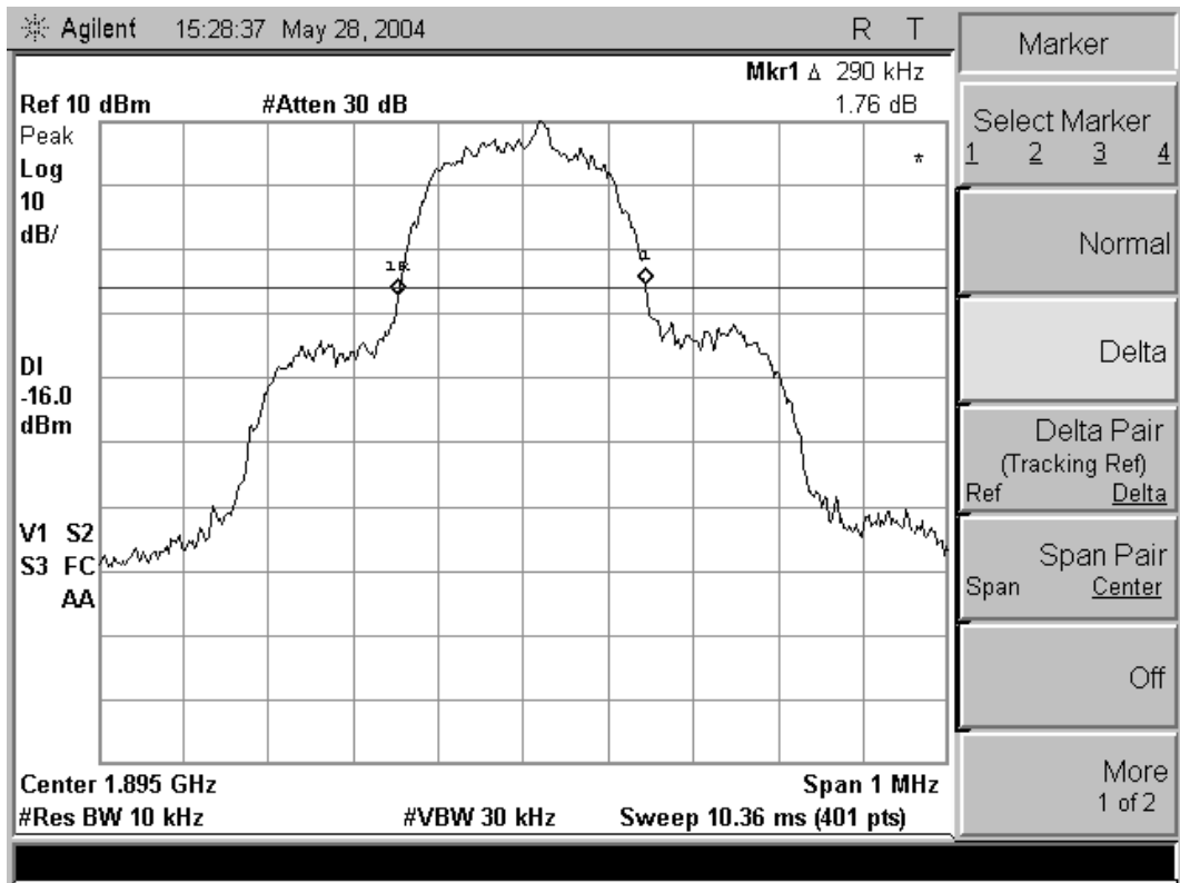
figure 4 26dB Bandwidth f_c = 1894.85 MHz
