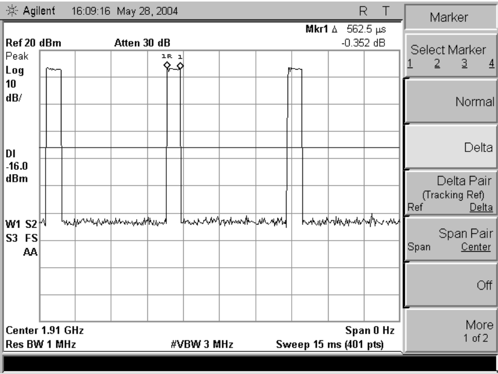
figure 2 (Modulation Characteristics)
