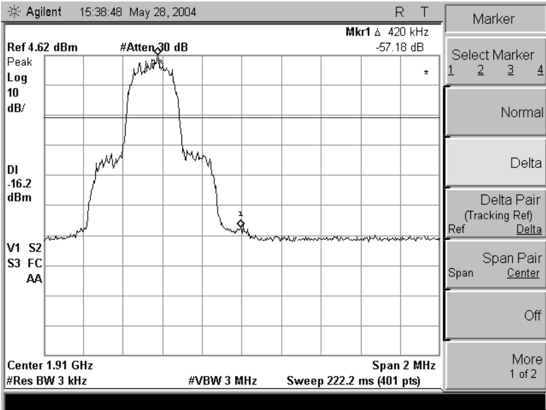
figure 7 Band Edge High frequency side
