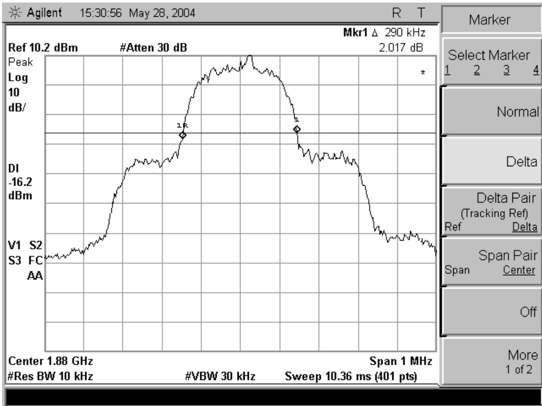
figure 3 26dB Bandwidth f_c = 1880.15 MHz
