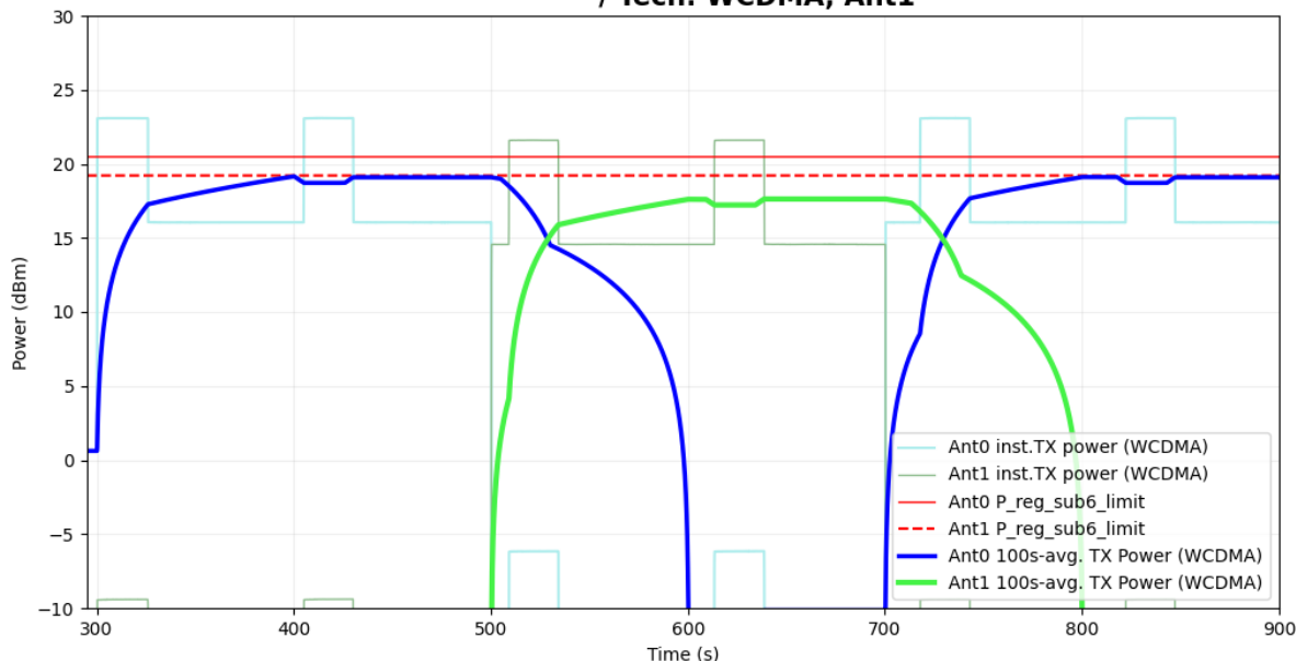
Figure 5- 48 Time-averaged conducted TX power over time for case 20 (WCDMA B2)
