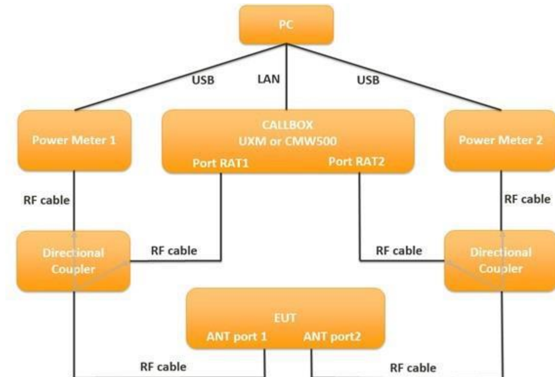
Figure 5- 5 TA-SAR conductive power test setup block diagram for scenarios 4/8
