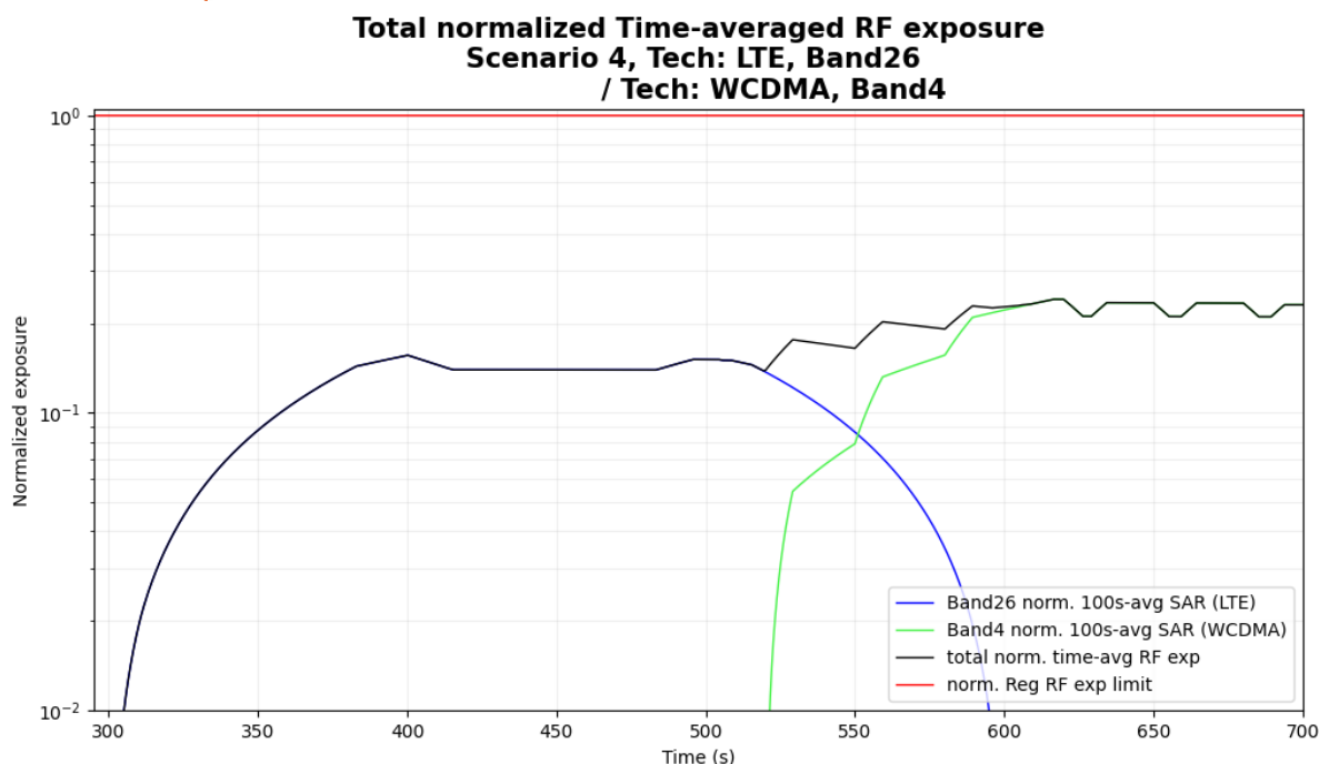
Figure 5- 45 Normalized time-averaged SAR for case 18 (LTE B26, WCDMA B4)
