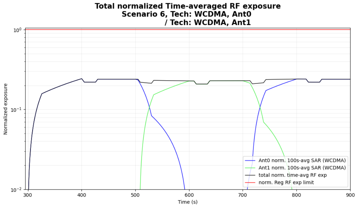
Figure 5- 49 Normalized time-averaged SAR for case 20 (WCDMA B2)
