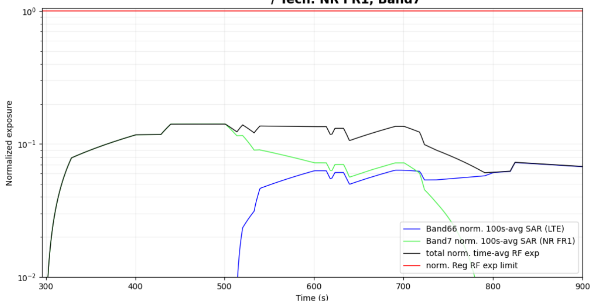
Figure 5- 55 Normalized time-averaged SAR for case 21 (LTE B66, sub6 NR n7)
