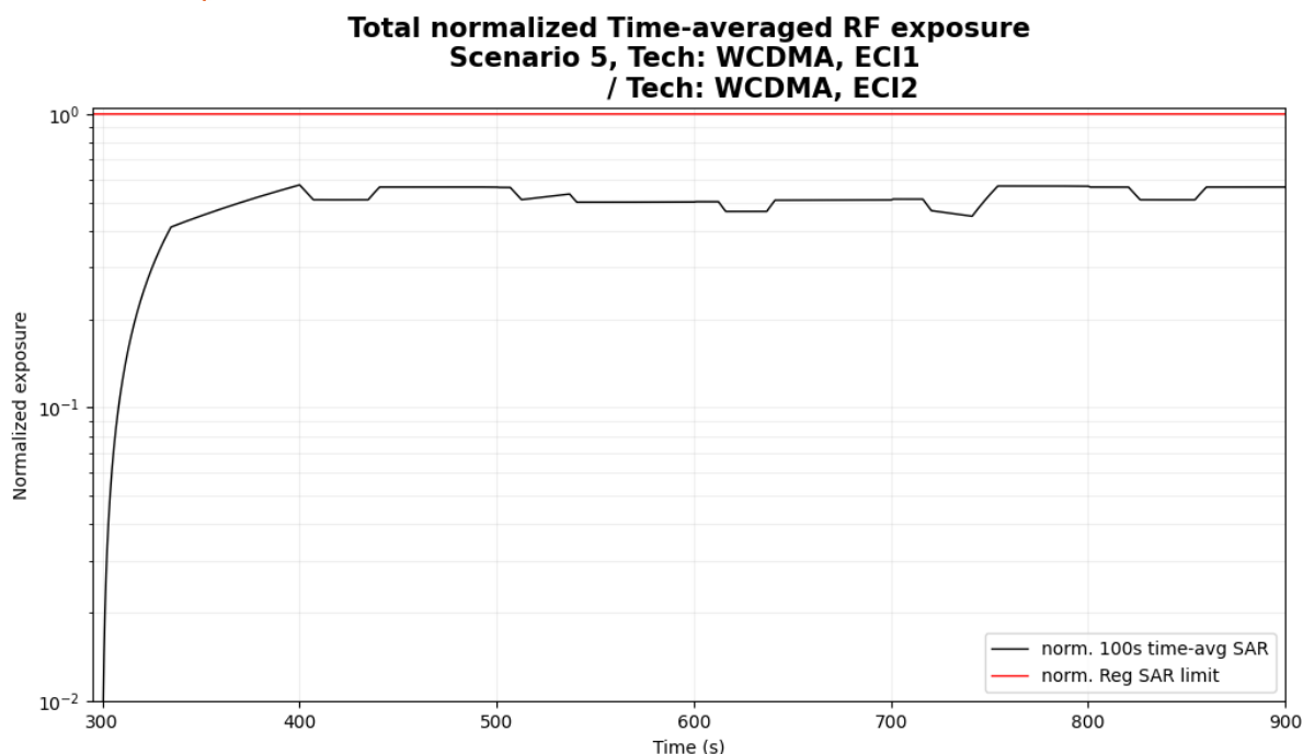
Figure 5- 47 Normalized time-averaged SAR for case 19 (WCDMA B2)
