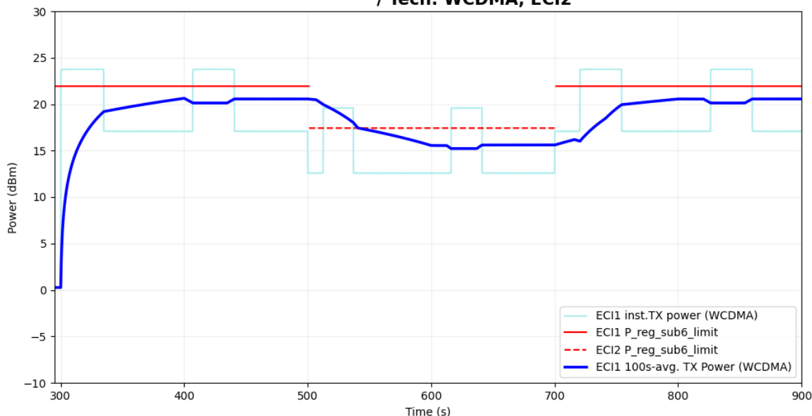
Figure 5- 46 Time-averaged conducted TX power over time for case 19 (WCDMA B2)
