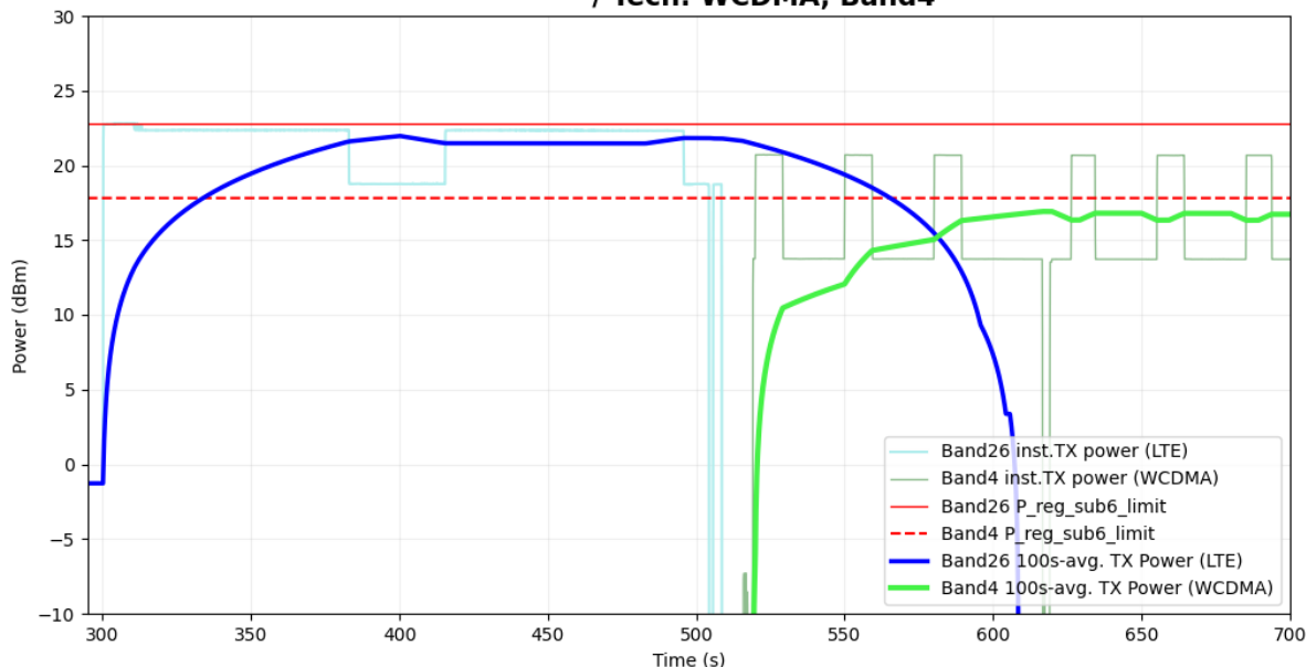
Figure 5- 44 Time-averaged conducted TX power over time for case 18 (LTE B26, WCDMA B4)
