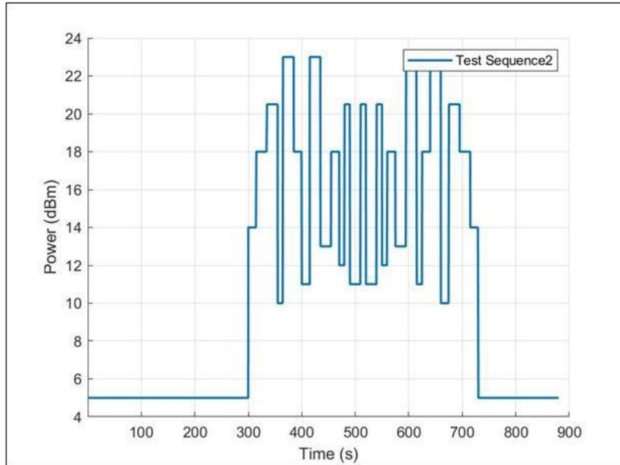
Figure 4-3 Test sequence 2
