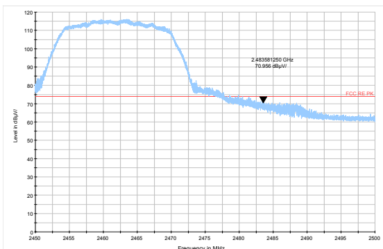
802.11g-Channel 11 Peak
