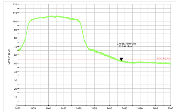
802.11g-Channel 11 Average
