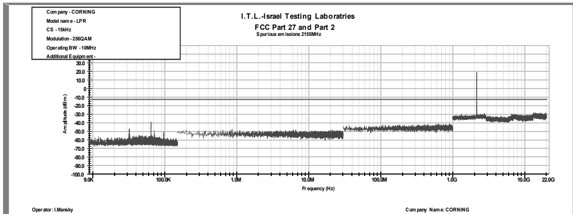
Figure 376: Spurious Emissions at Antenna Terminal 256QAM, 2155.0MHz, B.W. 10MHz, Sub Carrier 15 kHz
