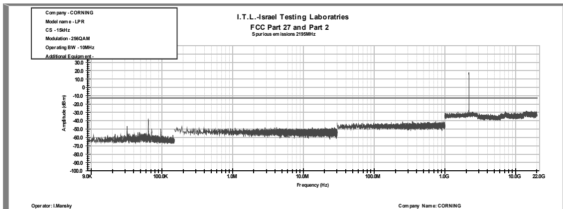
Figure 377: Spurious Emissions at Antenna Terminal 256QAM, 2195.0MHz, B.W. 10MHz, Sub Carrier 15 kHz
