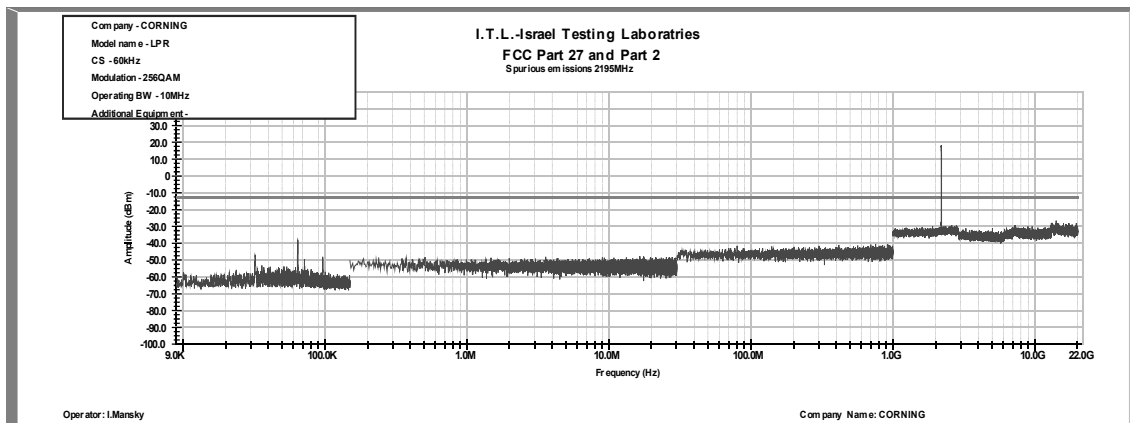
Figure 383: Spurious Emissions at Antenna Terminal 256QAM, 2195.0MHz, B.W. 10MHz, Sub Carrier 60 kHz
