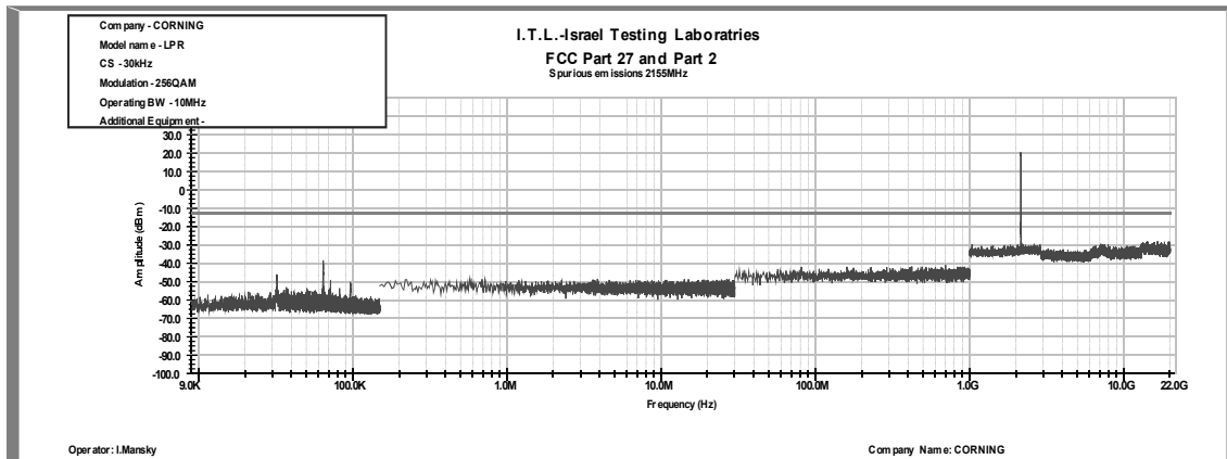
Figure 379: Spurious Emissions at Antenna Terminal 256QAM, 2155.0MHz, B.W. 10MHz, Sub Carrier 30 kHz
