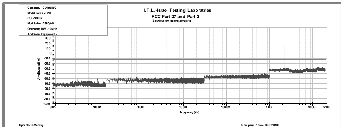
Figure 380: Spurious Emissions at Antenna Terminal 256QAM, 2195.0MHz, B.W. 10MHz, Sub Carrier 30 kHz
