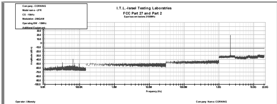
Figure 385: Spurious Emissions at Antenna Terminal 256QAM, 2155.0MHz, B.W. 15MHz, Sub Carrier 15 kHz
