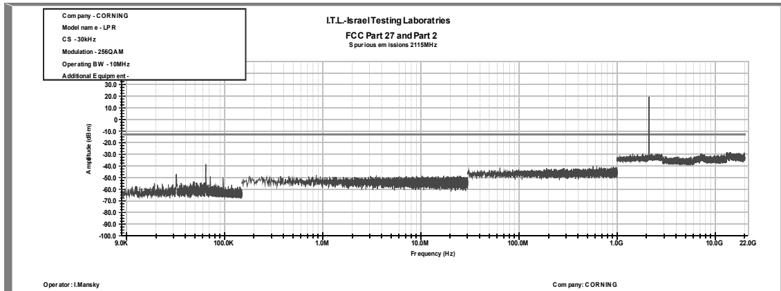
Figure 378: Spurious Emissions at Antenna Terminal 256QAM, 2115.0MHz, B.W. 10MHz, Sub Carrier 30 kHz
