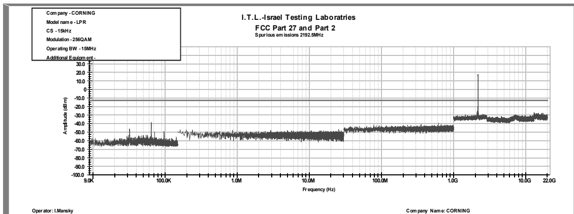
Figure 386: Spurious Emissions at Antenna Terminal 256QAM, 2192.5MHz, B.W. 15MHz, Sub Carrier 15 kHz
