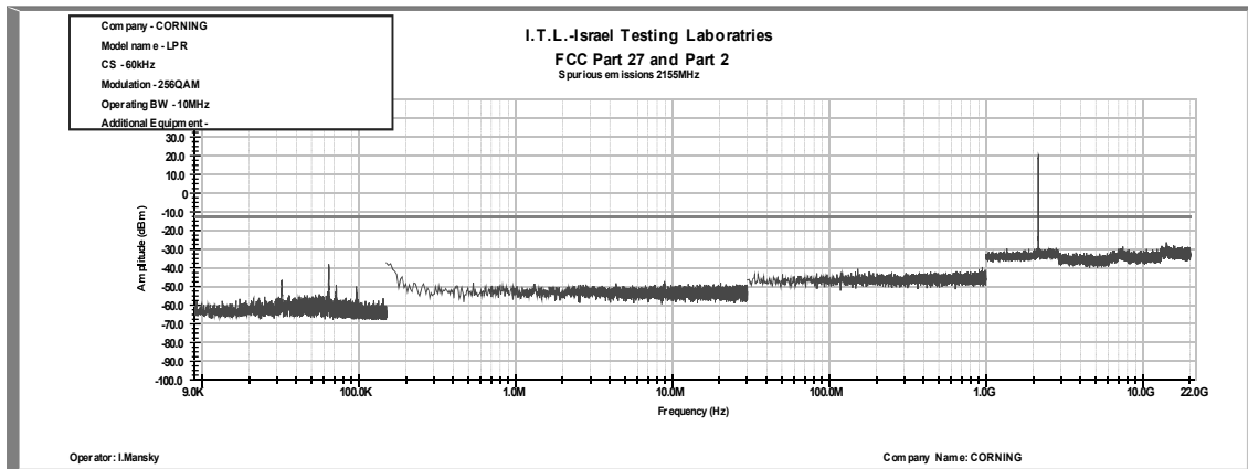
Figure 382: Spurious Emissions at Antenna Terminal 256QAM, 2155.0MHz, B.W. 10MHz, Sub Carrier 60 kHz
