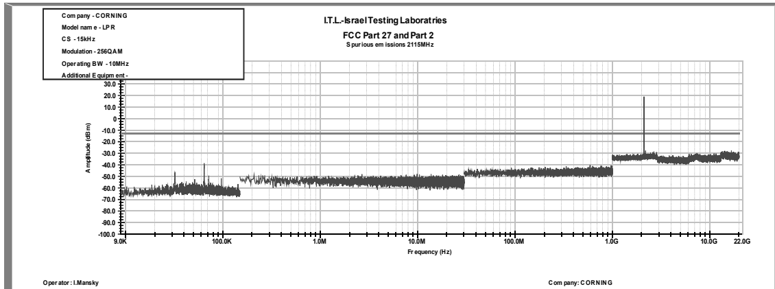
Figure 375: Spurious Emissions at Antenna Terminal 256QAM, 2115.0MHz, B.W. 10MHz, Sub Carrier 15 kHz
