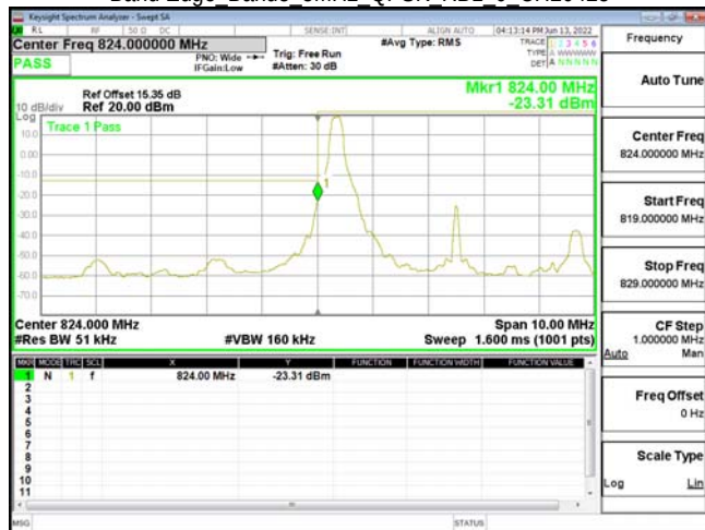
Band Edge Band5 5MHz QPSK RB1 0 CH20425
