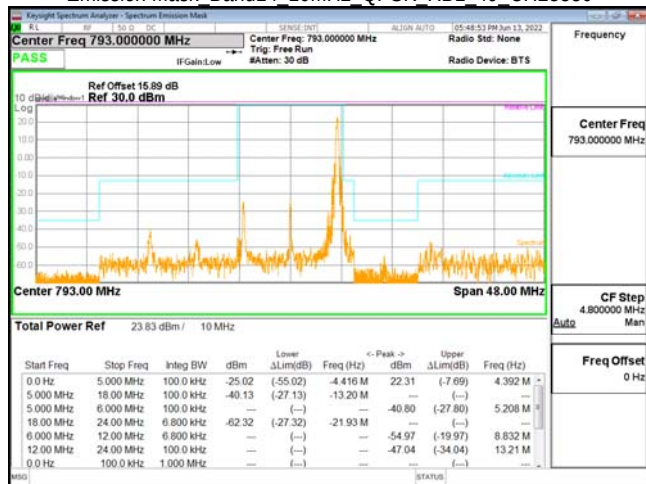
Emission Mask Band14 10MHz QPSK RB50 0 CH23330
