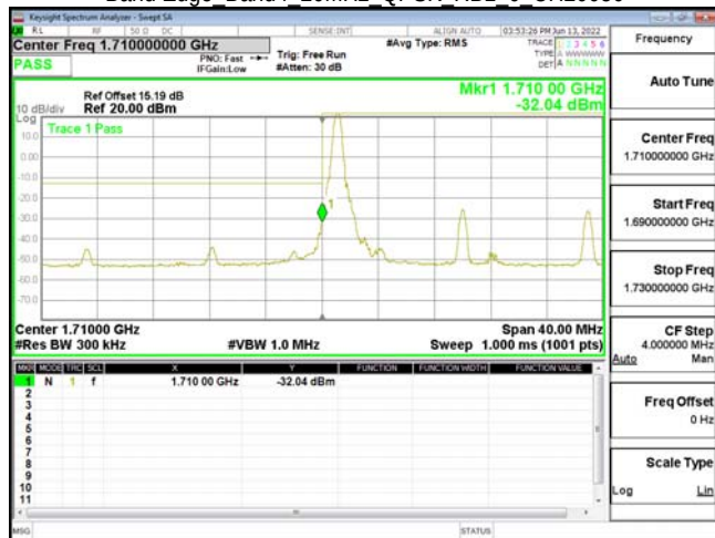
Band Edge Band4 20MHz QPSK RB1 0 CH20050
