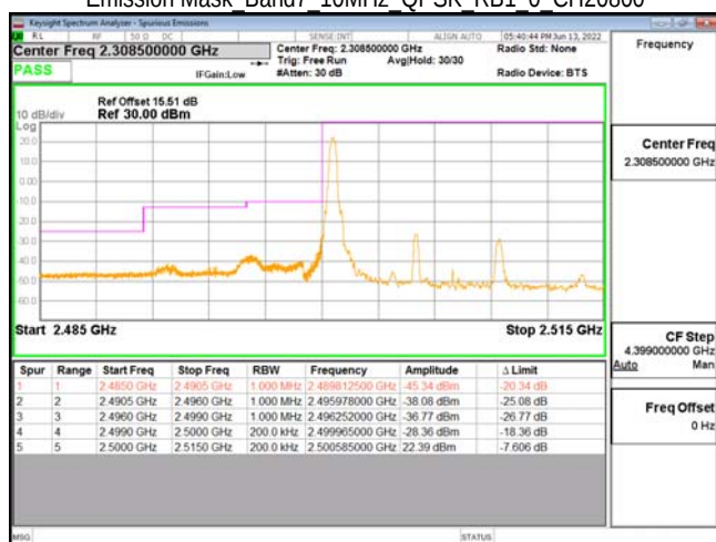
Emission Mask Band7 10MHz QPSK RB1 0 CH20800
