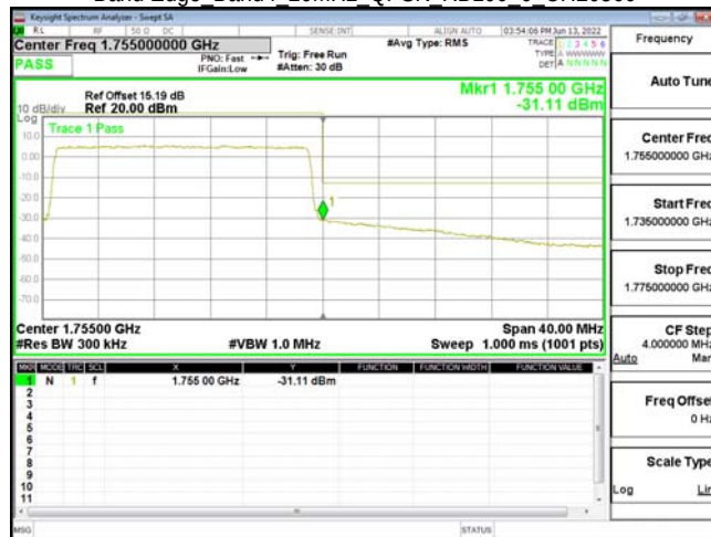
Band Edge Band4 20MHz QPSK RB100 0 CH20300
