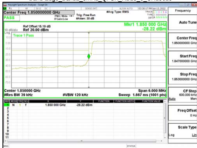
Band Edge Band2 3MHz QPSK RB15 0 CH19185
