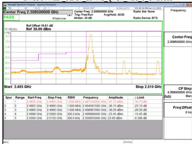
Emission Mask Band7 15MHz QPSK RB1 74 CH21375
