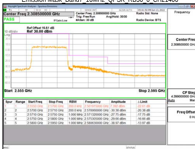
Emission Mask Band7 10MHz QPSK RB50 0 CH21400
