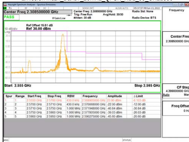
Emission Mask Band7 20MHz QPSK RB1 99 CH21350
