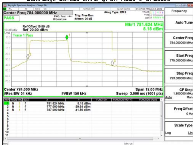
Band Edge Band13 5MHz QPSK RB25 0 CH23205
