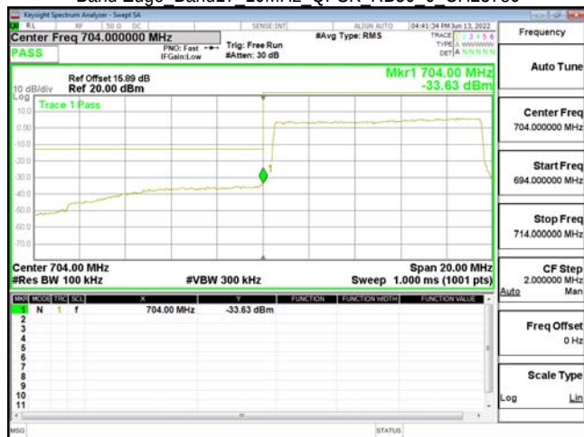
Band Edge Band17 10MHz QPSK RB50 0 CH23780
