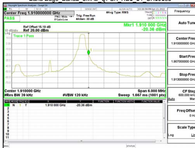
Band Edge Band2 3MHz QPSK RB1 14 CH19185
