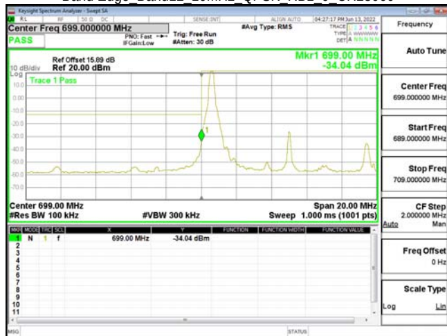
Band Edge Band12 10MHz QPSK RB1 0 CH23060
