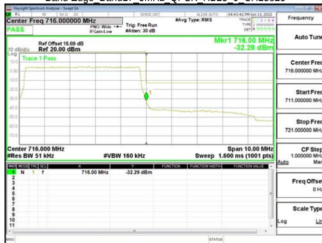
Band Edge Band17 5MHz QPSK RB25 0 CH23825
