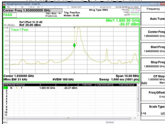
Band Edge Band2 5MHz QPSK RB1 0 CH18625
