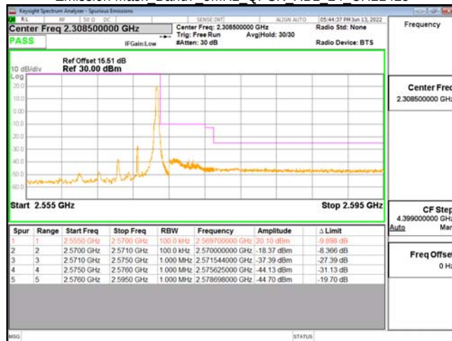
Emission Mask Band7 5MHz QPSK RB1 24 CH21425
