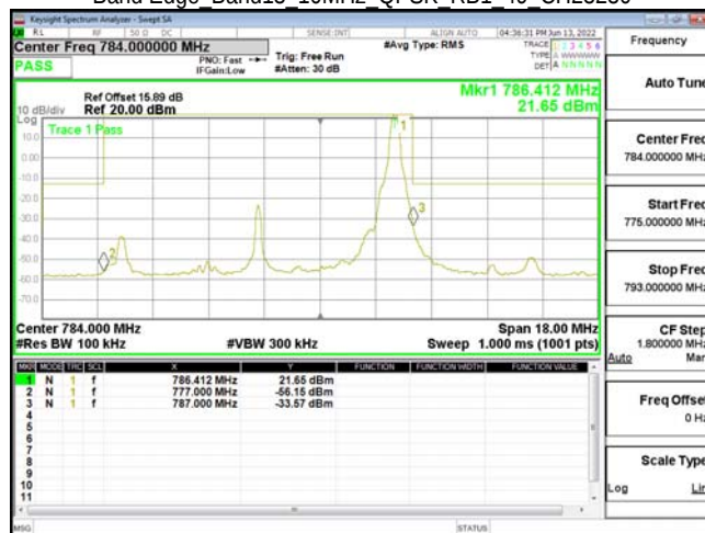
Band Edge Band13 10MHz QPSK RB1 49 CH23230
