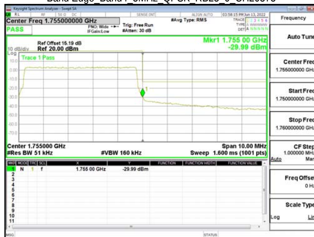
Band Edge Band4 5MHz QPSK RB25 0 CH20375
