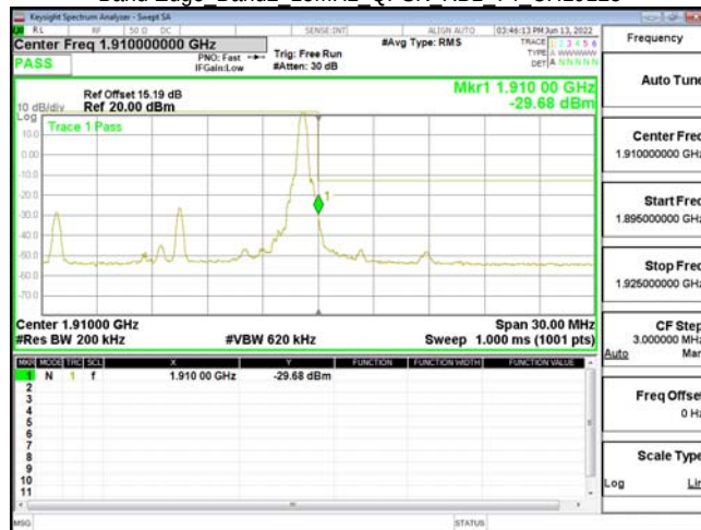
Band Edge Band2 15MHz QPSK RB1 74 CH19125
