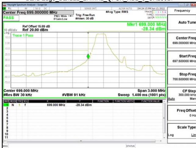
Band Edge Band12 1.4MHz QPSK RB1 0 CH23017
