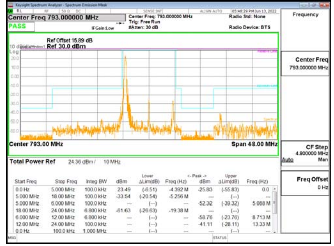
Emission Mask Band14 10MHz QPSK RB1 0 CH23330
