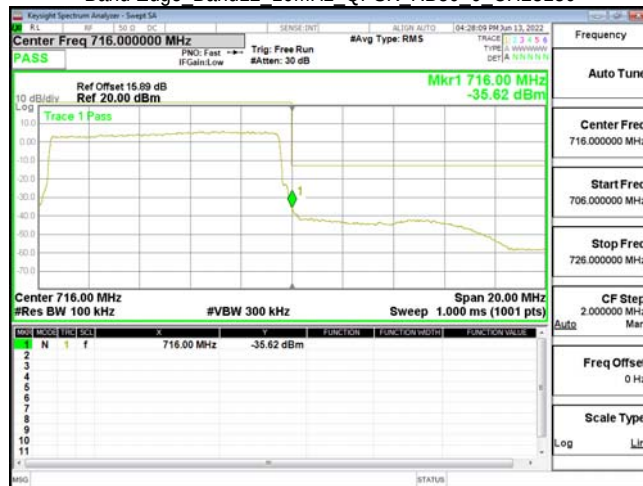
Band Edge Band12 10MHz QPSK RB50 0 CH23130
