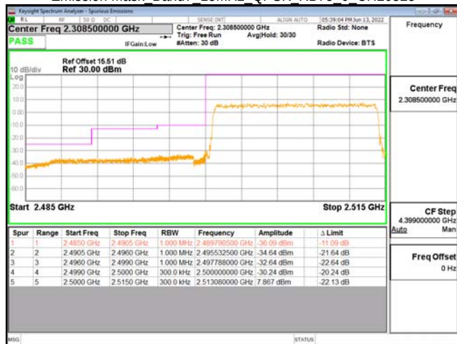
Emission Mask Band7 15MHz QPSK RB75 0 CH20825
