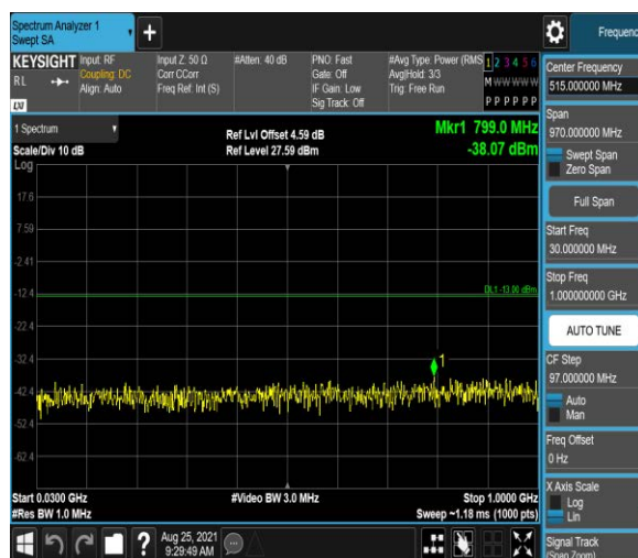
Band4-20MHz-16QAM-20300:30~1000MHz
