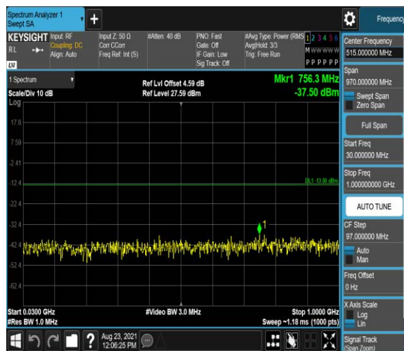
Band2-20MHz-16QAM-19100:30~1000MHz
