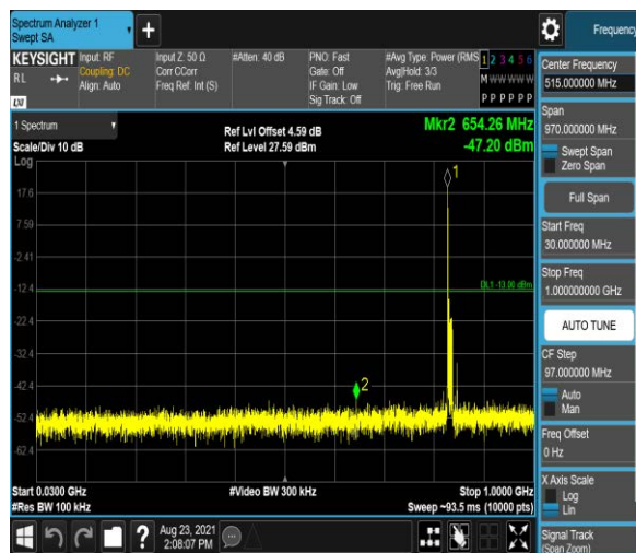
Band5-10MHz-16QAM-20600:30~1000MHz
