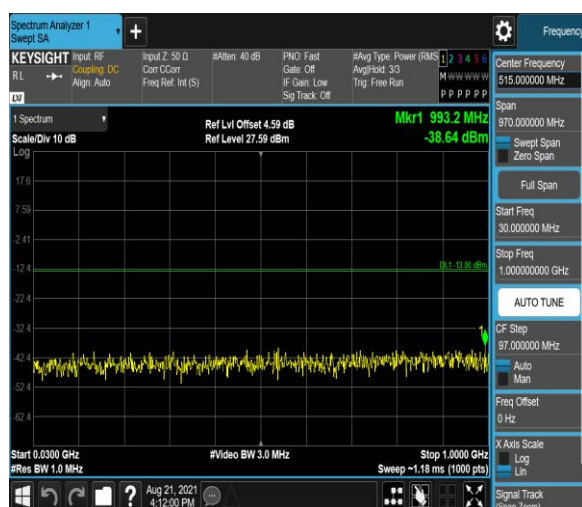
Band2-1.4MHz-16QAM-19193:30~1000MHz
