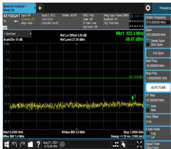
Band2-1.4MHz-16QAM-18900:30~1000MHz
