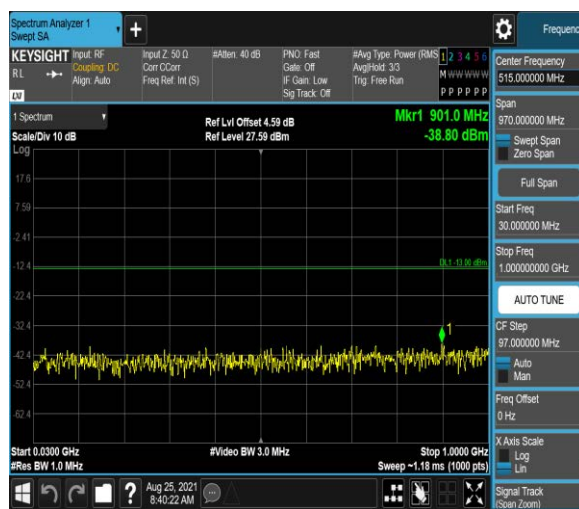
Band4-1.4MHz-16QAM-20175:30~1000MHz
