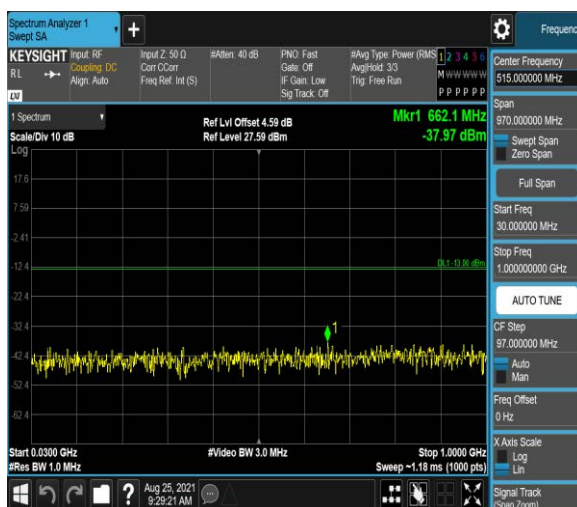
Band4-20MHz-QPSK-20300:30~1000MHz
