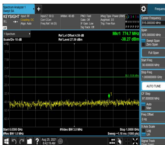
Band4-1.4MHz-16QAM-20393:30~1000MHz
