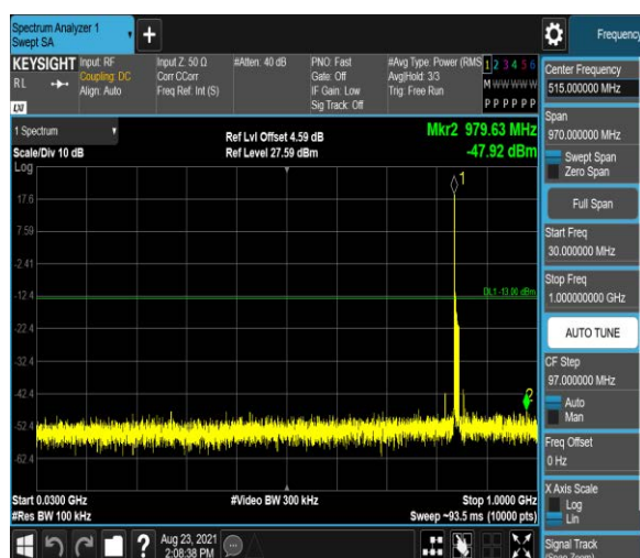
Band5-10MHz-QPSK-20600:30~1000MHz
