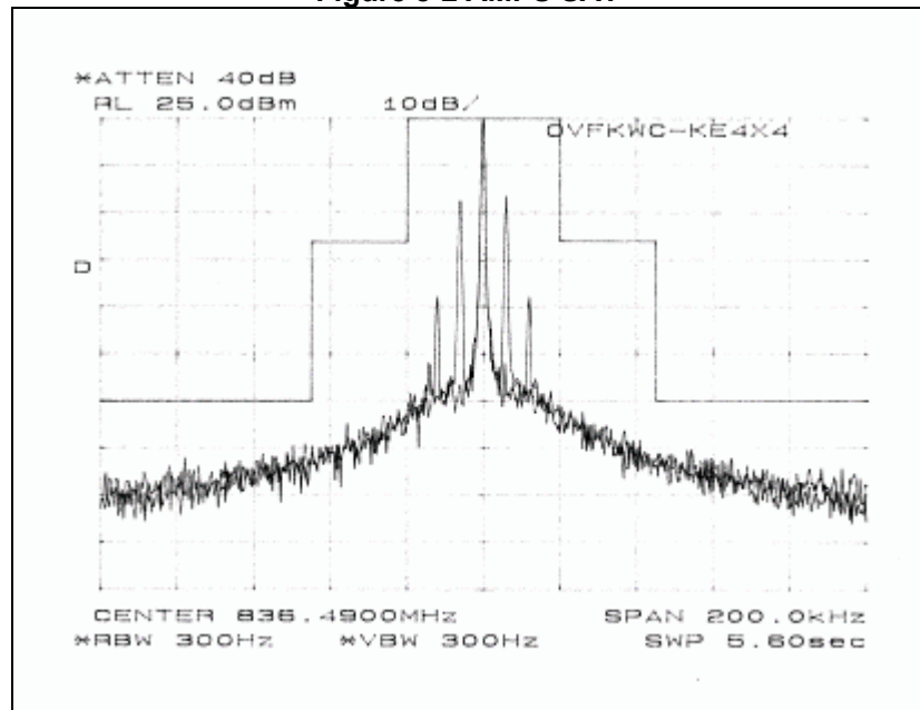
Figure 8-2 AMPS SAT
