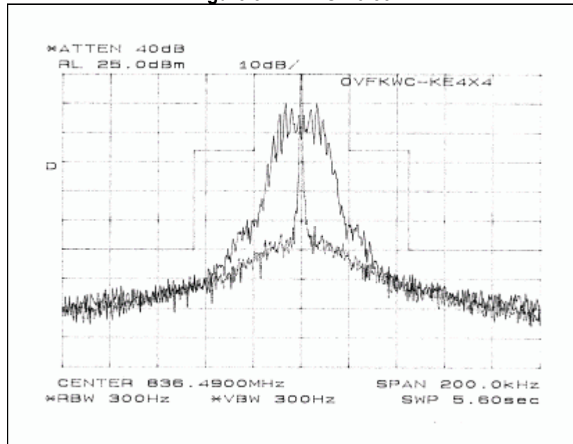
Figure 8-1 AMPS Voice
