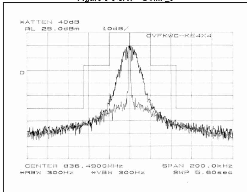
Figure 8-6 SAT + DTMF_9
