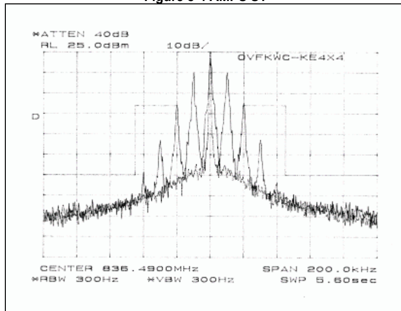
Figure 8-4 AMPS ST
