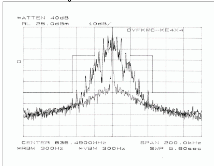
Figure 8-7 AMPS WIDEBAND
