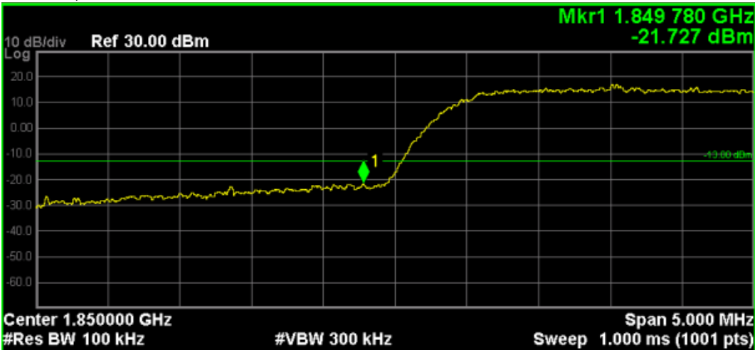
WCDMA Band II, Channel 9262
