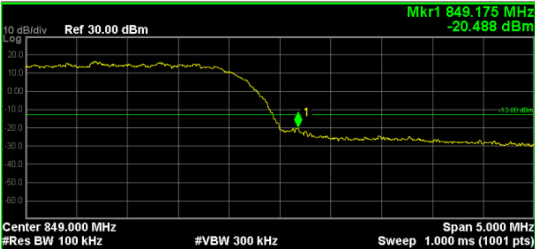
WCDMA Band V, Channel 4233
