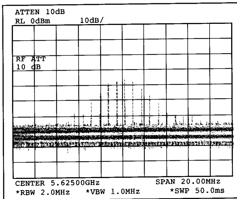
Figure 18. RFI/EMI Detection Data - Front Cabinet Vertical Linear
