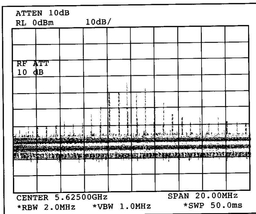
Figure 17. RFI/EMI Detection Data - Front Cabinet Horizontal Linear
