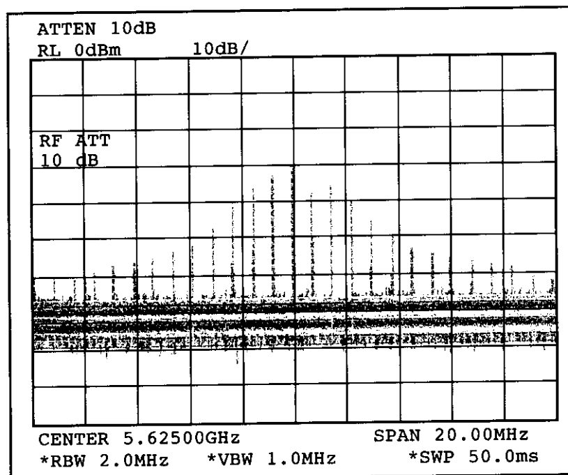
Figure 19. RFI/EMI Detection Data - Back Cabinet Horizontal Linear
