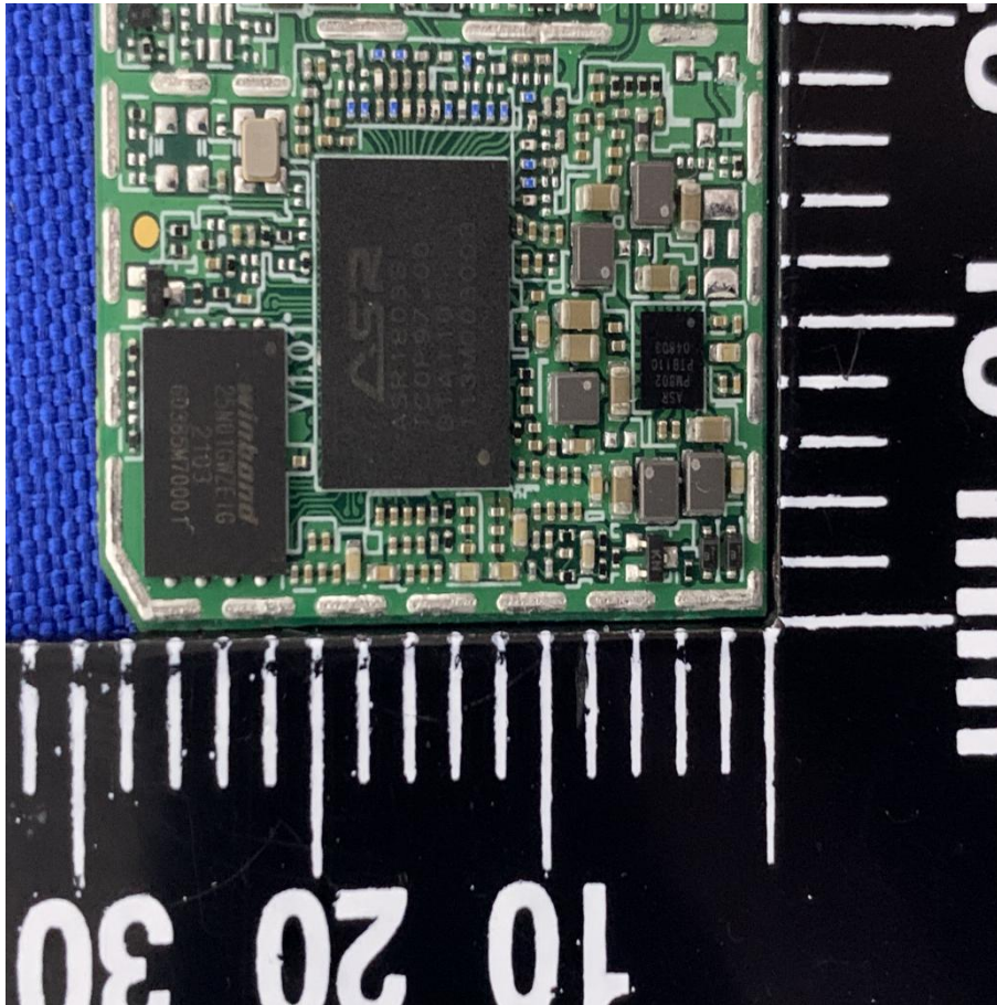
MAIN BOARD TOP VIEW
