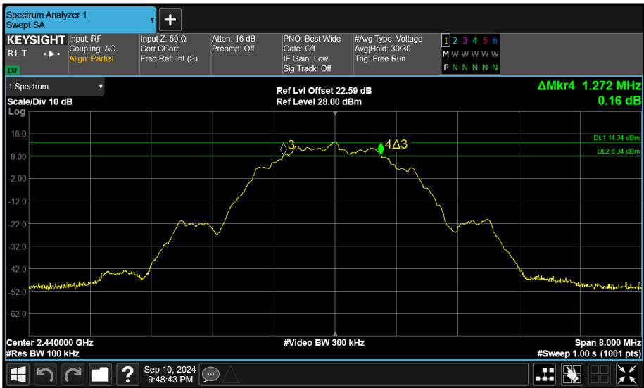
Figure 227 - Core 1 (B) 2440 MHz (CH17) 6 dB Bandwidth
