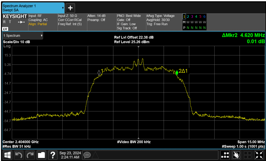
Figure 198 - Core 1 (B) 2404 MHz (CH2) 99% Bandwidth
