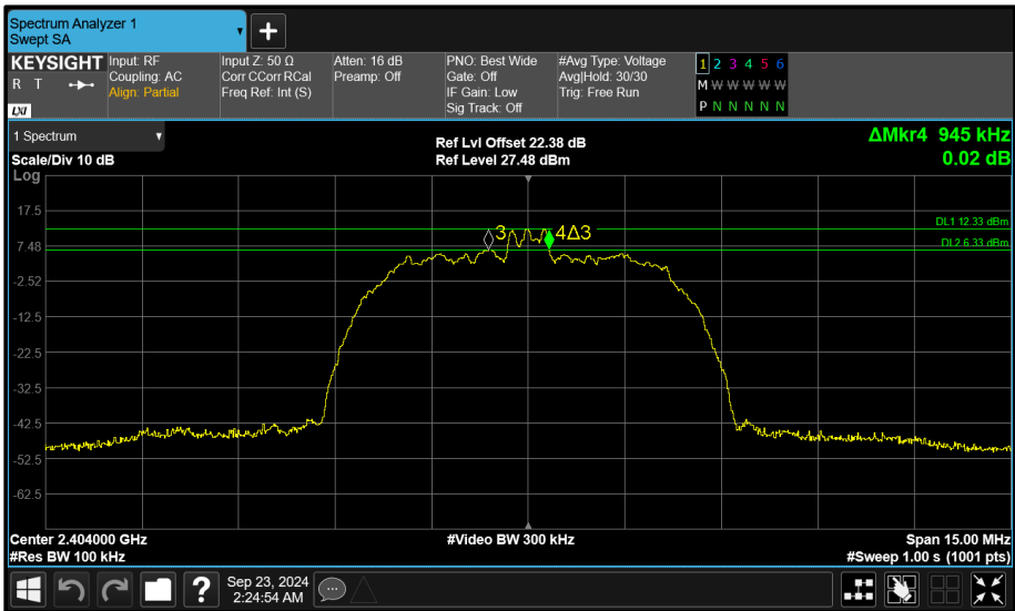
Figure 199 - Core 1 (B) 2404 MHz (CH2) 6 dB Bandwidth
