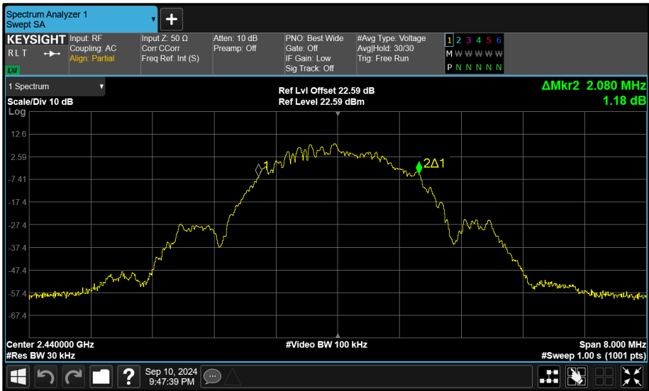
Figure 226 - Core 1 (B) 2440 MHz (CH17) 99% Bandwidth
