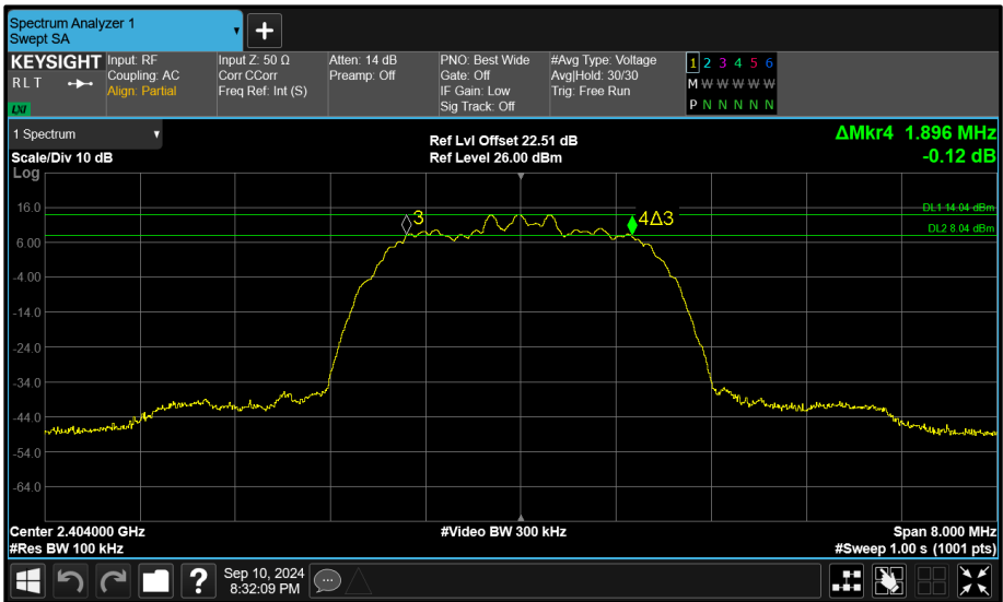
Figure 187 - Core 1 (B) 2404 MHz (CH2) 6 dB Bandwidth
