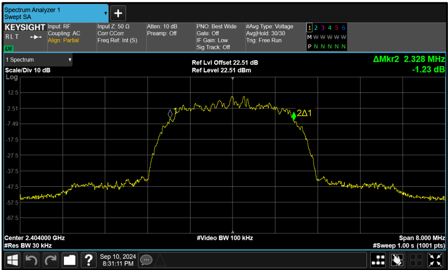
Figure 186 - Core 1 (B) 2404 MHz (CH2) 99% Bandwidth
