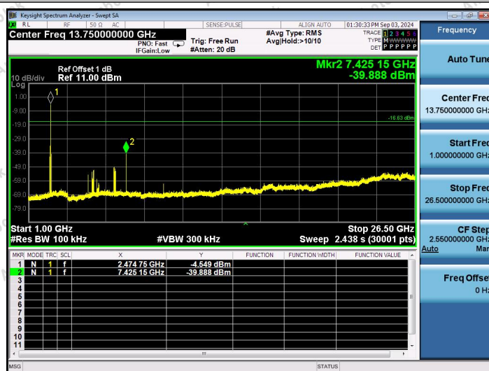
2.4G-Ant1-2475-1000~26500-PASS
