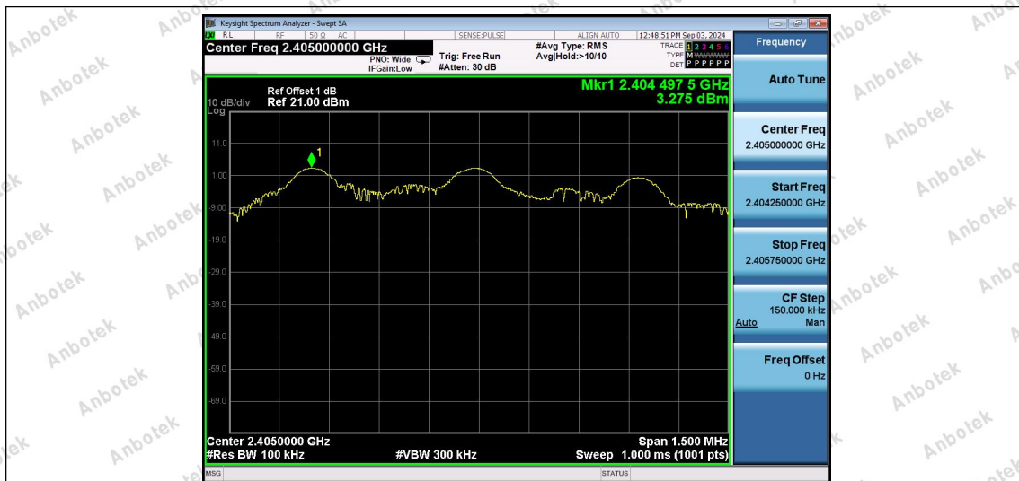
2.4G-Ant1-2405-0~Reference-PASS
