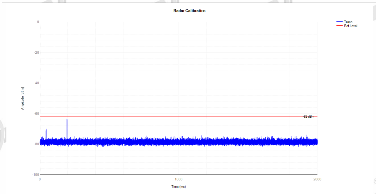
5510MHz DFS_FCC_T6001
