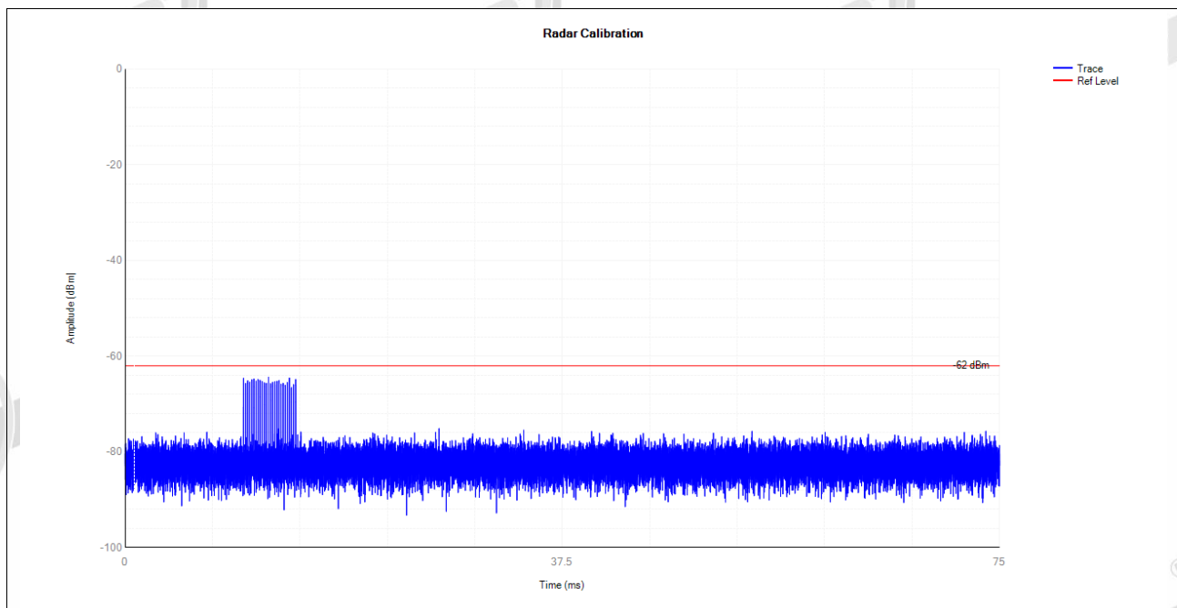
5570MHz DFS_FCC_T3000
