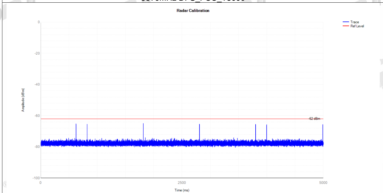
5570MHz DFS_FCC_T6000
