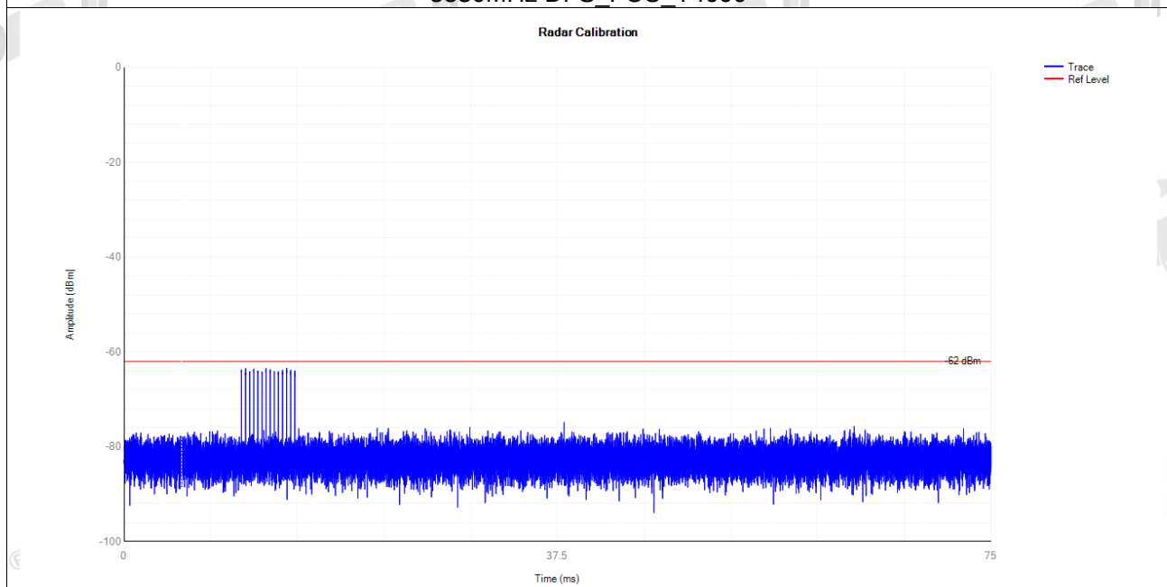
5530MHz DFS_FCC_T5000
