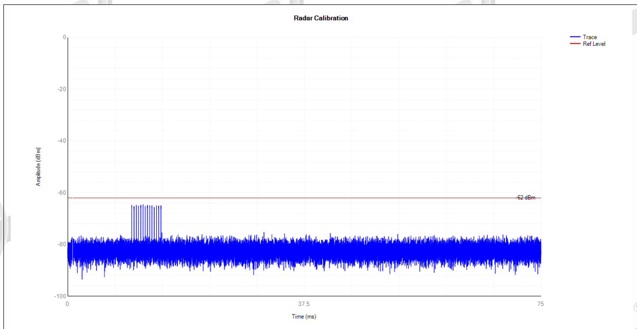
5570MHz DFS_FCC_T5000
