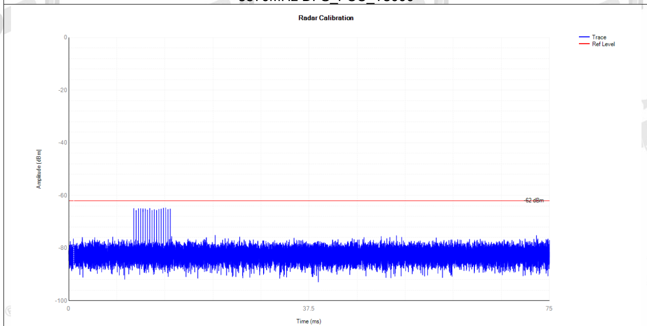
5570MHz DFS_FCC_T4000
