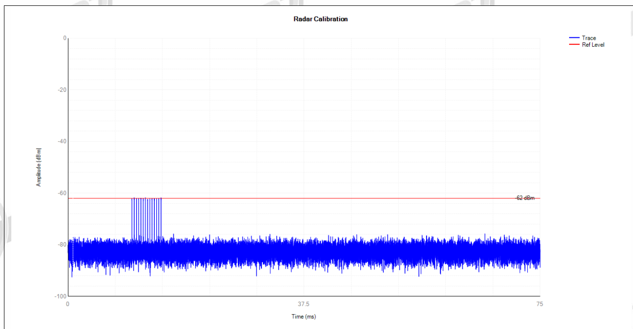
5510MHz DFS_FCC_T5000
