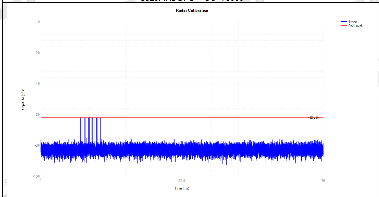
5510MHz DFS_FCC_T4000
