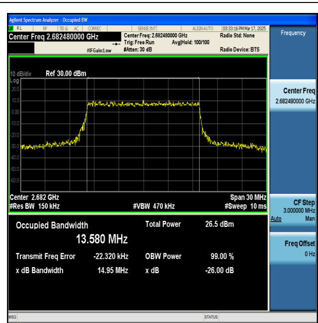
NTNV-n41-PC2-30-15-H-CP-256QAM-Outer_Full-Ant1- PASS
