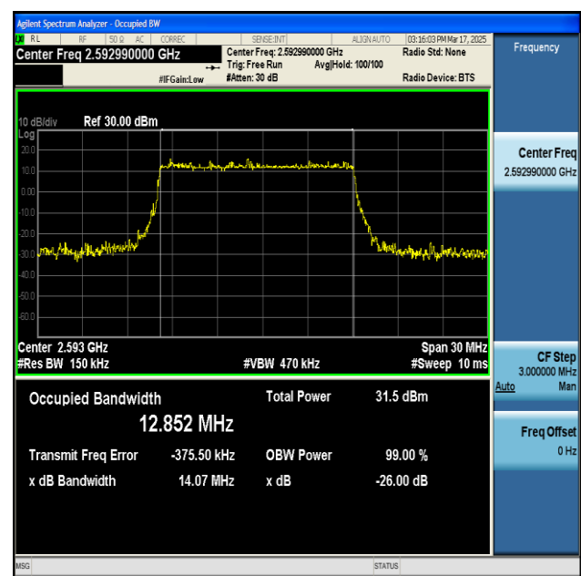
NTNV-n41-PC2-30-15-M-DFT-64QAM-Outer_Full-Ant1- PASS
