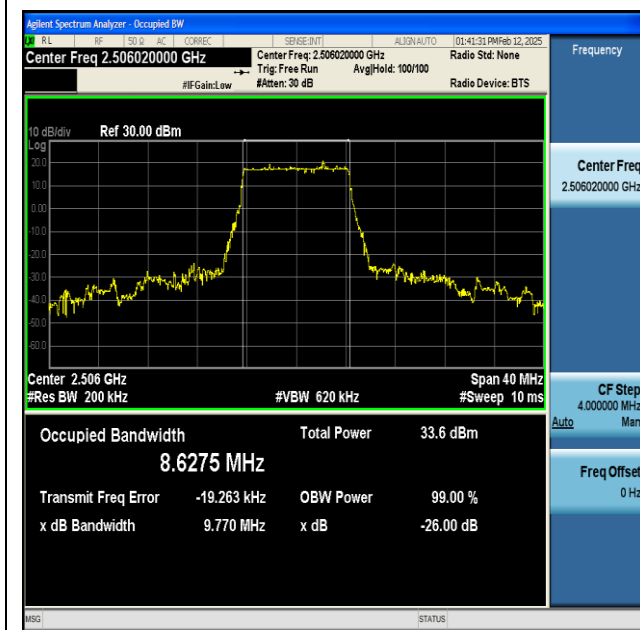
NTNV-n41-PC2-30-20-L-DFT-BPSK-Outer_Full-Ant1- PASS
