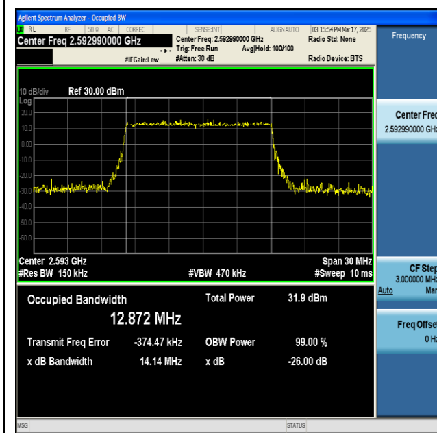
NTNV-n41-PC2-30-15-M-DFT-16QAM-Outer_Full-Ant1- PASS
