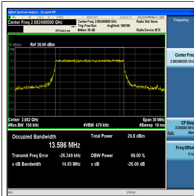
NTNV-n41-PC2-30-15-H-CP-64QAM-Outer_Full-Ant1- PASS
