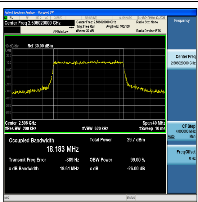
NTNV-n41-PC2-30-20-L-CP-64QAM-Outer_Full-Ant1- PASS
