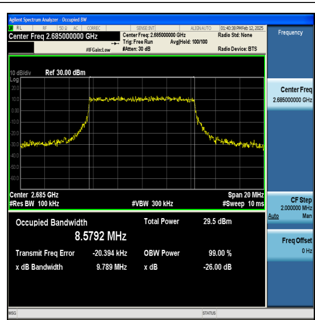
NTNV-n41-PC2-30-10-H-CP-64QAM-Outer_Full-Ant1- PASS
