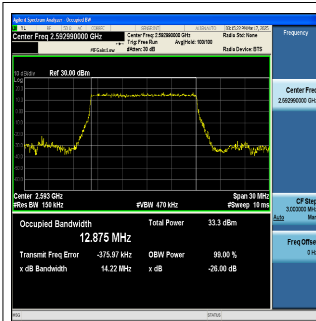
NTNV-n41-PC2-30-15-M-DFT-BPSK-Outer_Full-Ant1- PASS
