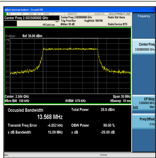
NTNV-n41-PC2-30-15-L-CP-16QAM-Outer_Full-Ant1-PASS
