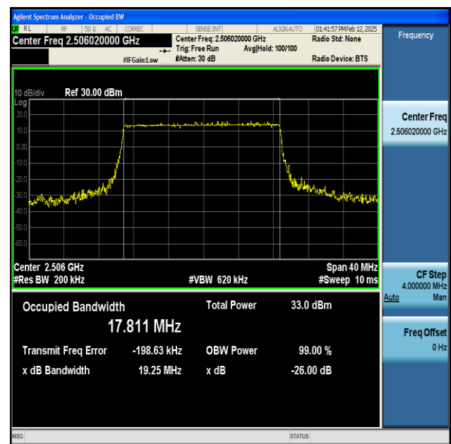
NTNV-n41-PC2-30-20-L-DFT-QPSK-Outer_Full-Ant1- PASS
