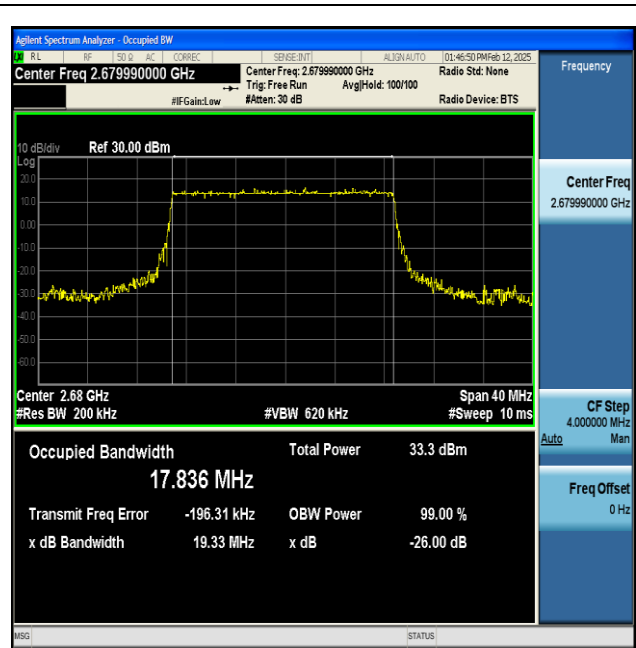
NTNV-n41-PC2-30-20-H-DFT-QPSK-Outer_Full-Ant1- PASS
