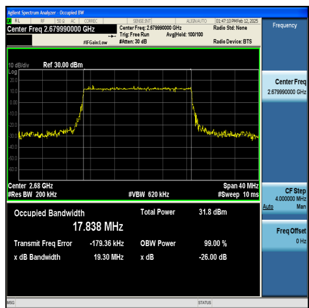
NTNV-n41-PC2-30-20-H-DFT-64QAM-Outer_Full-Ant1- PASS
