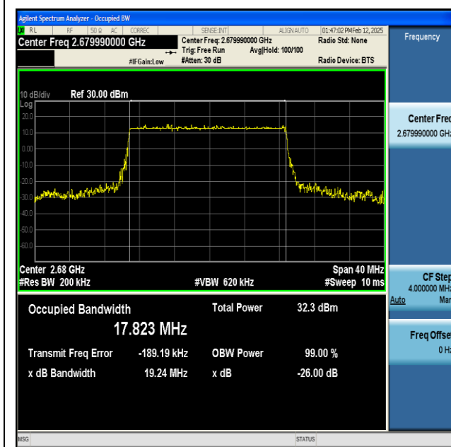
NTNV-n41-PC2-30-20-H-DFT-16QAM-Outer_Full-Ant1- PASS
