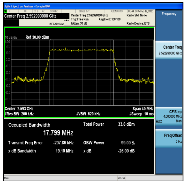
NTNV-n41-PC2-30-20-M-DFT-BPSK-Outer_Full-Ant1- PASS
