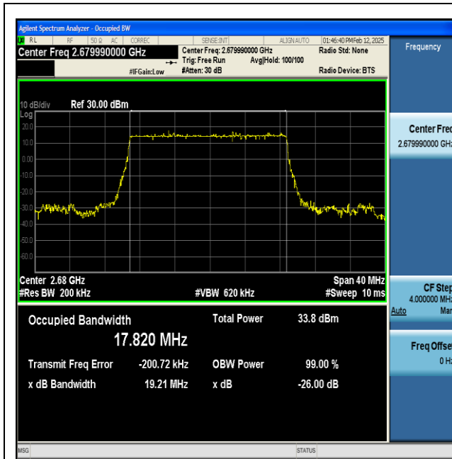
NTNV-n41-PC2-30-20-H-DFT-BPSK-Outer_Full-Ant1- PASS
