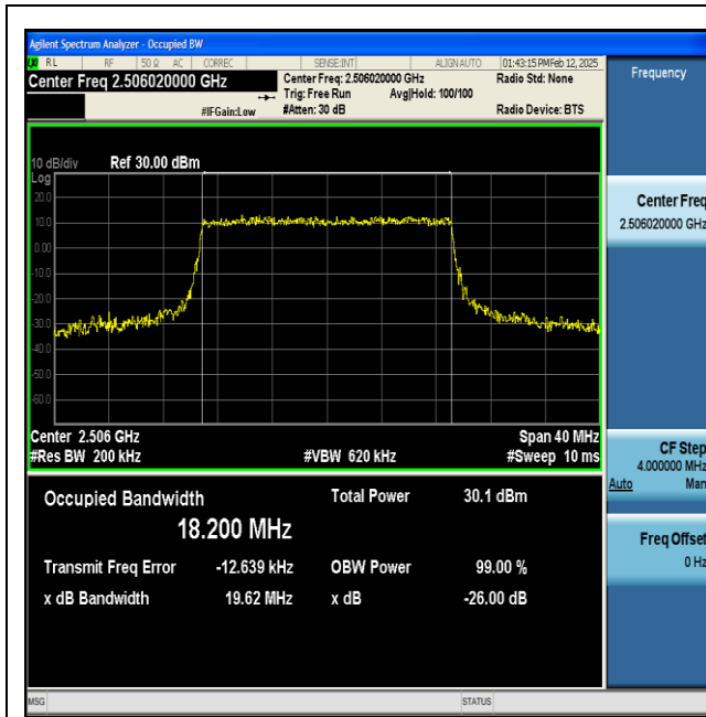
NTNV-n41-PC2-30-20-L-CP-16QAM-Outer_Full-Ant1- PASS
